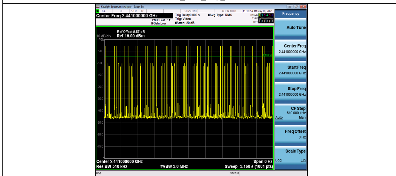
3DH1_Ant1_Hop_2441
