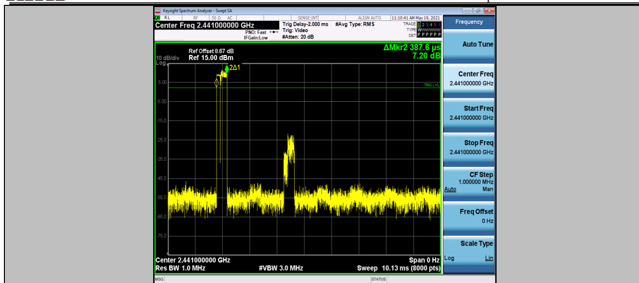
3DH1_Ant1_Hop_2441
