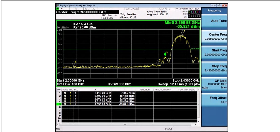
802.11b-Ant1-2412-PASS
