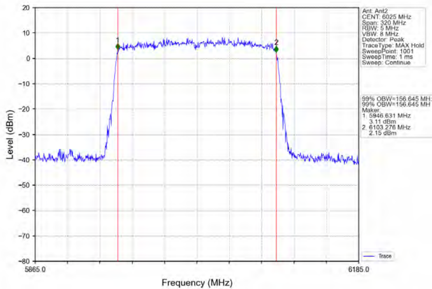
802.11ax(HEW160) LCH 6025MHz 2xRU996 Left Ant2 NTN
