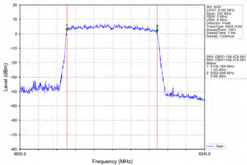
802.11ax(HEW160) MCH_6185MHz_2xRU996 Left Ant2 NTNv
