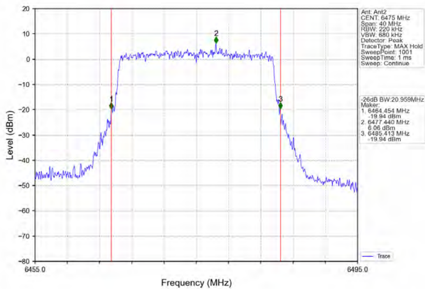
802.11ax(HEW20) MCH 6475MHz RU242 Left Ant2 NTVN
