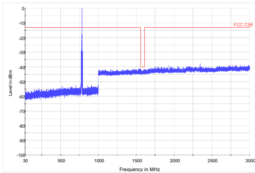
LTE Band 135MHz CH-Low 30MHz~3GHz
