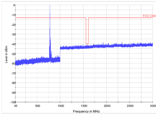
LTE Band 1310MHzCH-High 30MHz~3GHz
