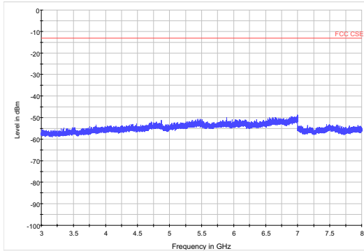
LTE Band 125MHzCH-Low3GHz~8GHz
