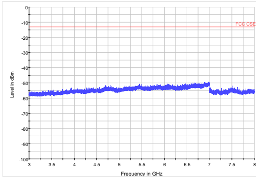
LTE Band 123MHzCH-Middle3GHz~8GHz
