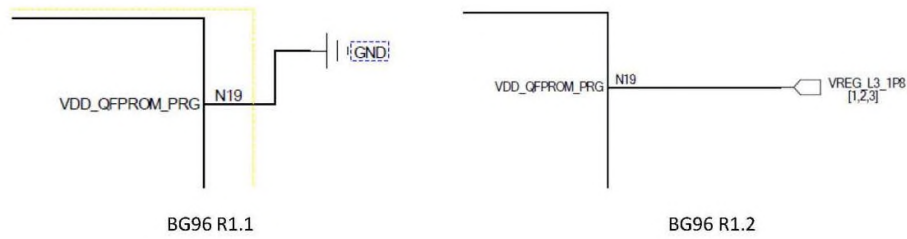
Figure 1: Schematic Designs of BG96 R1.1 and R1.2
