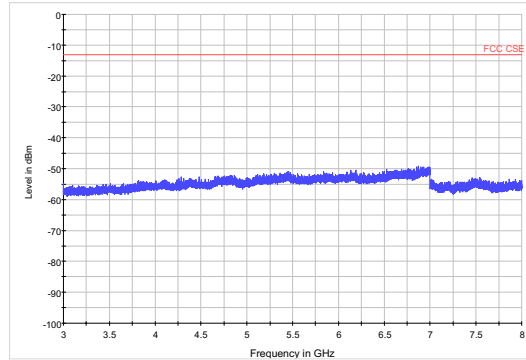
LTE Band 12 3MHz CH-Low3GHz~8GHz
