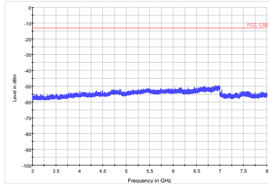
LTE Band 125MHzCH-Middle3GHz~8GHz
