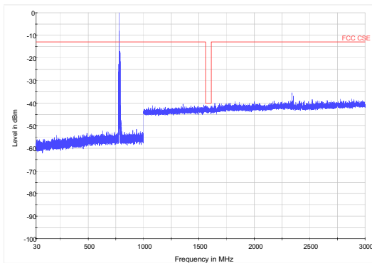
LTE Band 135MHzCH-High 30MHz~3GHz
