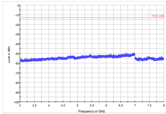
LTE Band 1210MHzCH-Low3GHz~8GHz
