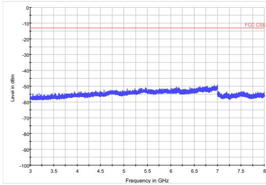
LTE Band 12 1.4MHz CH-Low3GHz~8GHz
