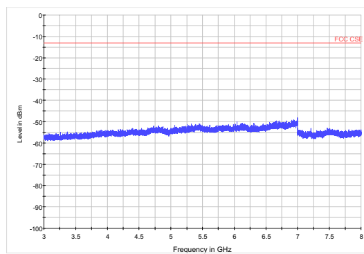
LTE Band 1310MHzCH-High 3GHz~8GHz
