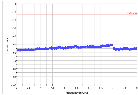
LTE Band 121.4MHzCH-Middle3GHz~8GHz
