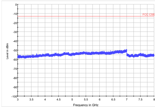
LTE Band 12 1.4MHz CH-High3GHz~8GHz
