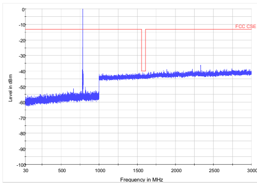
LTE Band 1310MHzCH-High 30MHz~3GHz
