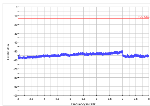
LTE Band 135MHzCH-High3GHz~8GHz
