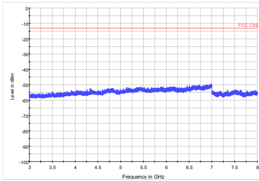
LTE Band 125MHzCH-High3GHz~8GHz
