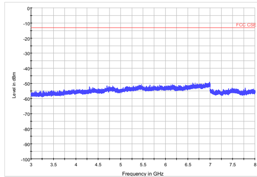
LTE Band 1210MHzCH-High 3GHz~8GHz
