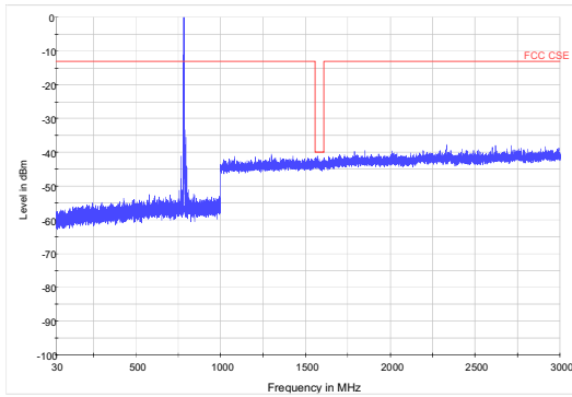
LTE Band 1310MHz CH-Low 30MHz~3GHz
