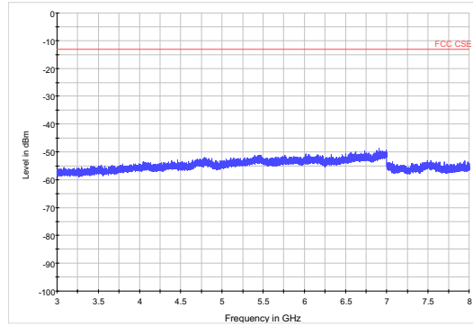
LTE Band 12 3MHz CH-High3GHz~8GHz
