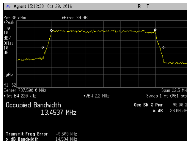
Plot 662. Occupied Bandwidth, QAM-16, Mid Channel, Band 12, Port 1, 15 MHz
