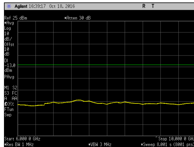
Plot 859. Spurious Emissions at Antenna Terminal, Mid Channel, Band 10, Port 2, 6 GHz – 10 GHz, 15 MHz
