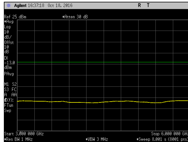
Plot 858. Spurious Emissions at Antenna Terminal, Mid Channel, Band 10, Port 2, 3 GHz – 6 GHz, 15 MHz
