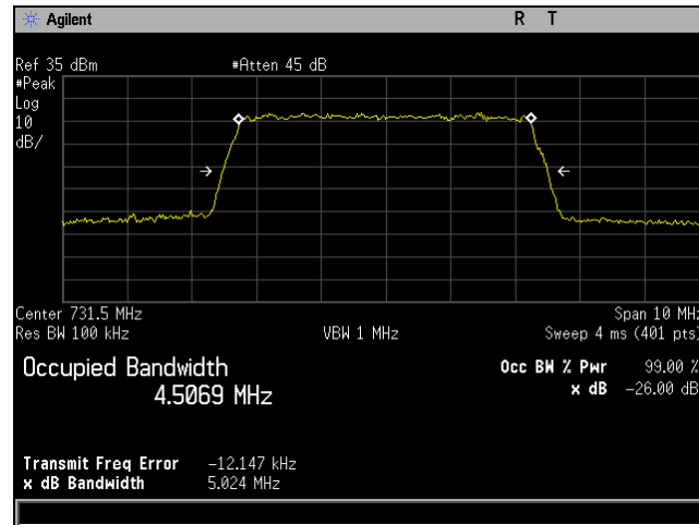
Plot 634. Occupied Bandwidth, QAM-16, Low Channel, Band 12, Port 2, 5 MHz
