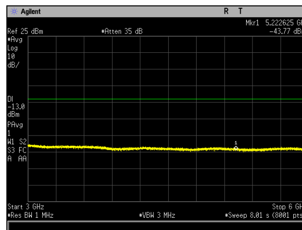
Plot 935. Spurious Emissions at Antenna Terminal, Mid Channel, Band 13, Port 2, 3 GHz – 6 GHz, 5 MHz
