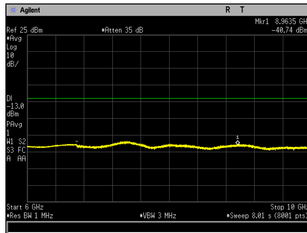
Plot 942. Spurious Emissions at Antenna Terminal, High Channel, Band 13, Port 2, 6 GHz – 10 GHz, 5 MHz
