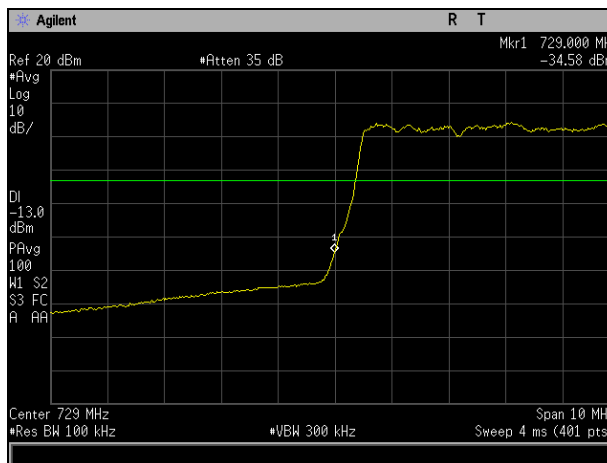
Plot 1113. Conducted Band Edge, QAM-64, Low Channel, Band 12, Port 2, 10 MHz
