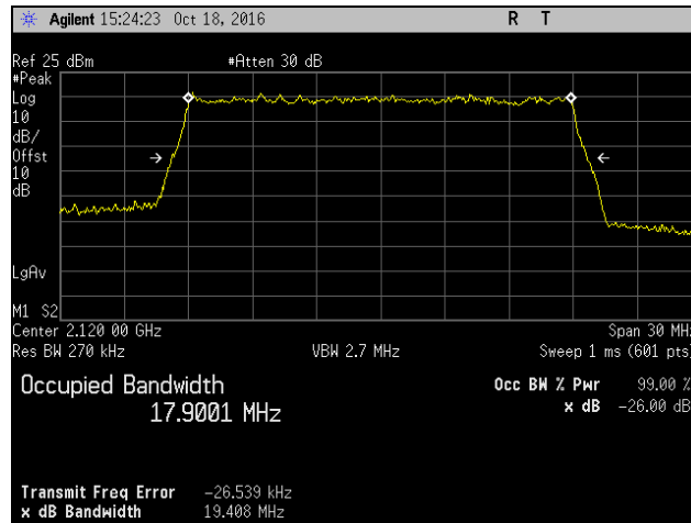
Plot 616. Occupied Bandwidth, -QAM-16, Low Channel, Band 10, Port 2, 20 MHz
