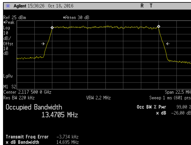
Plot 589. Occupied Bandwidth, QAM-16, Low Channel, Band 10, Port 1, 15 MHz
