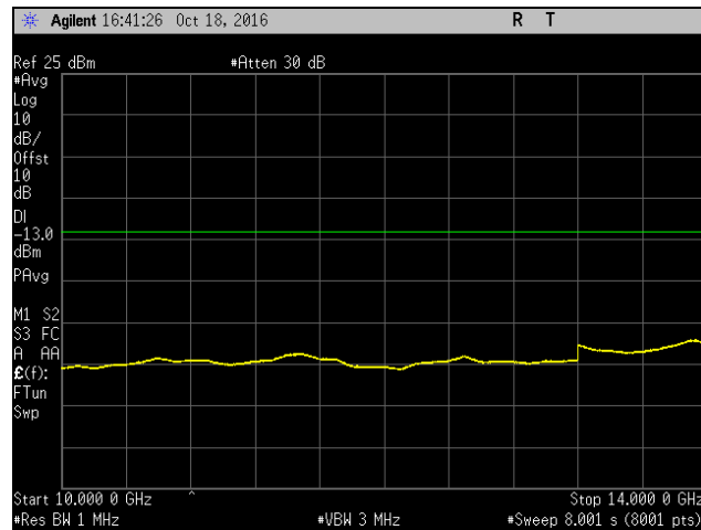
Plot 867. Spurious Emissions at Antenna Terminal, High Channel, Band 10, Port 2, 10 GHz – 14 GHz, 15 MHz
