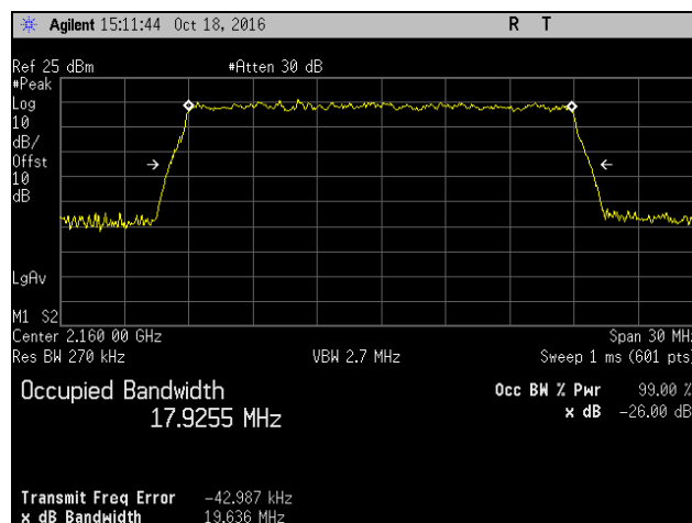
Plot 618. Occupied Bandwidth, QAM-16, High Channel, Band 10, Port 2, 20 MHz
