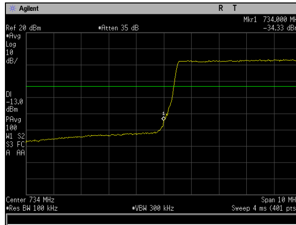
Plot 1165. Conducted Band Edge, QAM-16, Low Channel, Band 17, Port 1, 10 MHz
