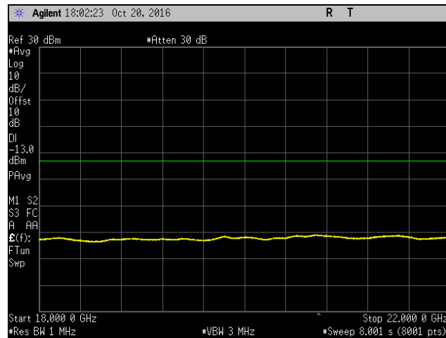
Plot 912. Spurious Emissions at Antenna Terminal, Low Channel, Band 12, Port 2, 18 GHz – 22 GHz, 15 MHz
