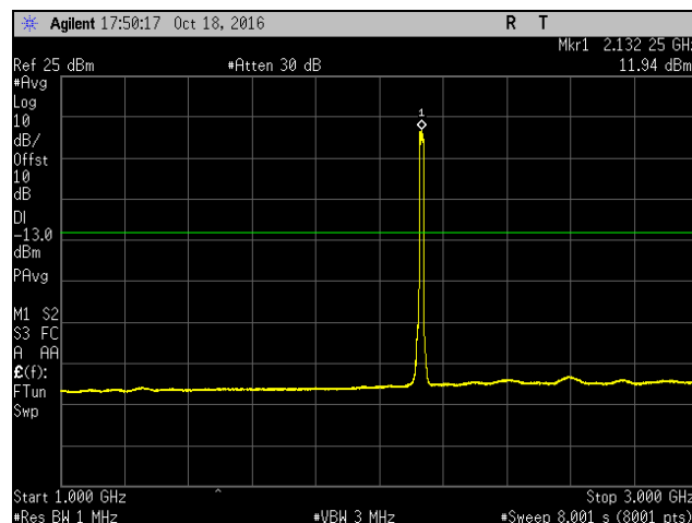
Plot 794. Spurious Emissions at Antenna Terminal, Mid Channel, Band 4, Port 2, 1 GHz – 3 GHz, 15 MHz
