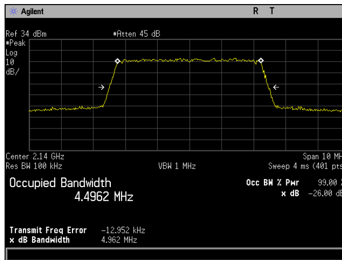
Plot 566. Occupied Bandwidth, QAM-64, Mid Channel, Band 10, Port 2, 5 MHz
