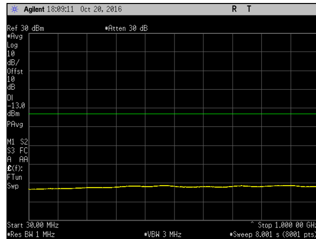
Plot 786. Spurious Emissions at Antenna Terminal, Low Channel, Band 4, Port 2, 30 MHz – 1 GHz, 15 MHz
