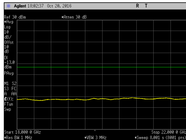
Plot 919. Spurious Emissions at Antenna Terminal, Mid Channel, Band 12, Port 2, 18 GHz – 22 GHz, 15 MHz
