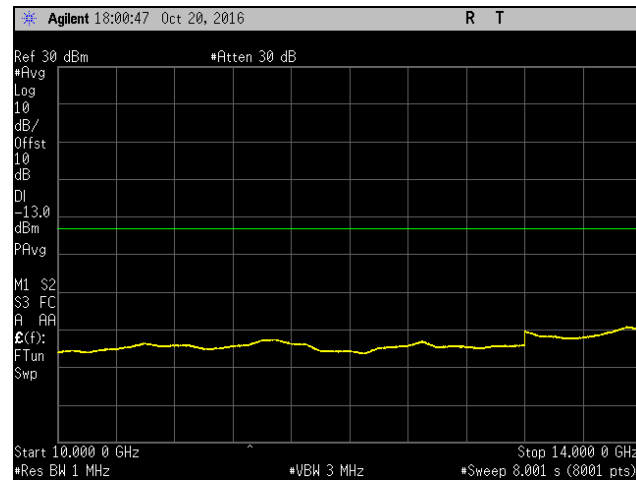
Plot 924. Spurious Emissions at Antenna Terminal, High Channel, Band 12, Port 2, 10 GHz – 14 GHz, 15 MHz
