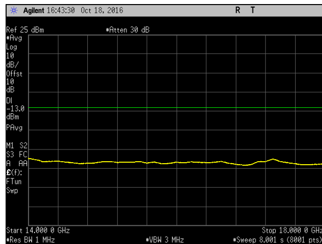
Plot 868. Spurious Emissions at Antenna Terminal, High Channel, Band 10, Port 2, 14 GHz – 18 GHz, 15 MHz
