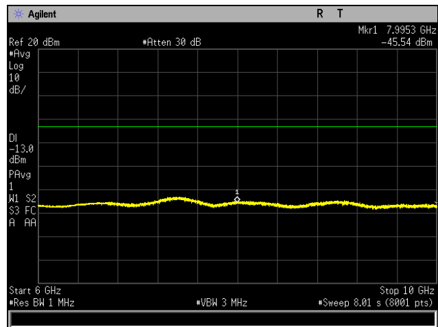
Plot 976. Spurious Emissions at Antenna Terminal, High Channel, Band 17, Port 2, 6 GHz – 10 GHz, 5 MHz
