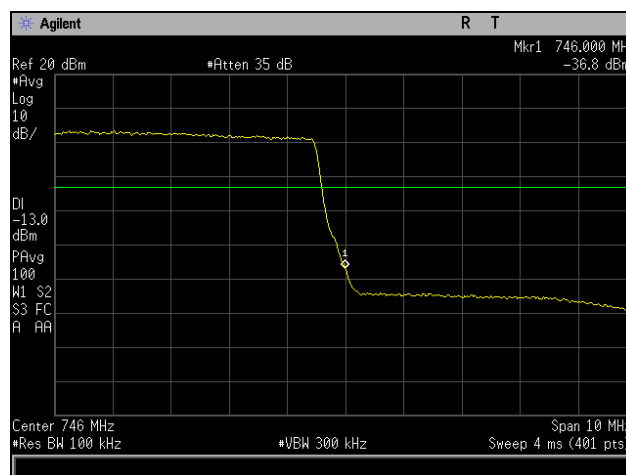
Plot 1116. Conducted Band Edge, QPSK, High Channel, Band 12, Port 2, 10 MHz
