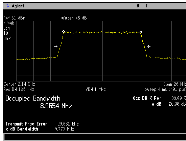
Plot 575. Occupied Bandwidth, QAM-64, Mid Channel, Band 10, Port 1, 10 MHz
