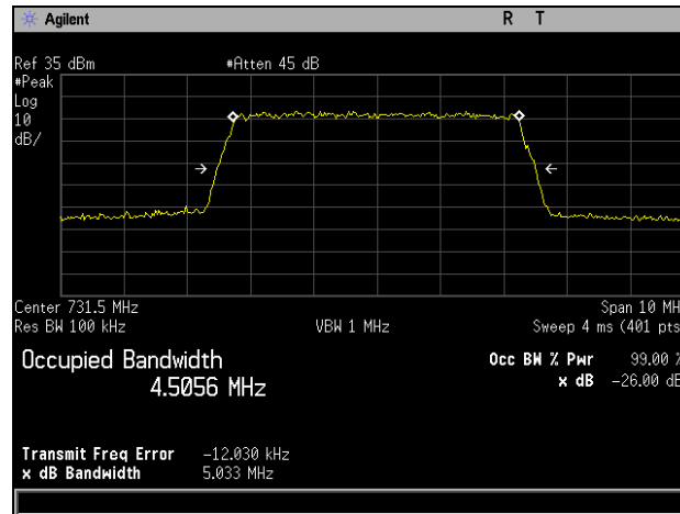
Plot 625. Occupied Bandwidth, QAM-16, Low Channel, Band 12, Port 1, 5 MHz
