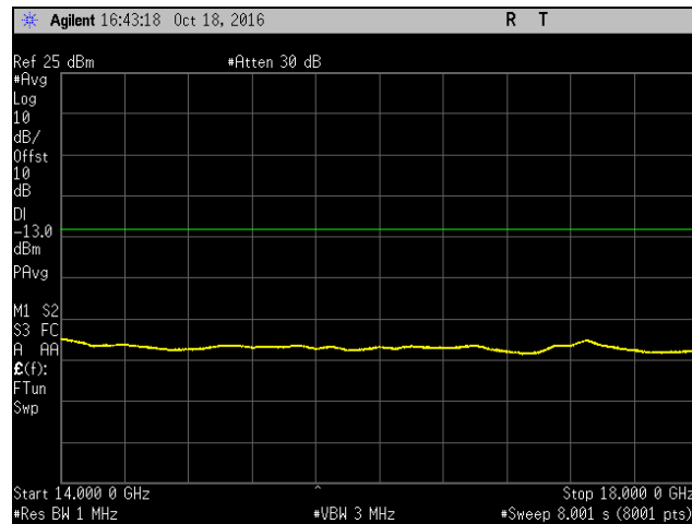
Plot 861. Spurious Emissions at Antenna Terminal, Mid Channel, Band 10, Port 2, 14 GHz – 18 GHz, 15 MHz
