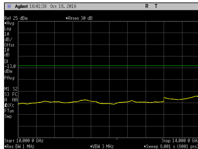
Plot 790. Spurious Emissions at Antenna Terminal, Low Channel, Band 4, Port 2, 10 GHz – 14 GHz, 15 MHz
