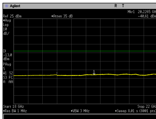
Plot 764. Spurious Emissions at Antenna Terminal, High Channel, Band 4, Port 2, 18 GHz – 22 GHz, 5 MHz
