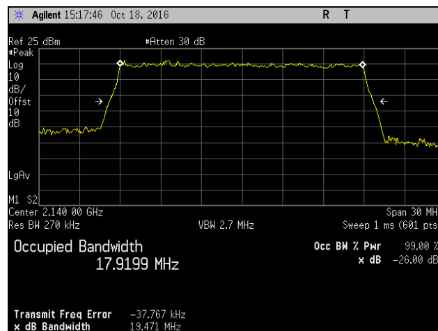
Plot 608. Occupied Bandwidth, QAM-16, Mid Channel, Band 10, Port 1, 20 MHz
