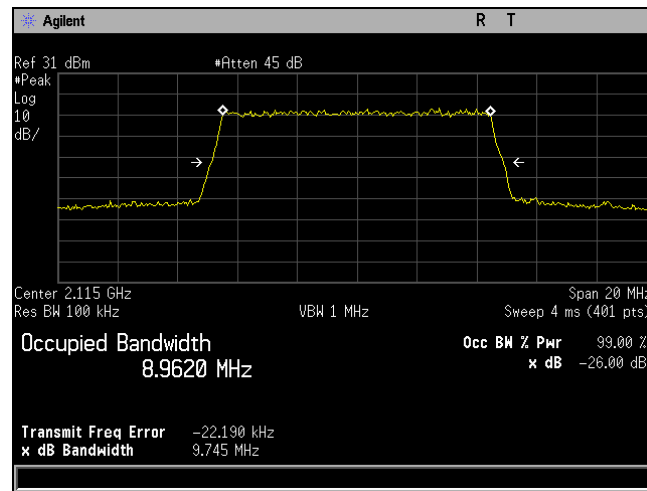
Plot 583. Occupied Bandwidth, QAM-64, Low Channel, Band 10, Port 2, 10 MHz
