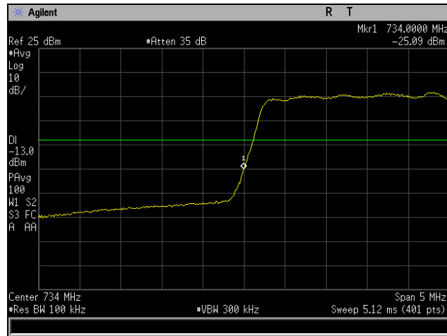
Plot 1159. Conducted Band Edge, QAM-16, Low Channel, Band 17, Port 2, 5 MHz
