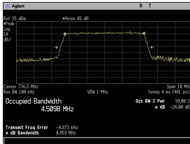
Plot 718. Occupied Bandwidth, QPSK, Low Channel, Band 17, Port 2, 5 MHz
