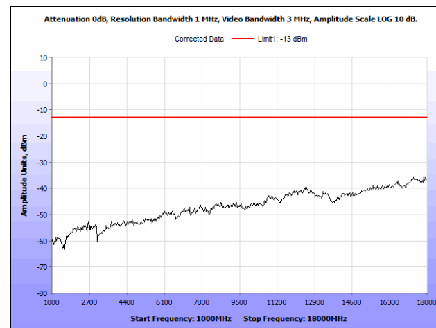
Plot 742. Radiated Spurious Emissions, Band 13, 1 GHz – 18 GHz
