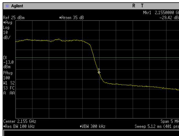
Plot 1004. Conducted Band Edge, QAM-16, High Channel, Band 4, Port 2, 5 MHz
