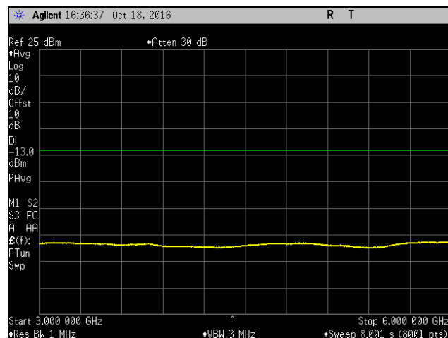
Plot 851. Spurious Emissions at Antenna Terminal, Low Channel, Band 10, Port 2, 3 GHz – 6 GHz, 15 MHz
