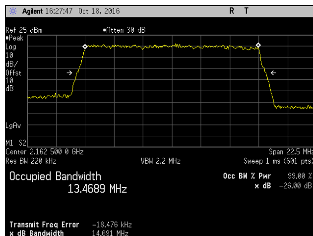
Plot 600. Occupied Bandwidth, QAM-16, High Channel, Band 10, Port 2, 15 MHz
