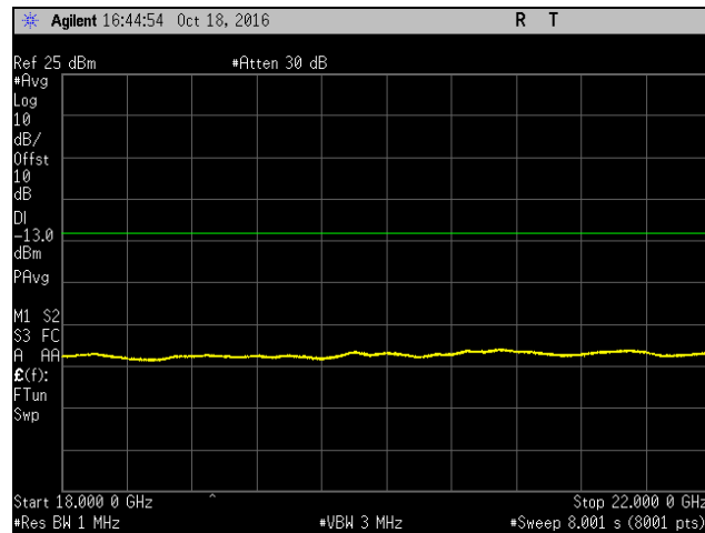
Plot 855. Spurious Emissions at Antenna Terminal, Low Channel, Band 10, Port 2, 18 GHz – 22 GHz, 15 MHz
