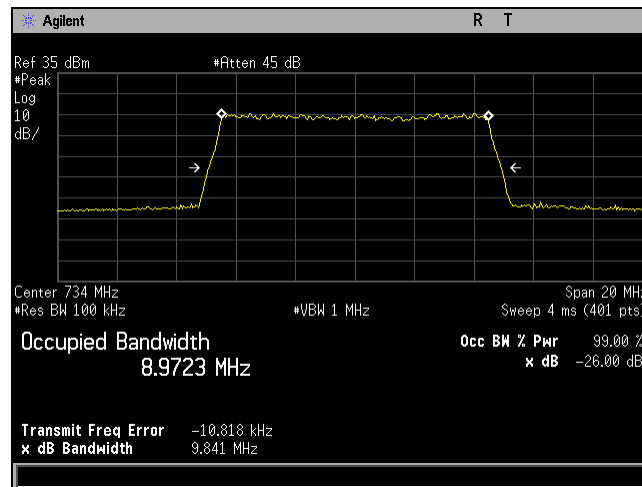
Plot 655. Occupied Bandwidth, QAM-64, Low Channel, Band 12, Port 2, 10 MHz
