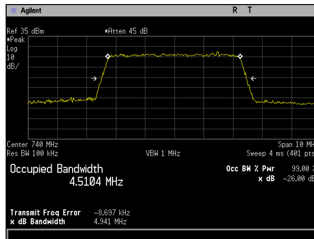
Plot 710. Occupied Bandwidth, QPSK, Mid Channel, Band 17, Port 1, 5 MHz
