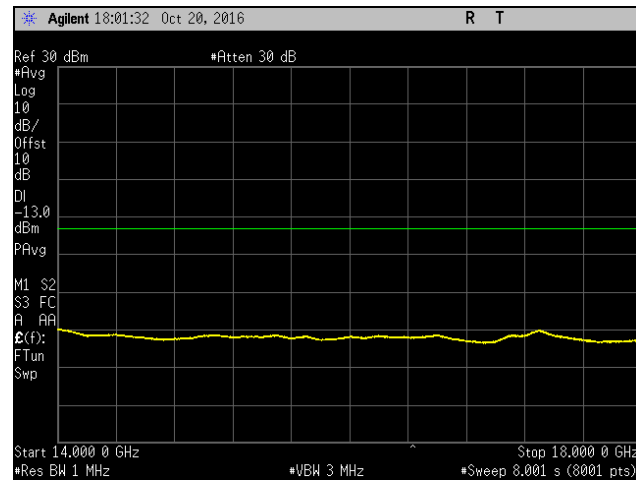
Plot 918. Spurious Emissions at Antenna Terminal, Mid Channel, Band 12, Port 2, 14 GHz – 18 GHz, 15 MHz
