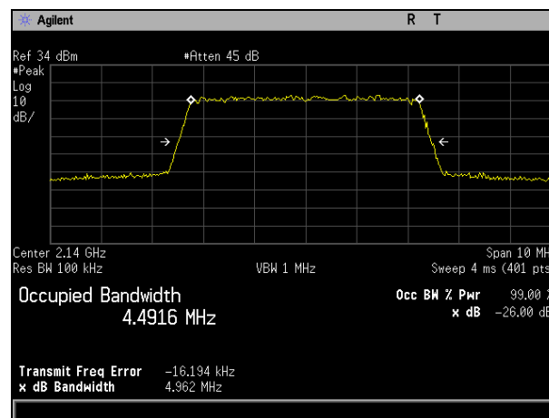
Plot 563. Occupied Bandwidth, QAM-16, Mid Channel, Band 10, Port 2, 5 MHz
