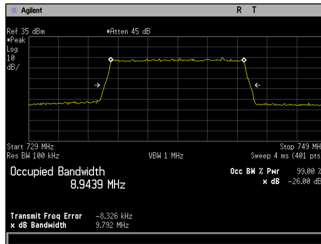
Plot 736. Occupied Bandwidth, QPSK, Low Channel, Band 17, Port 2, 10 MHz
