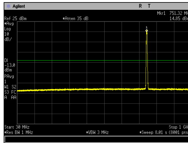
Plot 933. Spurious Emissions at Antenna Terminal, Mid Channel, Band 13, Port 2, 30 MHz – 1 GHz, 5 MHz
