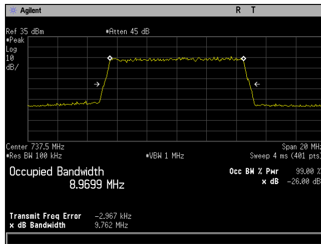
Plot 647. Occupied Bandwidth, QAM-64, Mid Channel, Band 12, Port 1, 10 MHz
