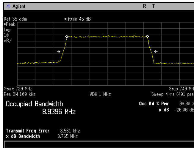
Plot 727. Occupied Bandwidth, QPSK, Low Channel, Band 17, Port 1, 10 MHz
