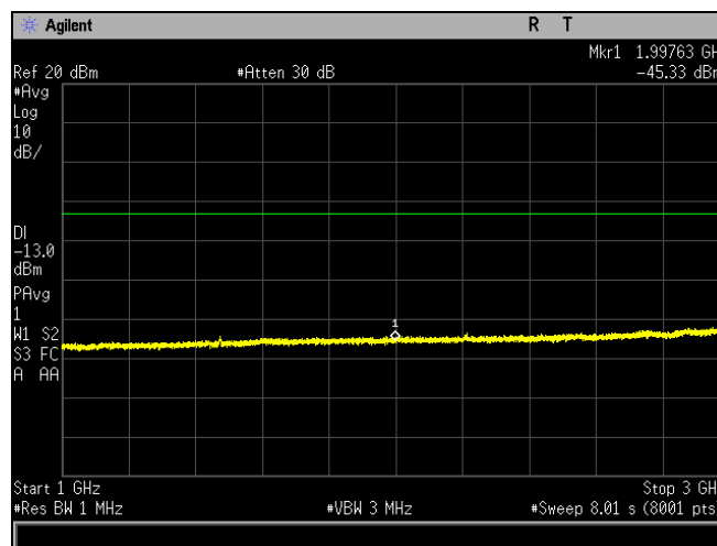
Plot 992. Spurious Emissions at Antenna Terminal, High Channel, Band 17, Port 2, 1 GHz – 3 GHz, 10 MHz
