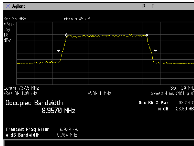
Plot 650. Occupied Bandwidth, QPSK, Mid Channel, Band 12, Port 1, 10 MHz
