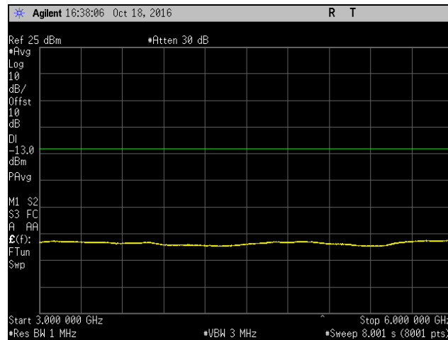
Plot 795. Spurious Emissions at Antenna Terminal, Mid Channel, Band 4, Port 2, 3 GHz – 6 GHz, 15 MHz
