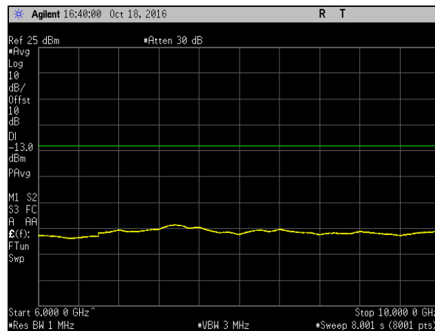
Plot 796. Spurious Emissions at Antenna Terminal, Mid Channel, Band 4, Port 2, 6 GHz – 10 GHz, 15 MHz
