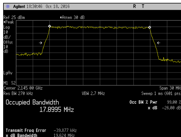
Plot 546. Occupied Bandwidth, QAM-16, High Channel, Band 4, Port 2, 20 MHz
