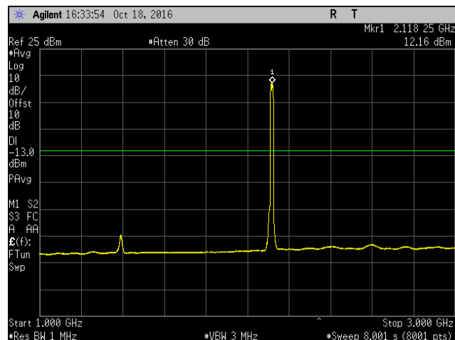
Plot 850. Spurious Emissions at Antenna Terminal, Low Channel, Band 10, Port 2, 1 GHz – 3 GHz, 15 MHz
