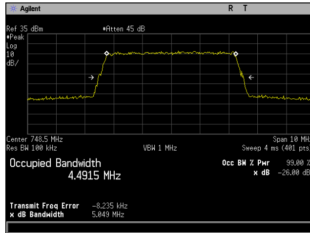
Plot 679. Occupied Bandwidth, QAM-16, Low Channel, Band 13, Port 1, 5 MHz
