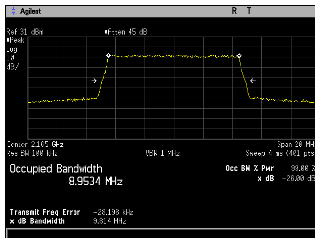
Plot 585. Occupied Bandwidth, QAM-64, High Channel, Band 10, Port 2, 10 MHz
