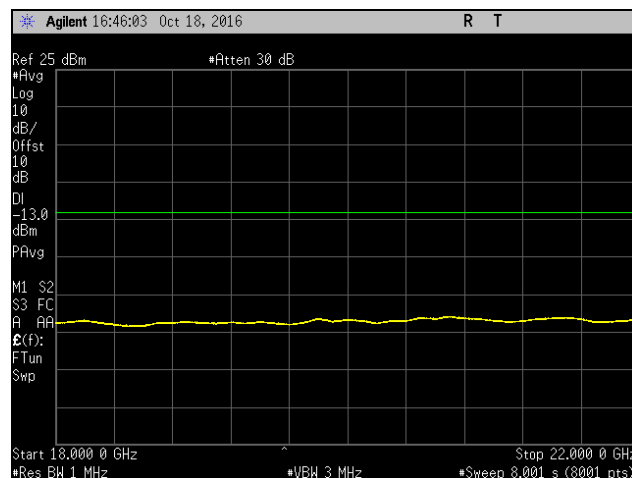
Plot 806. Spurious Emissions at Antenna Terminal, High Channel, Band 4, Port 2, 18 GHz – 22 GHz, 15 MHz
