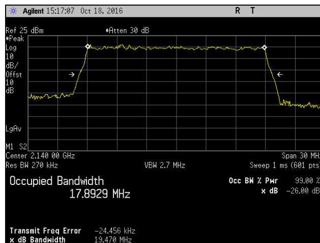
Plot 617. Occupied Bandwidth, QAM-16, Mid Channel, Band 10, Port 2, 20 MHz
