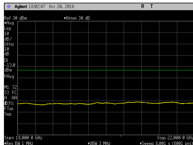
Plot 926. Spurious Emissions at Antenna Terminal, High Channel, Band 12, Port 2, 18 GHz – 22 GHz, 15 MHz
