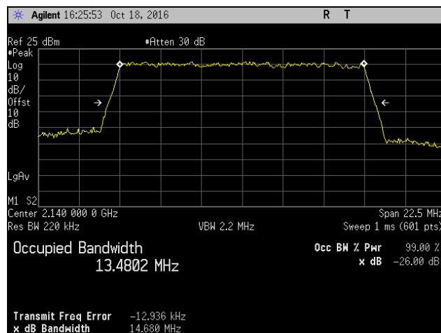
Plot 599. Occupied Bandwidth, QAM-16, Mid Channel, Band 10, Port 2, 15 MHz
