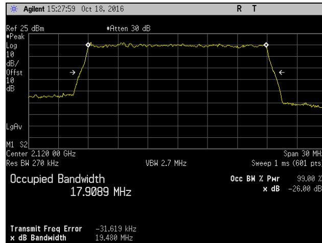
Plot 544. Occupied Bandwidth, -QAM-16, Low Channel, Band 4, Port 2, 20 MHz
