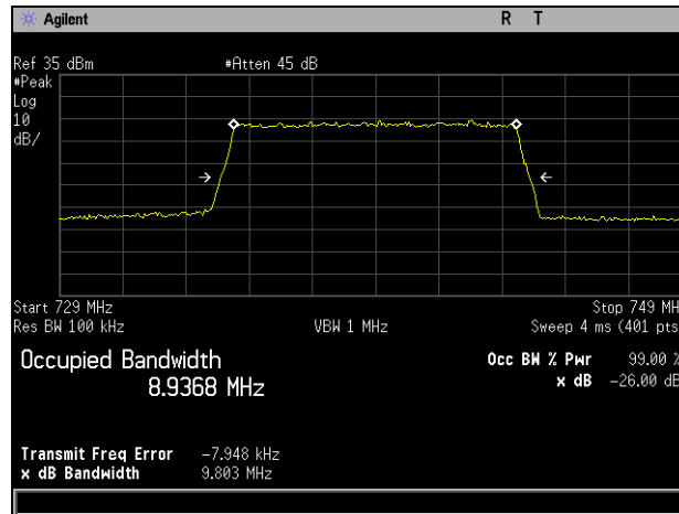
Plot 721. Occupied Bandwidth, QAM-16, Low Channel, Band 17, Port 1, 10 MHz
