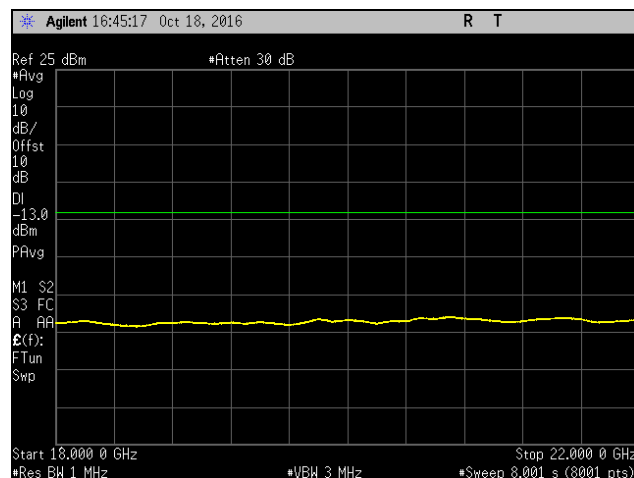
Plot 869. Spurious Emissions at Antenna Terminal, High Channel, Band 10, Port 2, 18 GHz – 22 GHz, 15 MHz
