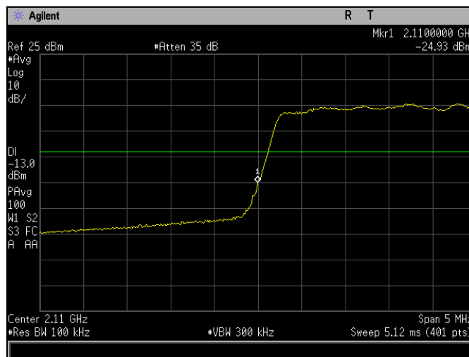
Plot 1007. Conducted Band Edge, QPSK, Low Channel, Band 4, Port 2, 5 MHz
