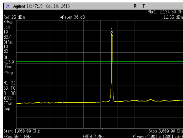
Plot 857. Spurious Emissions at Antenna Terminal, Mid Channel, Band 10, Port 2, 1 GHz – 3 GHz, 15 MHz
