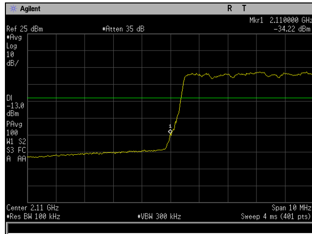
Plot 1015. Conducted Band Edge, QAM-16, Low Channel, Band 4, Port 2, 10 MHz
