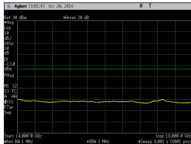
Plot 925. Spurious Emissions at Antenna Terminal, High Channel, Band 12, Port 2, 14 GHz – 18 GHz, 15 MHz
