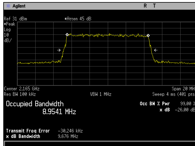
Plot 579. Occupied Bandwidth, QPSK, High Channel, Band 10, Port 1, 10 MHz
