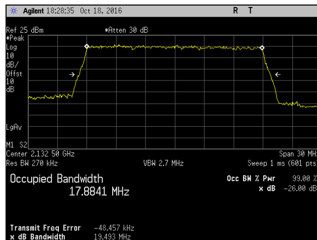
Plot 545. Occupied Bandwidth, QAM-16, Mid Channel, Band 4, Port 2, 20 MHz
