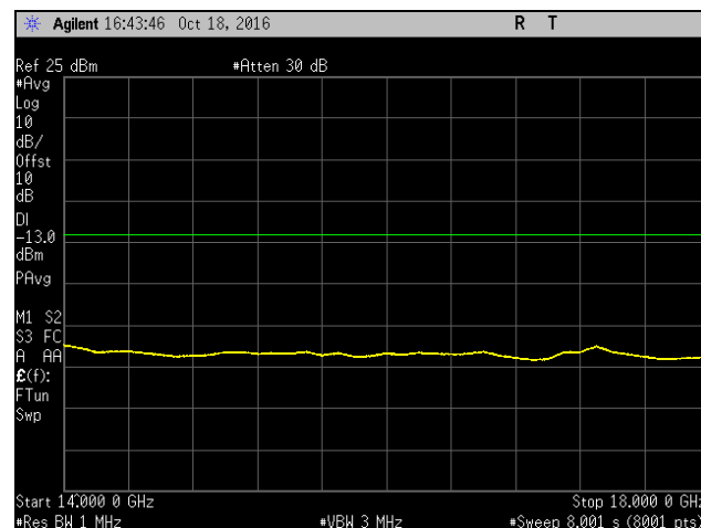
Plot 791. Spurious Emissions at Antenna Terminal, Low Channel, Band 4, Port 2, 14 GHz – 18 GHz, 15 MHz
