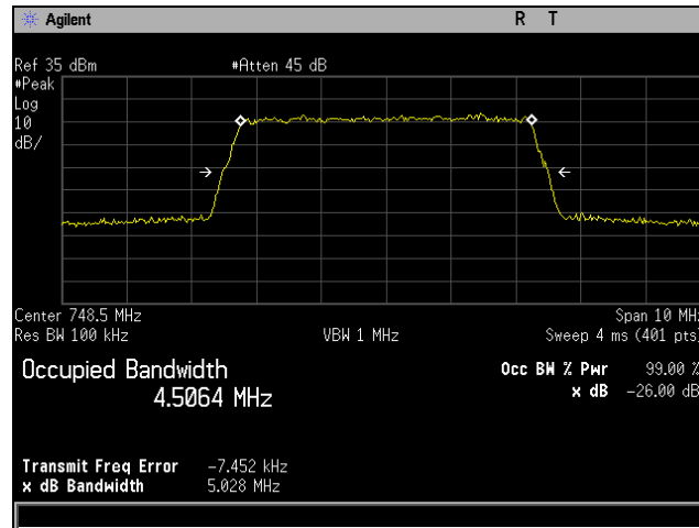
Plot 688. Occupied Bandwidth, QAM-16, Low Channel, Band 13, Port 2, 5 MHz
