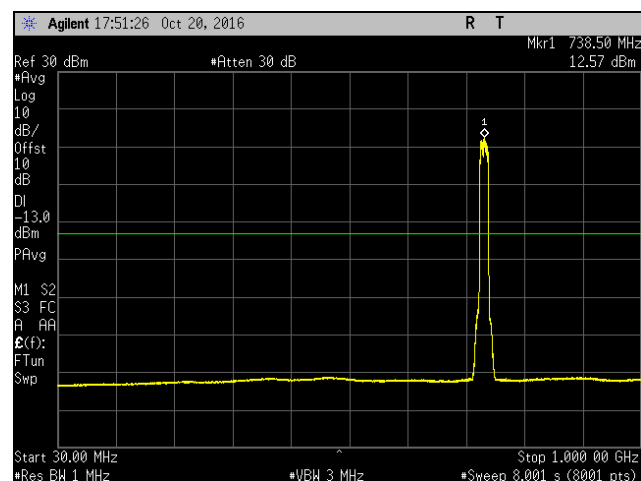
Plot 920. Spurious Emissions at Antenna Terminal, High Channel, Band 12, Port 2, 30 MHz – 1 GHz, 15 MHz
