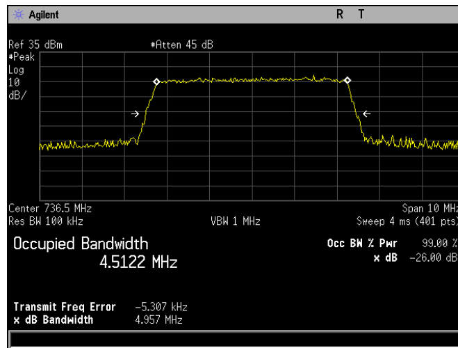
Plot 706. Occupied Bandwidth, QAM-64, Low Channel, Band 17, Port 1, 5 MHz
