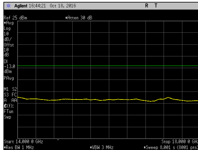
Plot 805. Spurious Emissions at Antenna Terminal, High Channel, Band 4, Port 2, 14 GHz – 18 GHz, 15 MHz
