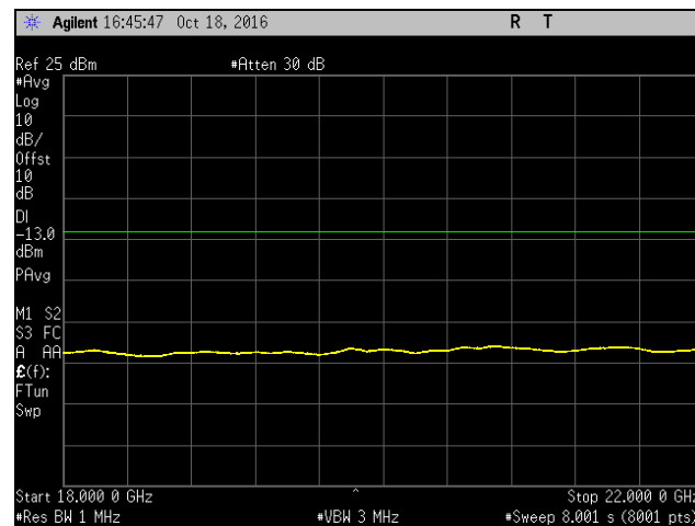
Plot 799. Spurious Emissions at Antenna Terminal, Mid Channel, Band 4, Port 2, 18 GHz – 22 GHz, 15 MHz
