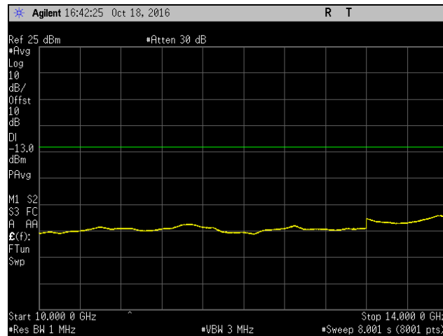
Plot 804. Spurious Emissions at Antenna Terminal, High Channel, Band 4, Port 2, 10 GHz – 14 GHz, 15 MHz
