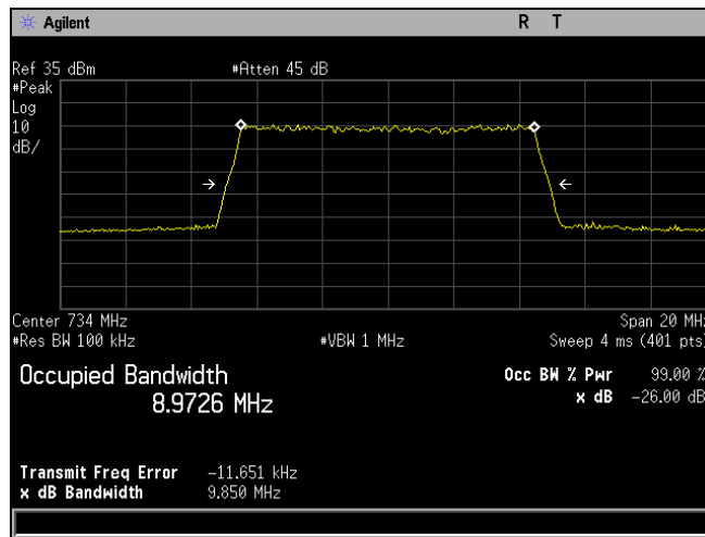
Plot 646. Occupied Bandwidth, QAM-64, Low Channel, Band 12, Port 1, 10 MHz
