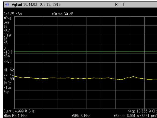
Plot 798. Spurious Emissions at Antenna Terminal, Mid Channel, Band 4, Port 2, 14 GHz – 18 GHz, 15 MHz
