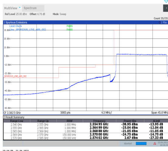
1-N38--30-15-L-6-CP-QPSK-Outer_Full-38@0-Ant0-PASS-see graph
