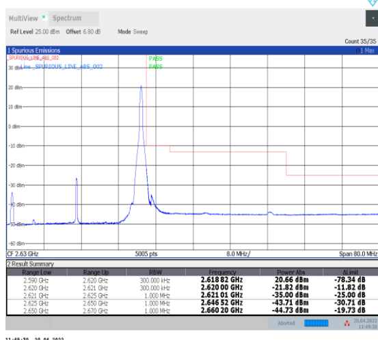
1-N38--30-30-H-5-CP-QPSK-Edge_1RB_Right-1@77-Ant0-PASS-see graph
