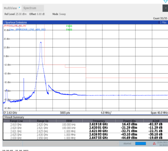
1-N38--30-10-H-5-CP-QPSK-Edge_1RB_Right-1@23- Ant0-PASS-see graph
