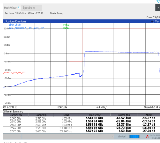
1-N38--30-30-L-6-CP-QPSK-Outer_Full-78@0-Ant0-PASS-see graph
