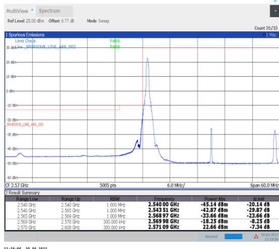
1-N38--30-30-L-1-DFT-PI2BPSK-Edge_1RB_Left-1@0-Ant0-PASS-see graph
