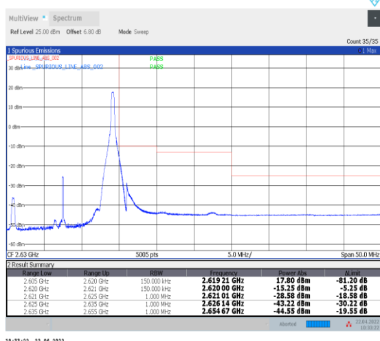
1-N38--30-15-H-5-CP-QPSK-Edge_1RB_Right-1@37-Ant0-PASS-see graph
