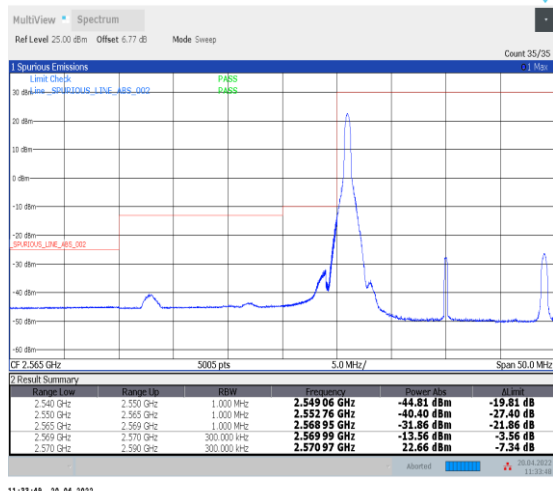
1-N38--30-20-L-1-DFT-PI2BPSK-Edge_1RB_Left-1@0-Ant0-PASS-see graph
