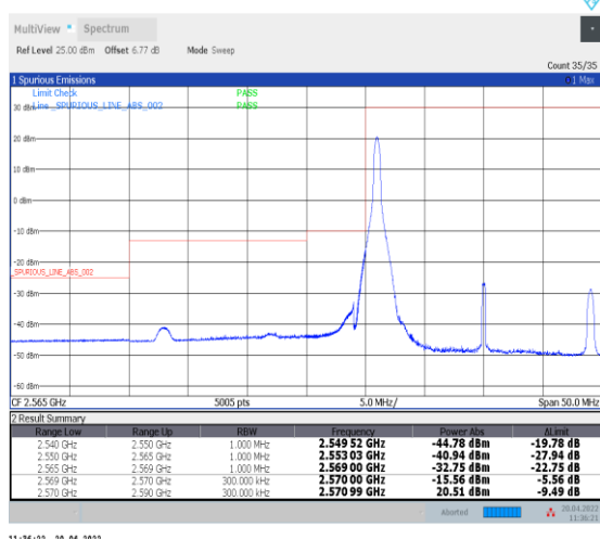
1-N38--30-20-L-4-CP-QPSK-Edge_1RB_Left-1@0-Ant0-PASS-see graph
