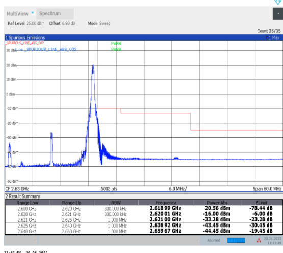
1-N38--30-20-H-5-CP-QPSK-Edge_1RB_Right-1@50- Ant0-PASS-see graph
