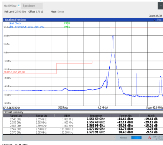
1-N38--30-15-L-1-DFT-PI2BPSK-Edge_1RB_Left-1@0-Ant0-PASS-see graph
