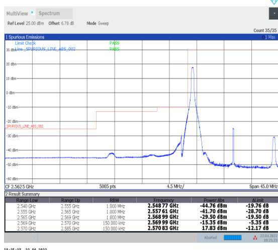
1-N38--30-15-L-4-CP-QPSK-Edge_1RB_Left-1@0-Ant0-PASS-see graph
