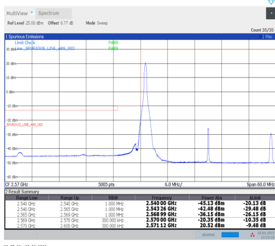
1-N38--30-30-L-4-CP-QPSK-Edge_1RB_Left-1@0-Ant0-PASS-see graph
