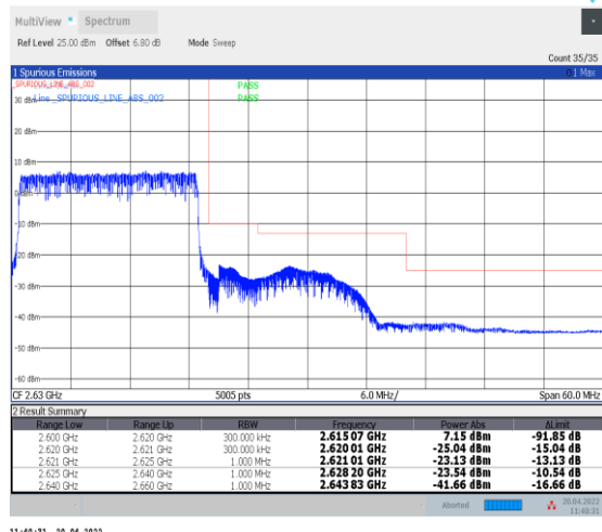
1-N38--30-20-H-3-DFT-PI2BPSK-Outer_Full-50@ 0-Ant0-PASS-see graph
