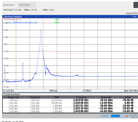
1-N38--30-15-H-2-DFT-PI2BPSK-Edge_1RB_Right-1@37-Ant0-PASS-see graph
