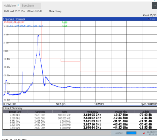
1-N38--30-10-H-2-DFT-PI2BPSK-Edge_1RB_Right-1@ 23-Ant0-PASS-see graph
