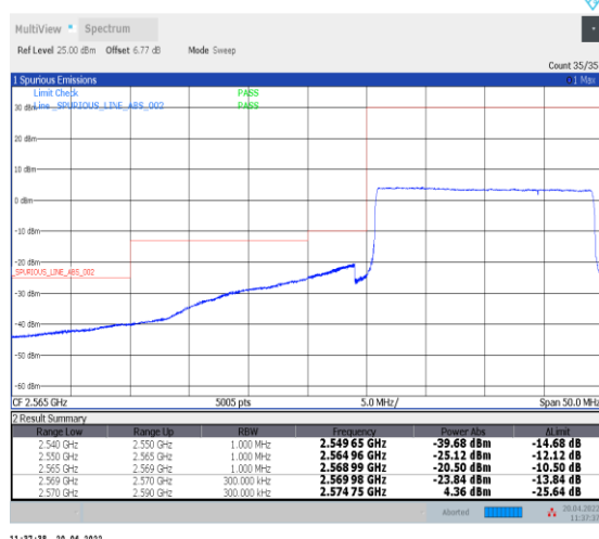
1-N38--30-20-L-6-CP-QPSK-Outer_Full-51@0-Ant0-PASS-see graph
