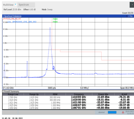
1-N38--30-30-H-2-DFT-PI2BPSK-Edge_1RB_Right-1@77-Ant0-PASS-see graph
