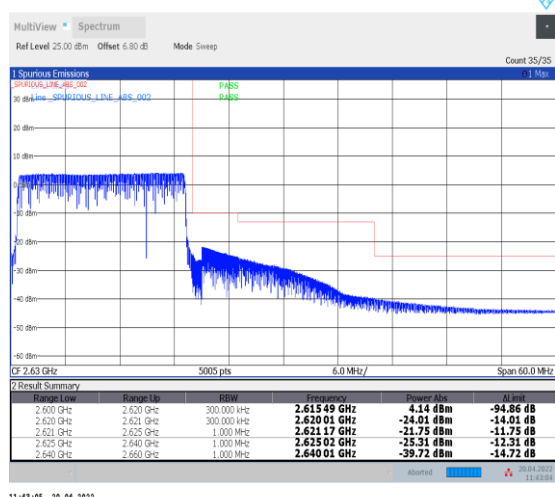
1-N38--30-20-H-6-CP-QPSK-Outer_Full-51@0-An t0-PASS-see graph
