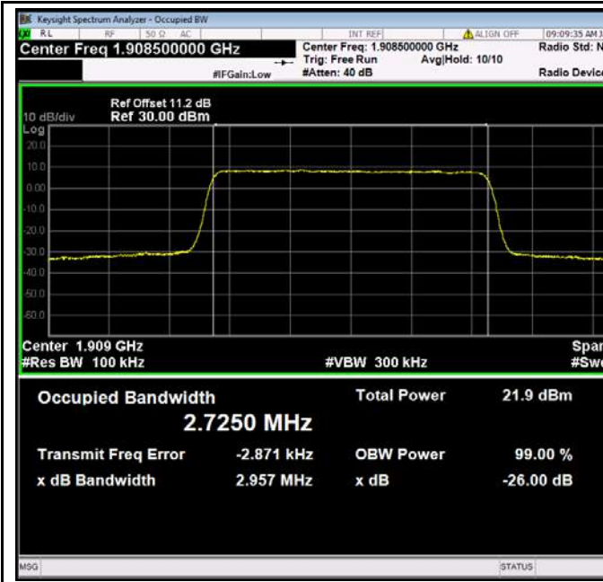
LTE band 2 - High CH QPSK-3
