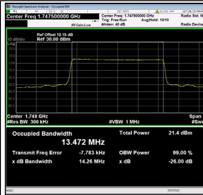
LTE band 4 - High CH QPSK-15
