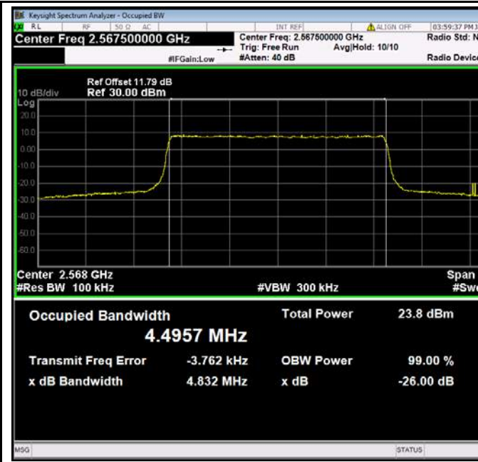
LTE band 7 - High CH QPSK-5
