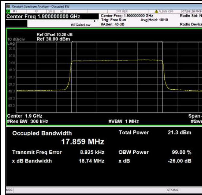
LTE band 2 - High CH QPSK-20
