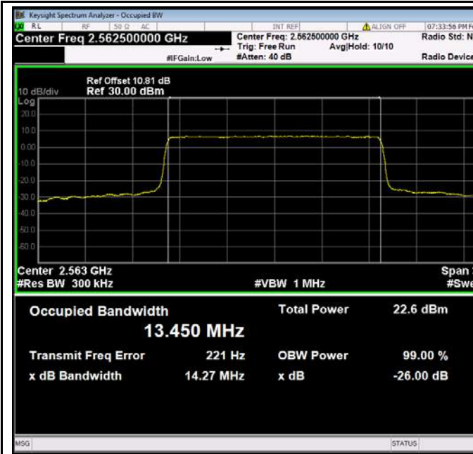
LTE band 7 - High CH QPSK-15
