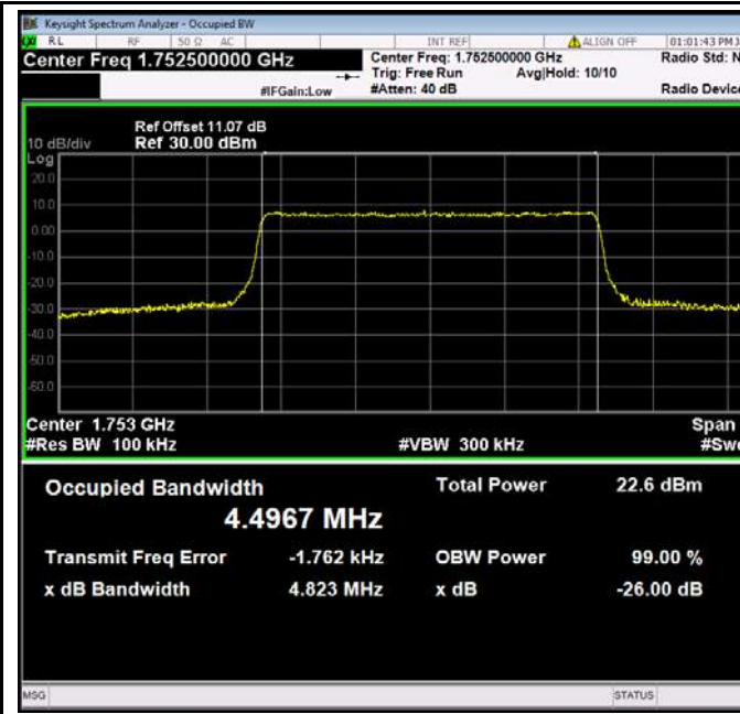
LTE band 4 - High CH QPSK-5
