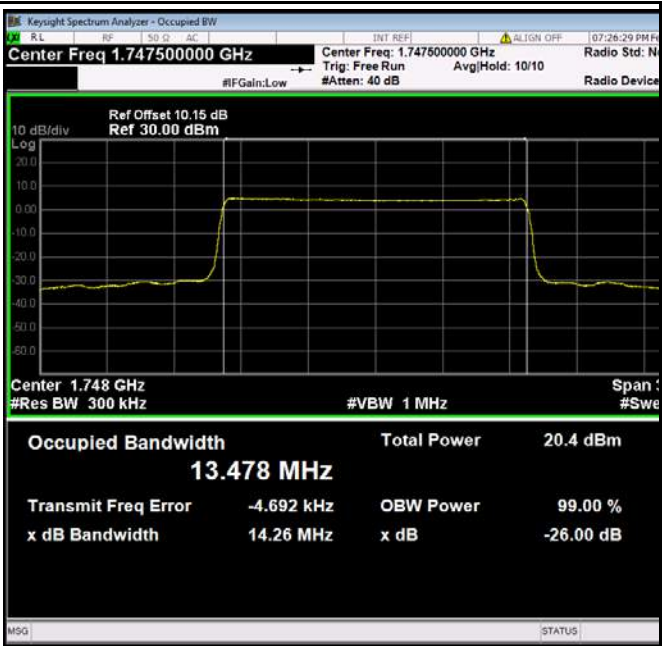
LTE band 4 - High CH 16QAM-15
