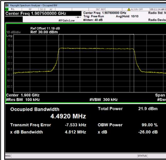
LTE band 2 - High CH QPSK-5
