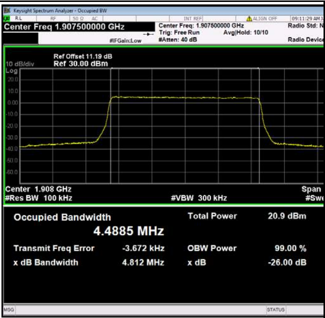
LTE band 2 - High CH 16QAM-5
