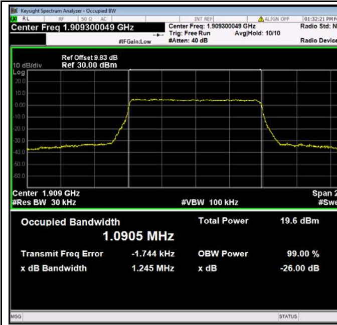
LTE band 2 - High CH QPSK-1.4
