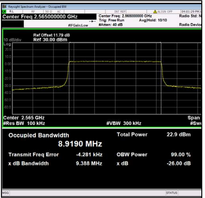
LTE band 7 - High CH 16QAM-10
