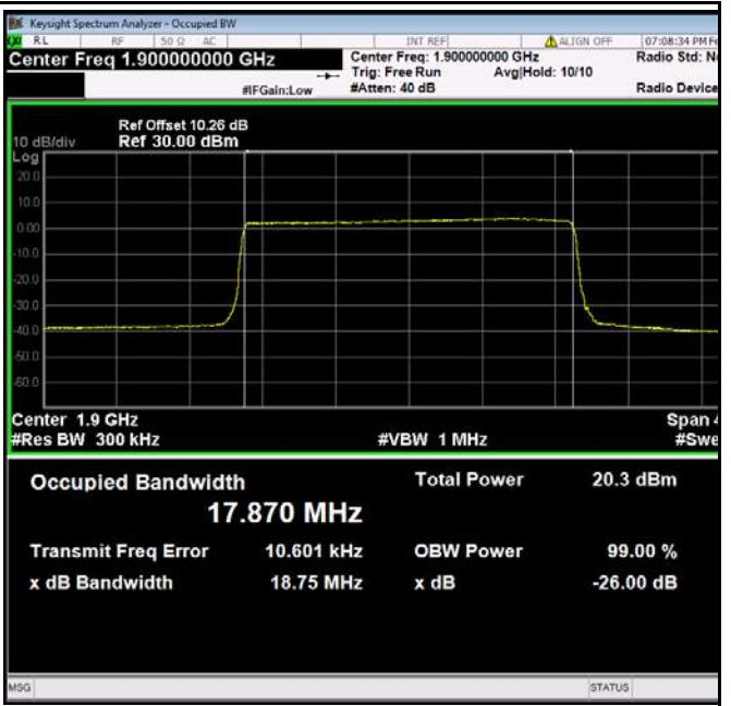
LTE band 2 - High CH 16QAM-20
