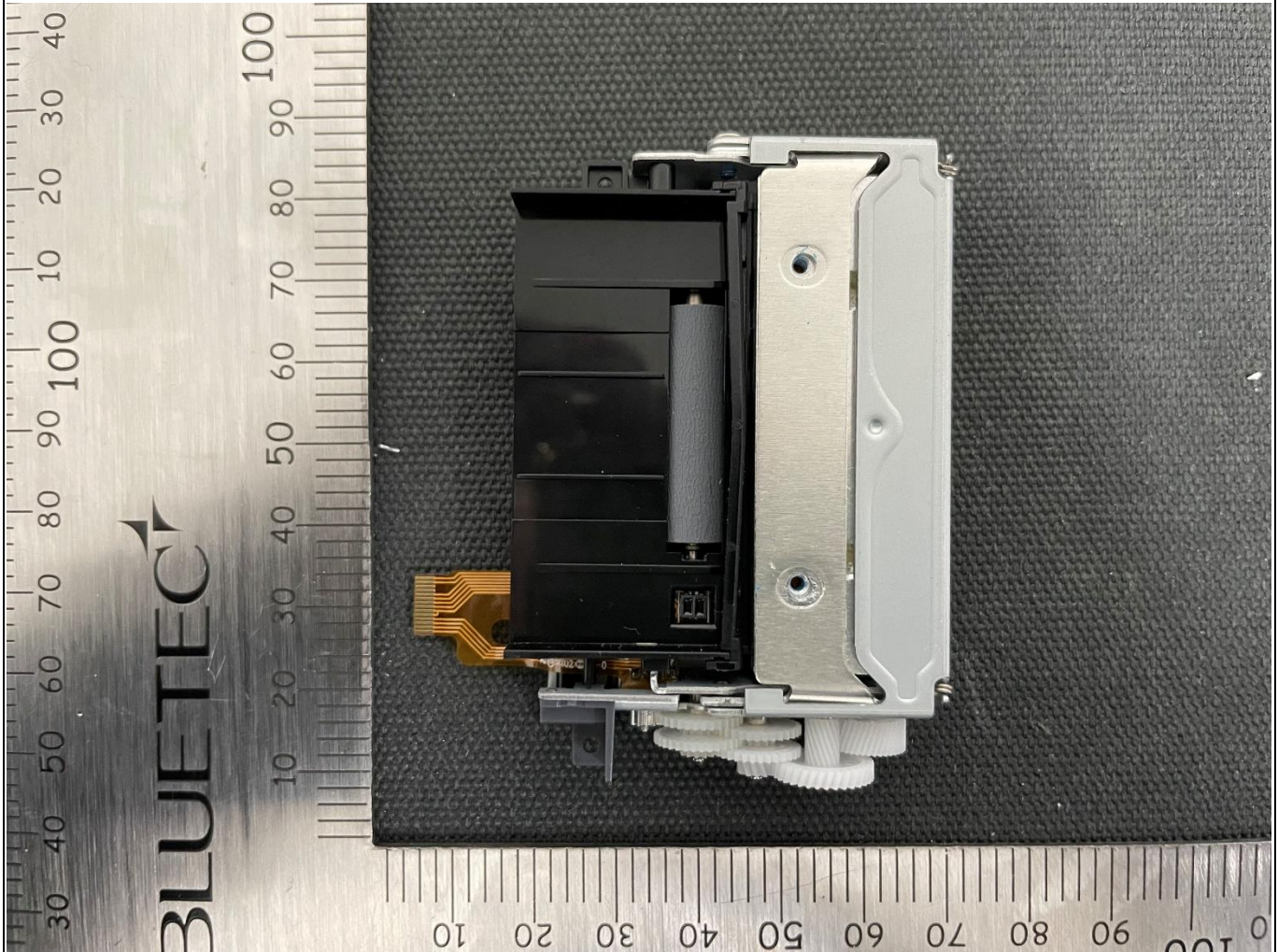
Printer_Rear
