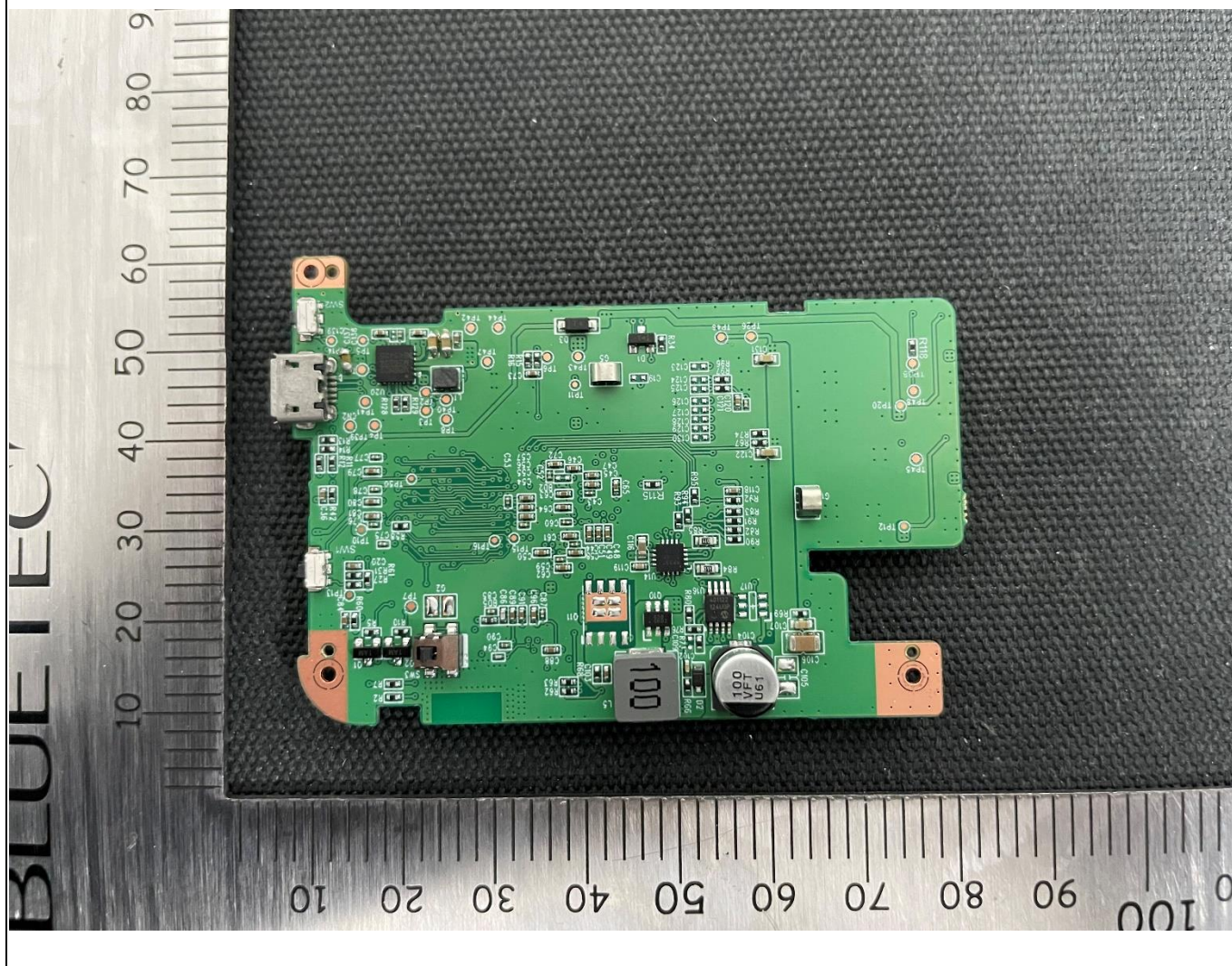
Main PCB_Rear
