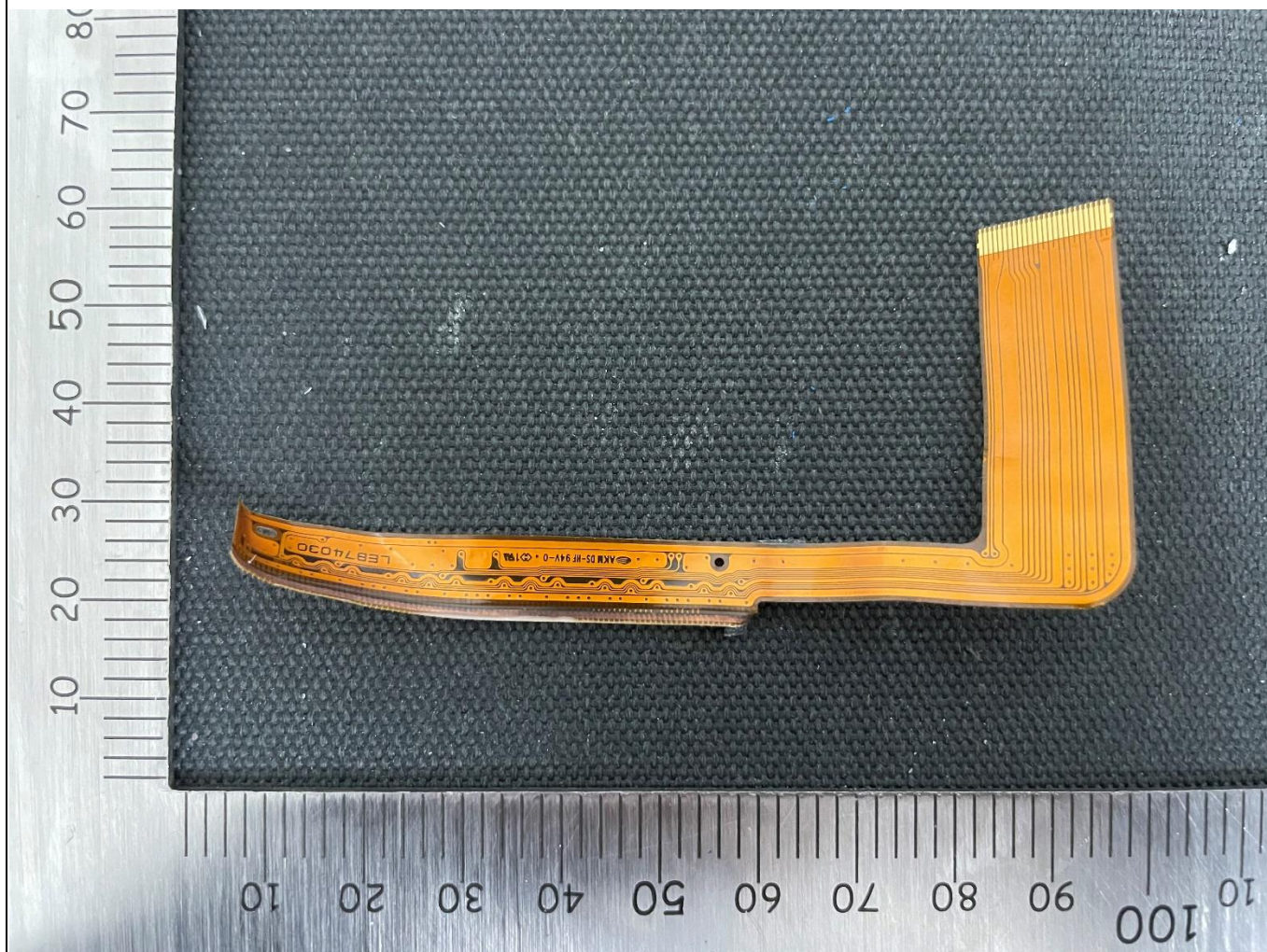
Printer FPCB_Front
