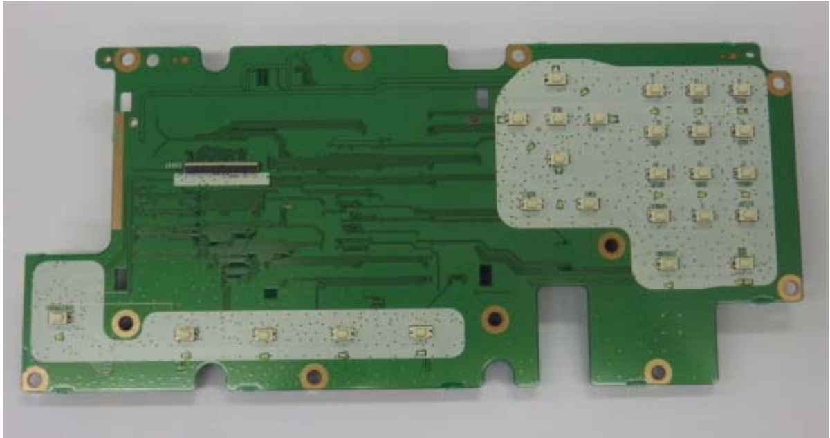
LOGIC unit (top view)
