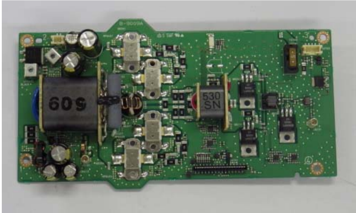
PA unit (top view)
