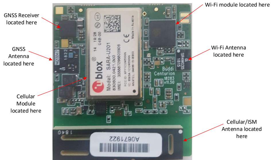
Figure 1: Smart Tag 4 PCB – top view
