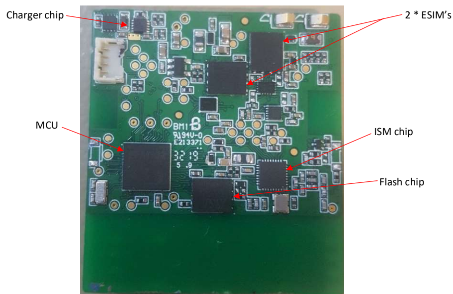
Figure 2: Smart Tag 4 PCB – bottom view
