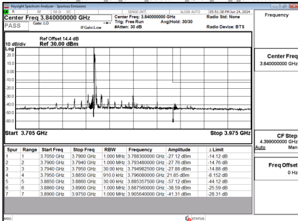
Band77-Part27_90MHz_CP_OFDM_SCS30kHz_QPSK_RB1_0_CH656000
