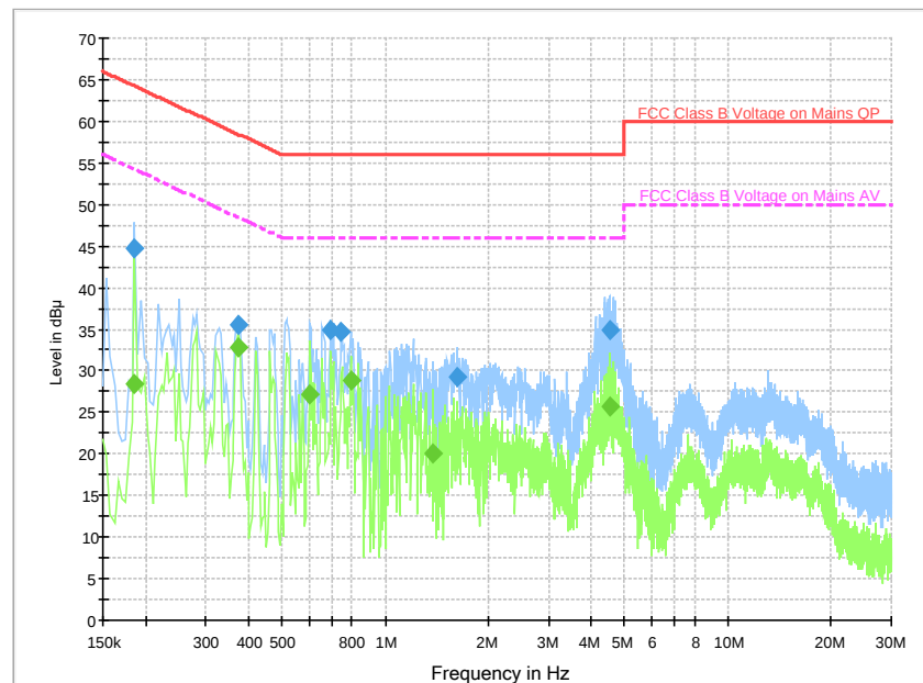
Fig. 112 AC Powerline Conducted Emission 802.11a CH169-Idle
