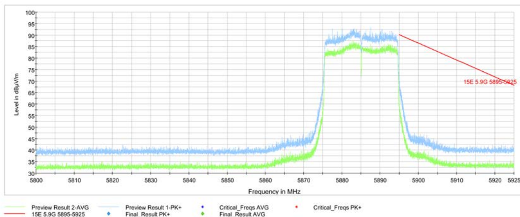
Fig. 110 Band Edges (802.11ax-HT20, 5885MHz)
