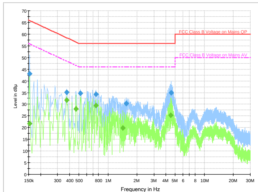
Fig. 111 AC Powerline Conducted Emission-802.11a CH169
