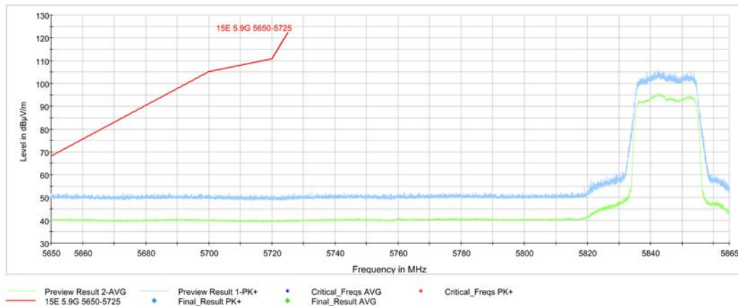
Fig. 109 Band Edges (802.11ax-HT20, 5845MHz)
