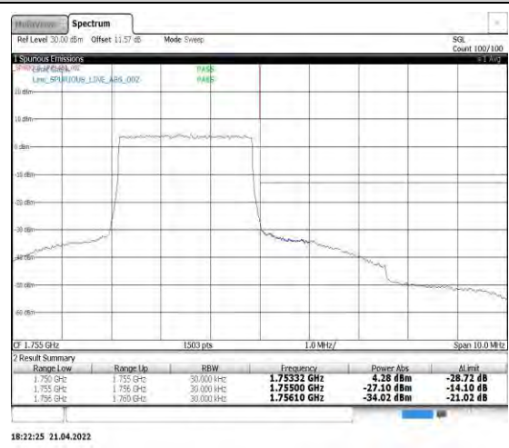
Band4-3MHz-QPSK-20385-15RB#0
