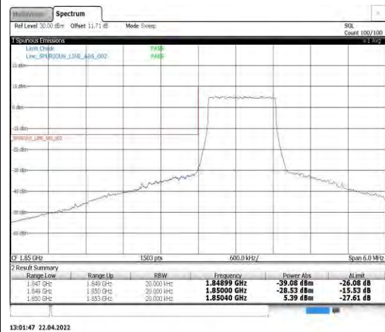
Band2-1.4MHz-16QAM-18607-6RB#0
