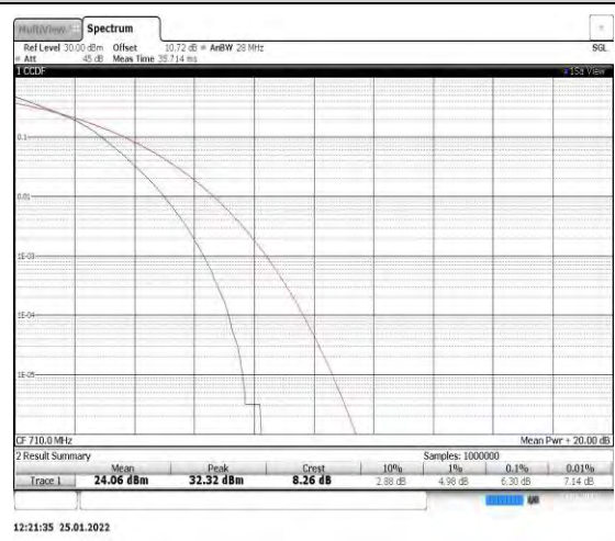
Band17-10MHz-16QAM-23790
