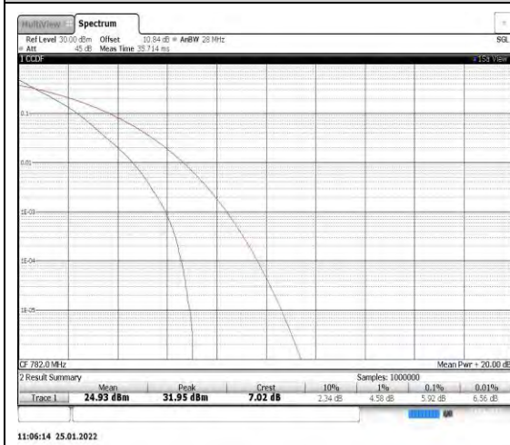
Band13-5MHz-QPSK-23230
