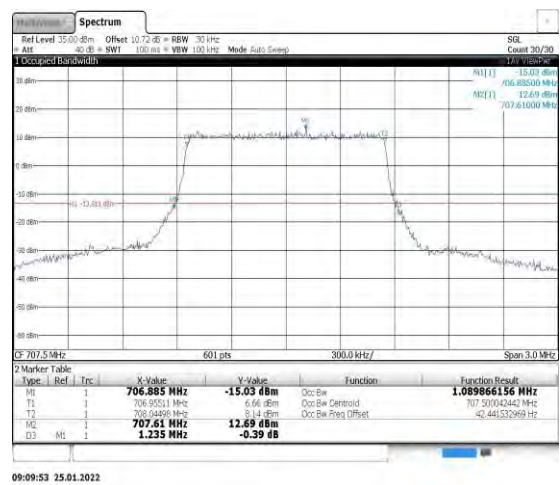
Band12-1.4MHz-16QAM-23095-6RB#0
