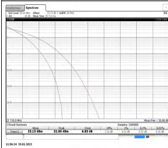
Band17-5MHz-QPSK-23790
