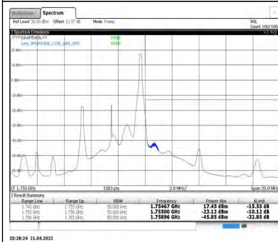
Band4-5MHz-16QAM-20375-1RB#24
