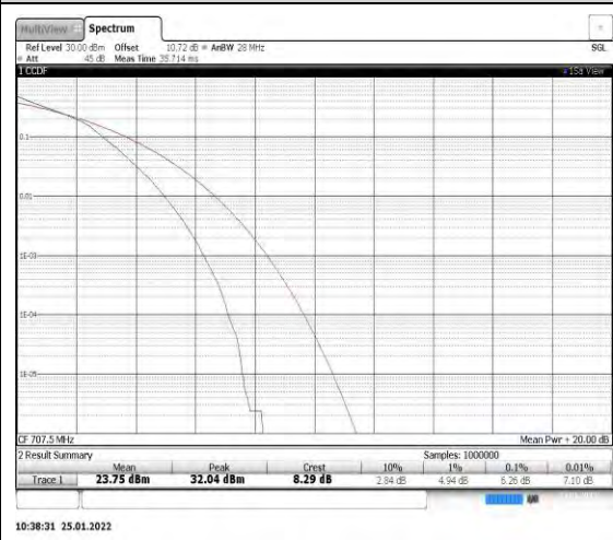
Band12-10MHz-16QAM-23095
