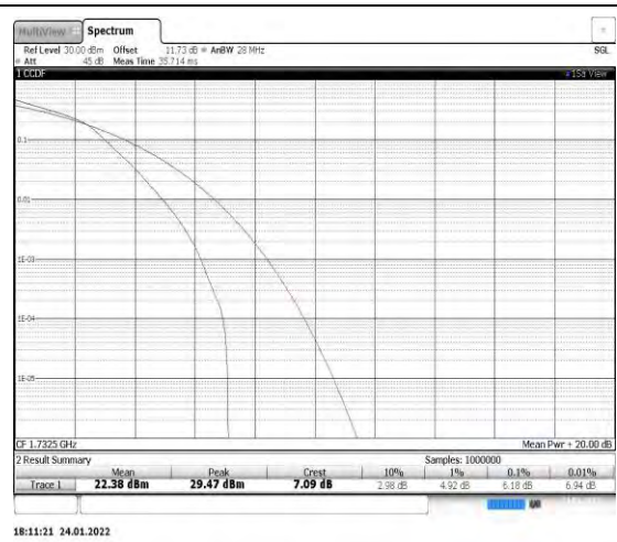
Band4-1.4MHz-16QAM-20175
