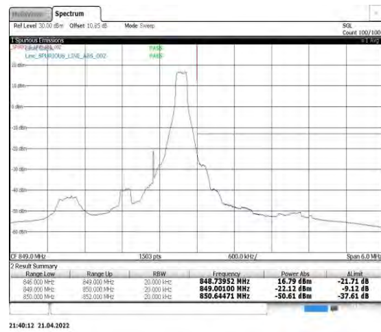
Band5-1.4MHz-QPSK-20643-1RB#5
