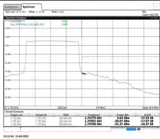
Band4-15MHz-QPSK-20325-75RB#0
