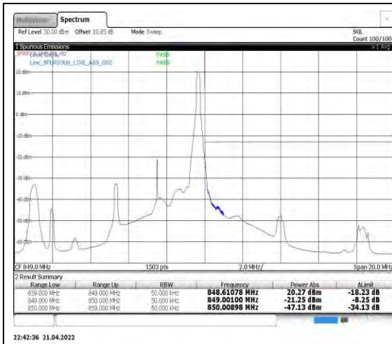
Band5-5MHz-QPSK-20625-1RB#24
