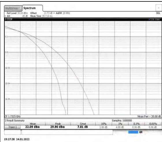
Band4-10MHz-16QAM-20175
