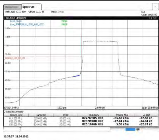
Band5-5MHz-16QAM-20425-25RB#0
