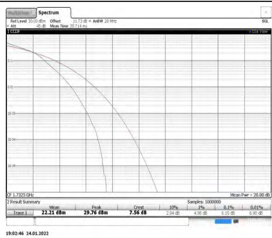
Band4-5MHz-16QAM-20175
