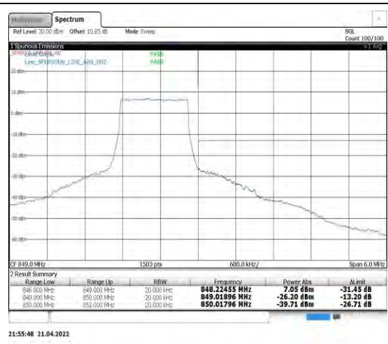
Band5-1.4MHz-16QAM-20643-6RB#0
