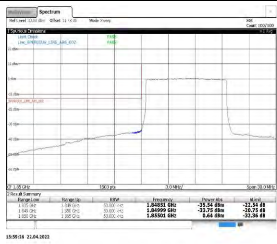
Band2-10MHz-16QAM-18650-50RB#0
