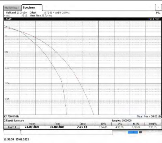
Band17-5MHz-16QAM-23790
