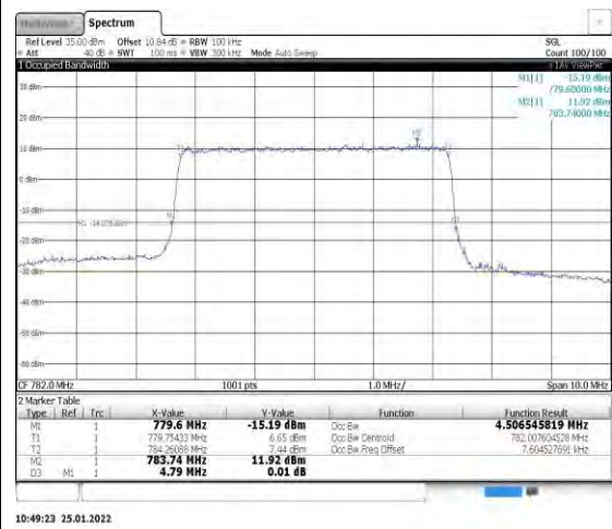
Band13-5MHz-16QAM-23230-25RB#0
