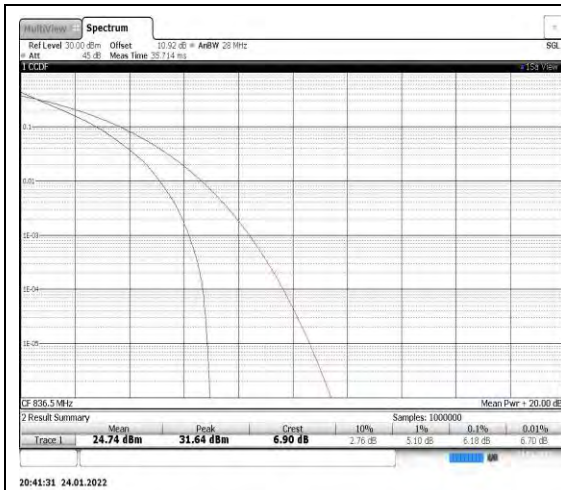
Band5-1.4MHz-QPSK-20525
