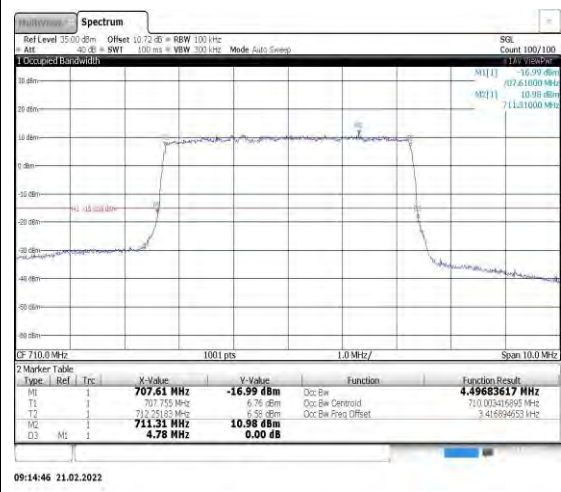
Band17-5MHz-16QAM-23790-25RB#0
