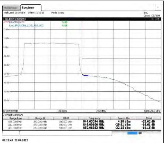
Band5-10MHz-16QAM-20600-50RB#0
