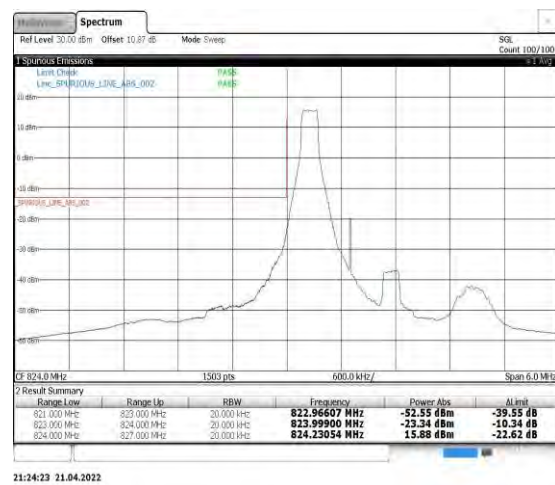
Band5-1.4MHz-16QAM-20407-1RB#0
