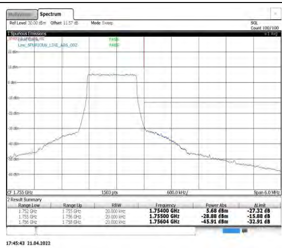
Band4-1.4MHz-16QAM-20393-6RB#0
