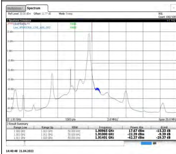
Band2-5MHz-16QAM-19175-1RB#24
