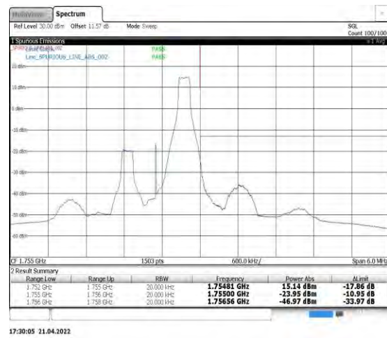
Band4-1.4MHz-QPSK-20393-1RB#5
