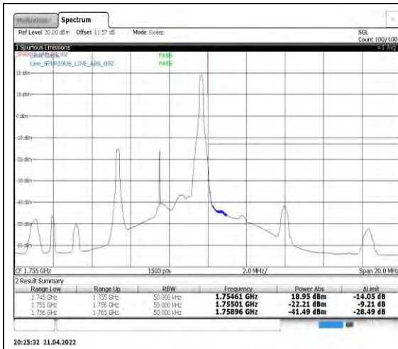
Band4-5MHz-QPSK-20375-1RB#24
