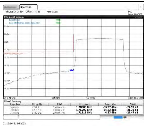
Band4-15MHz-16QAM-20025-75RB#0
