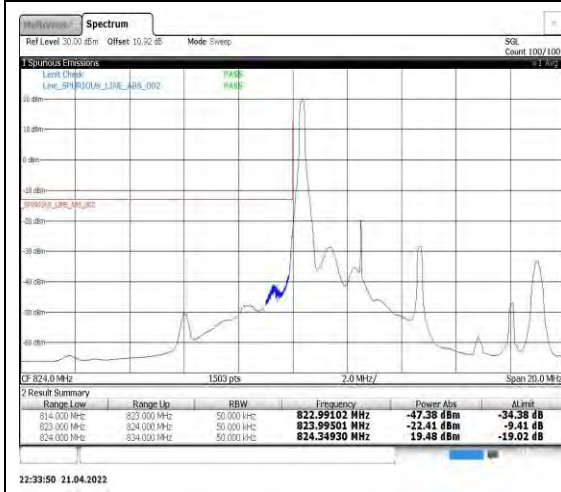
Band5-5MHz-16QAM-20425-1RB#0
