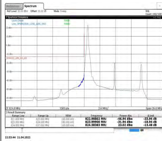
Band5-10MHz-16QAM-20450-1RB#0
