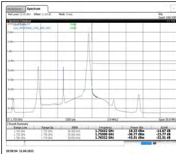
Band4-10MHz-16QAM-20350-1RB#49
