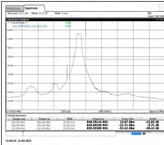
Band5-1.4MHz-16QAM-20643-1RB#5
