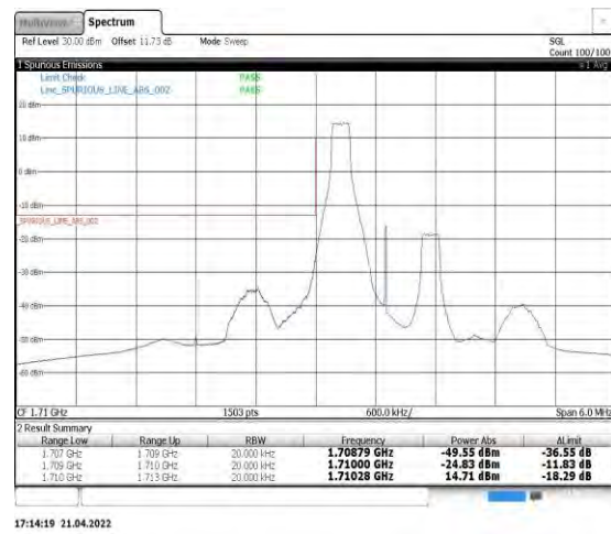
Band4-1.4MHz-16QAM-19957-1RB#0
