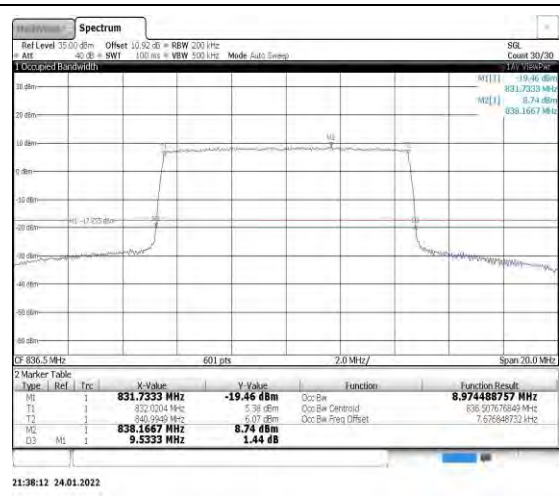
Band5-10MHz-16QAM-20525-50RB#0
