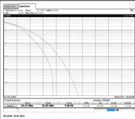
Band12-1.4MHz-16QAM-23095
