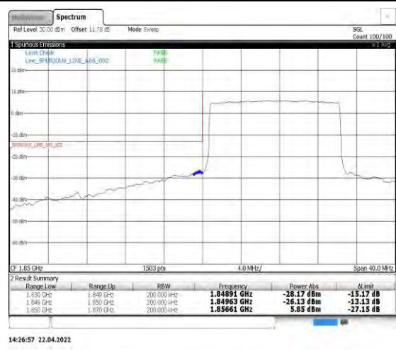
Band2-15MHz-QPSK-18675-75RB#0
