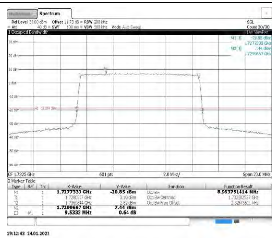
Band4-10MHz-16QAM-20175-50RB#0
