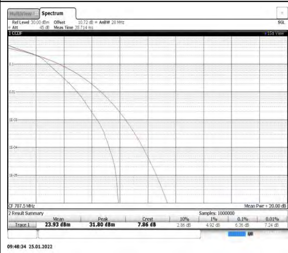
Band12-3MHz-16QAM-23095
