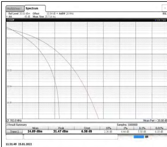
Band13-10MHz-QPSK-23230
