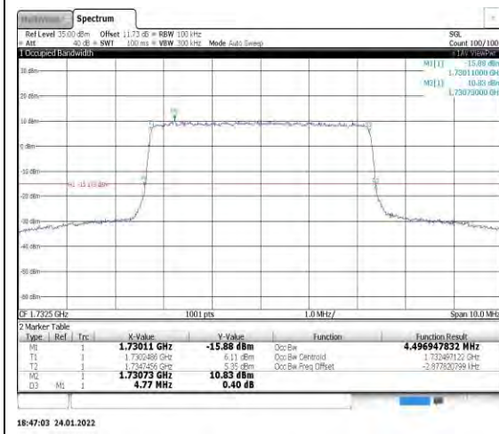
Band4-5MHz-QPSK-20175-25RB#0
