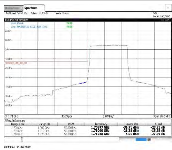
Band4-5MHz-QPSK-19975-25RB#0
