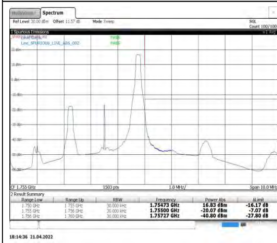
Band4-3MHz-QPSK-20385-1RB#14
