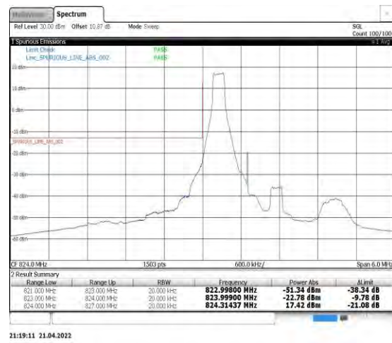
Band5-1.4MHz-QPSK-20407-1RB#0
