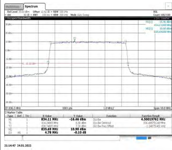
Band5-5MHz-16QAM-20525-25RB#0
