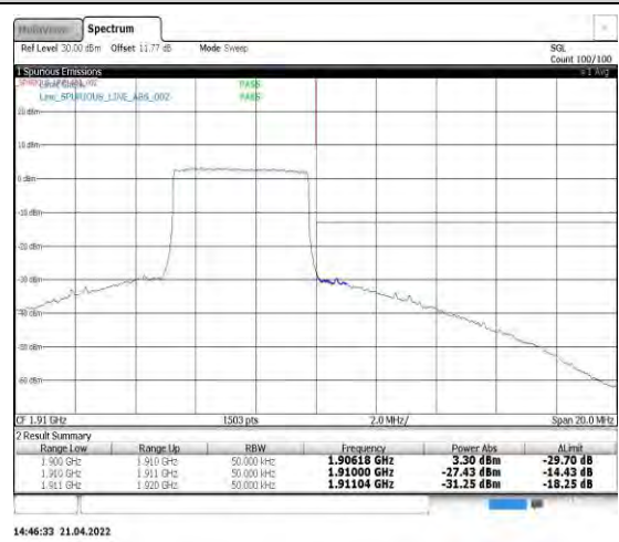
Band2-5MHz-16QAM-19175-25RB#0
