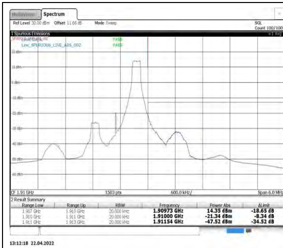
Band2-1.4MHz-16QAM-19193-1RB#5
