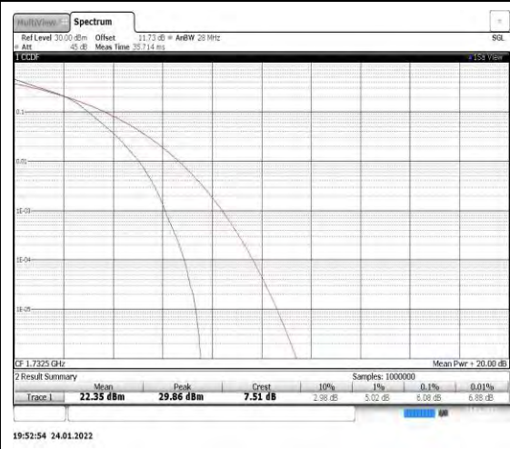
Band4-15MHz-16QAM-20175
