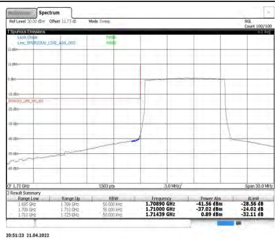
Band4-10MHz-16QAM-20000-50RB#0
