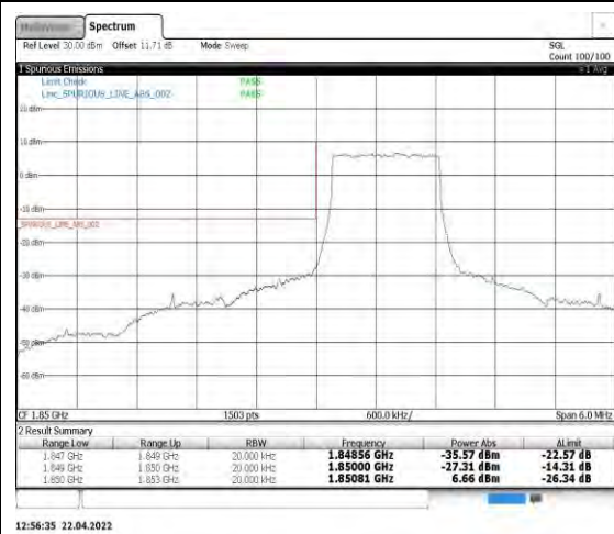
Band2-1.4MHz-QPSK-18607-6RB#0
