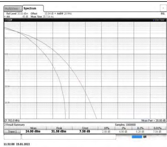
Band13-10MHz-16QAM-23230
