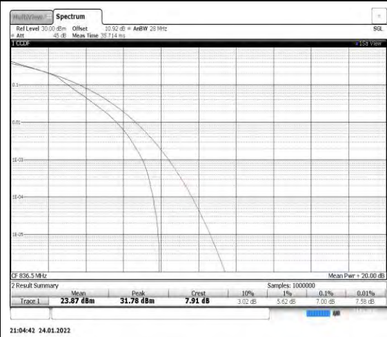
Band5-3MHz-16QAM-20525
