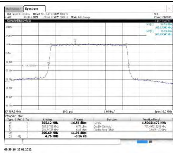
Band12-5MHz-16QAM-23095-25RB#0
