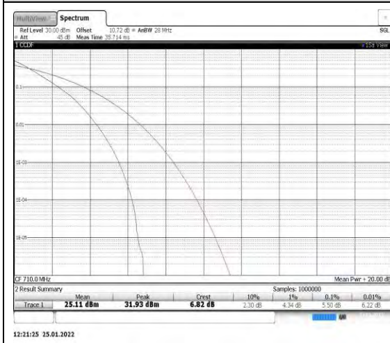
Band17-10MHz-QPSK-23790
