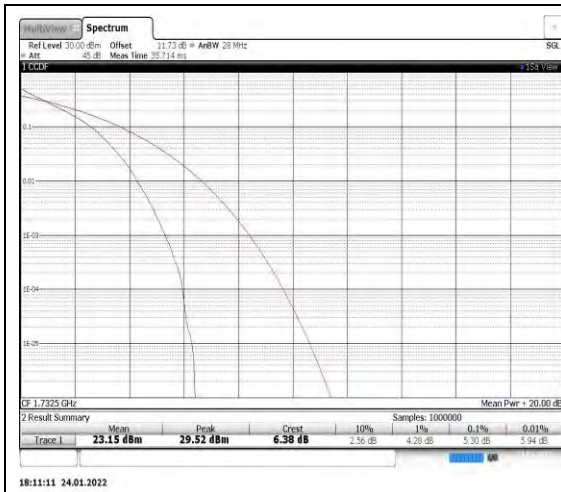
Band4-1.4MHz-QPSK-20175
