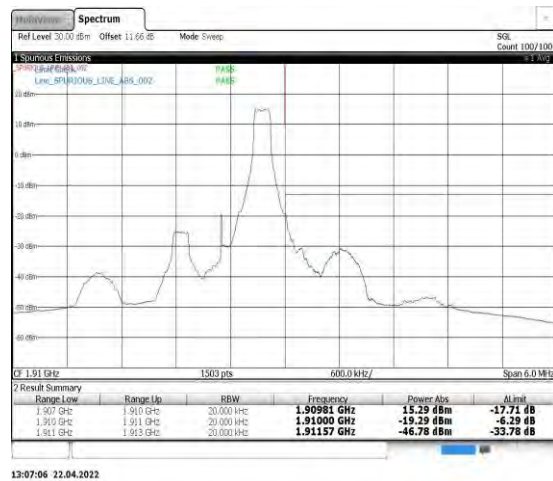
Band2-1.4MHz-QPSK-19193-1RB#5
