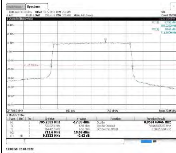
Band17-10MHz-QPSK-23790-50RB#0
