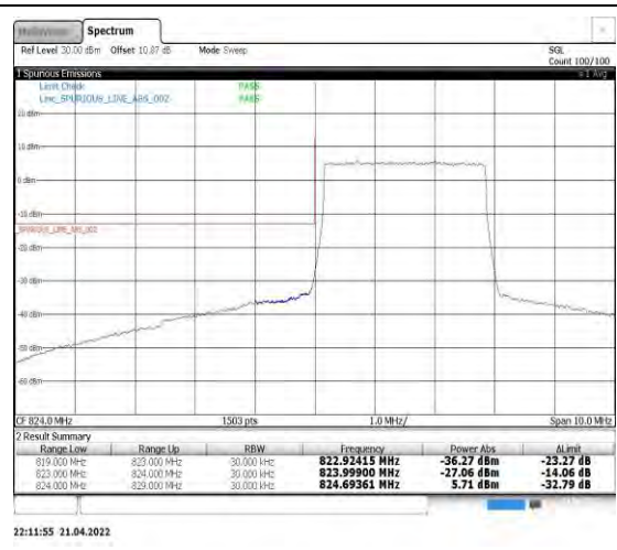
Band5-3MHz-16QAM-20415-15RB#0
