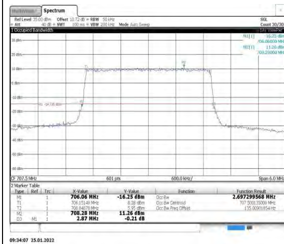
Band12-3MHz-QPSK-23095-15RB#0
