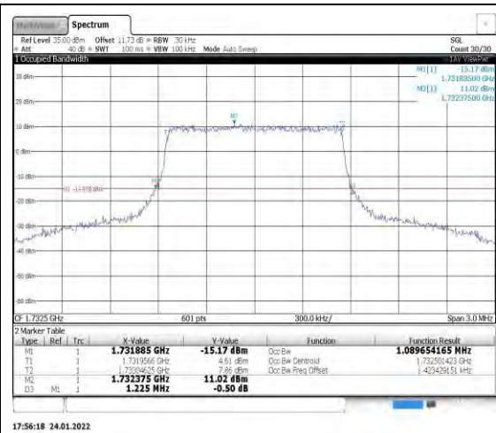
Band4-1.4MHz-16QAM-20175-6RB#0
