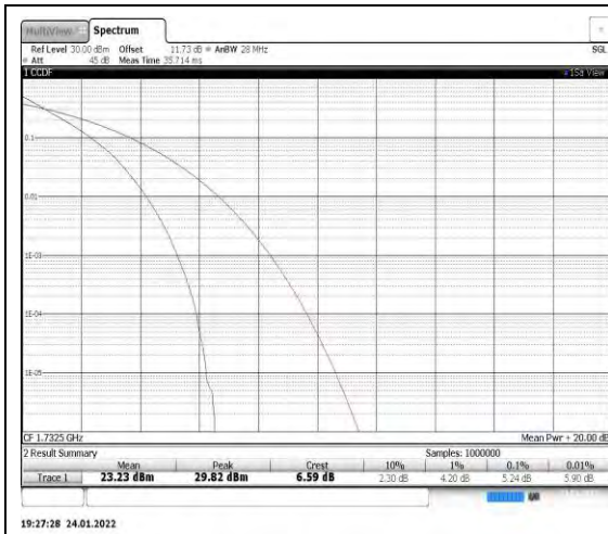
Band4-10MHz-QPSK-20175
