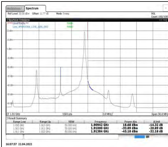
Band2-10MHz-16QAM-19150-1RB#49
