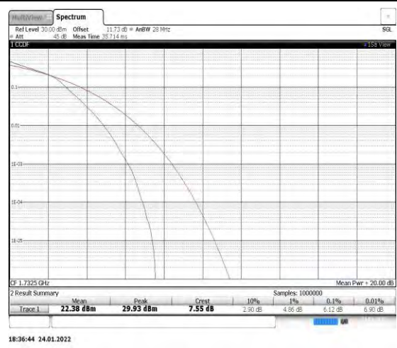
Band4-3MHz-16QAM-20175
