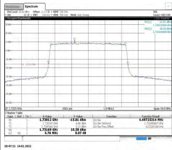
Band4-5MHz-16QAM-20175-25RB#0
