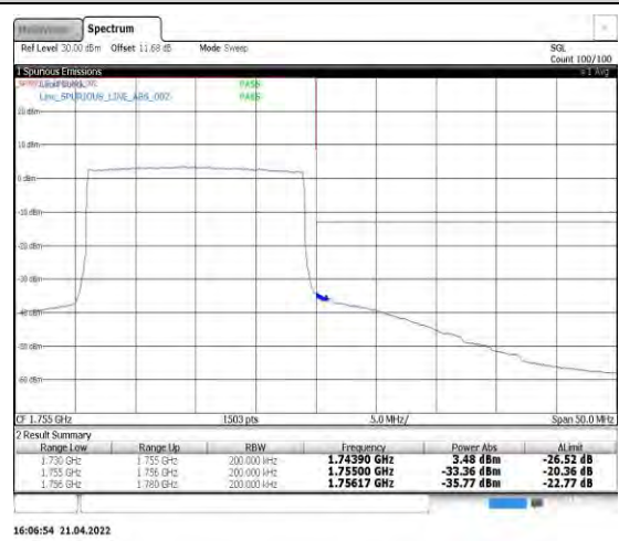
Band4-20MHz-16QAM-20300-100RB#0
