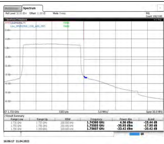
Band4-20MHz-QPSK-20300-100RB#0
