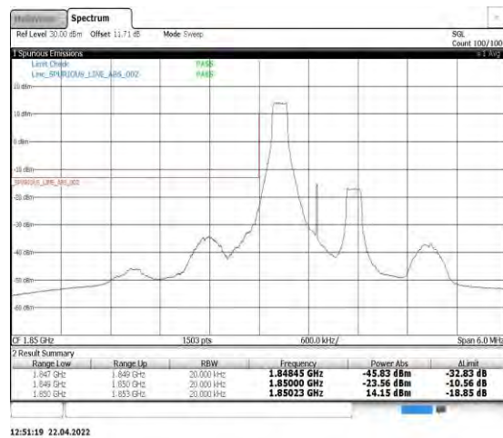
Band2-1.4MHz-16QAM-18607-1RB#0
