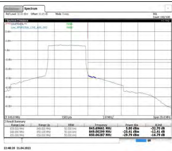
Band5-5MHz-QPSK-20625-25RB#0
