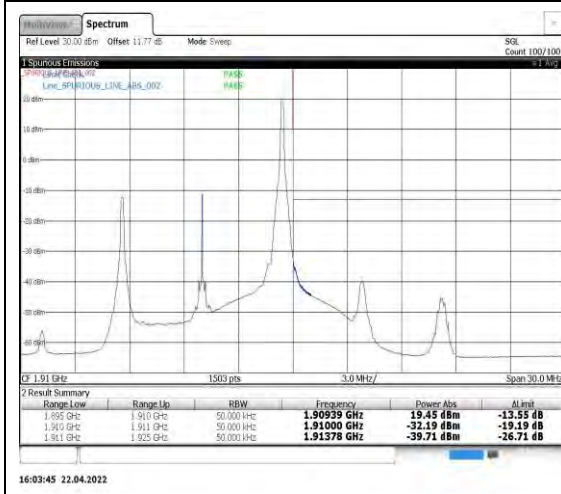
Band2-10MHz-QPSK-19150-1RB#49
