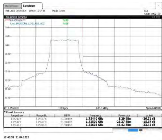
Band4-1.4MHz-QPSK-20393-6RB#0
