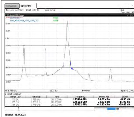
Band4-15MHz-QPSK-20325-1RB#74
