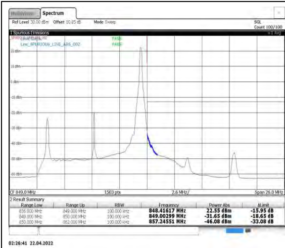
Band5-10MHz-16QAM-20600-1RB#49
