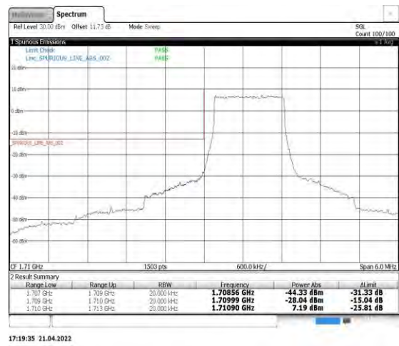
Band4-1.4MHz-QPSK-19957-6RB#0
