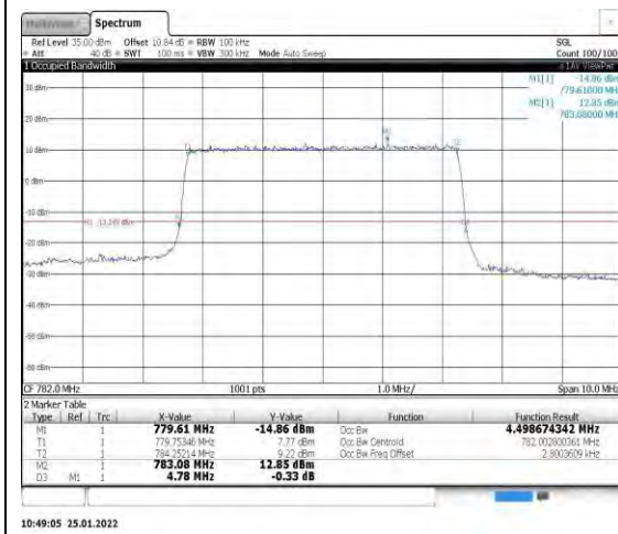
Band13-5MHz-QPSK-23230-25RB#0
