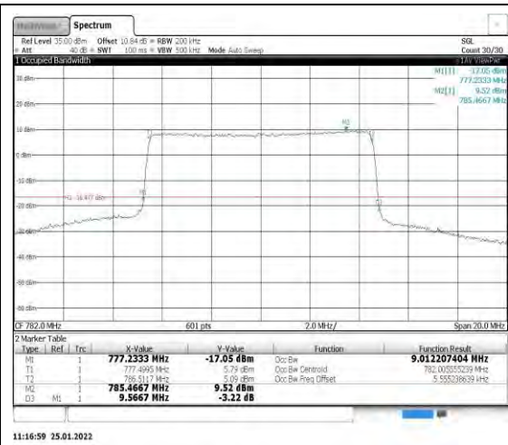
Band13-10MHz-16QAM-23230-50RB#0
