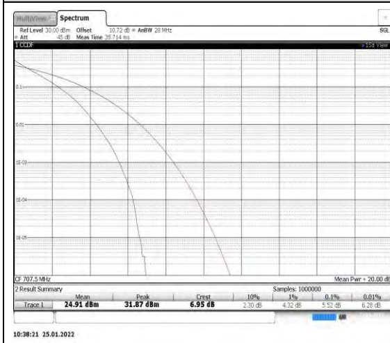
Band12-10MHz-QPSK-23095
