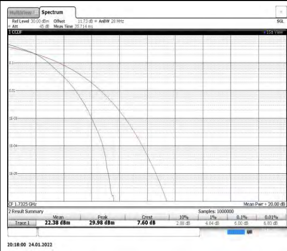
Band4-20MHz-16QAM-20175
