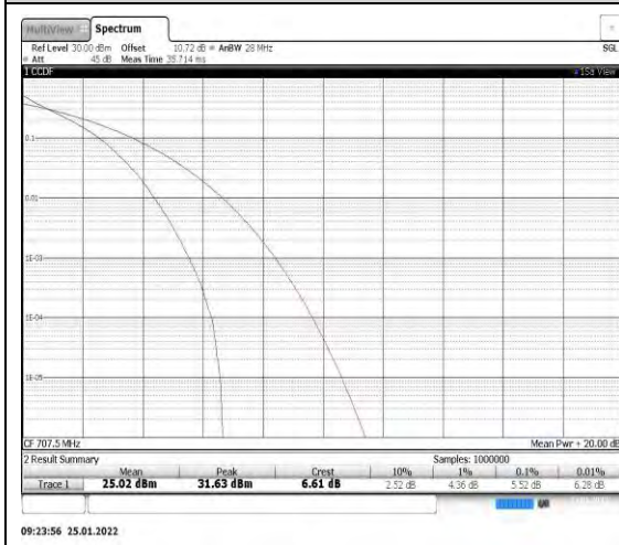
Band12-1.4MHz-QPSK-23095
