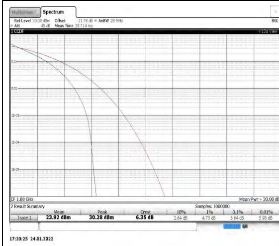
Band2-15MHz-QPSK-18900
