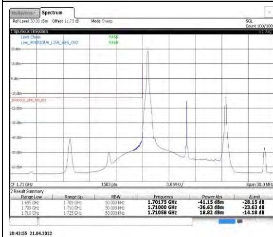
Band4-10MHz-16QAM-20000-1RB#0
