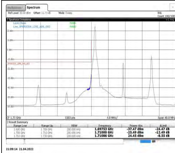
Band4-15MHz-QPSK-20025-1RB#0
