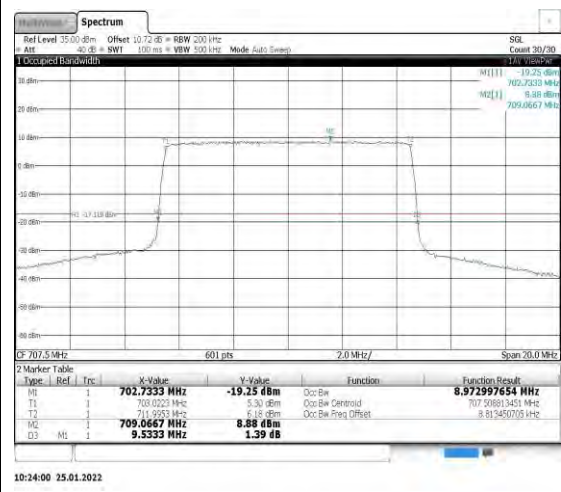
Band12-10MHz-16QAM-23095-50RB#0
