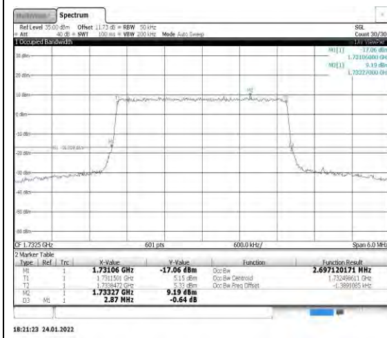
Band4-3MHz-QPSK-20175-15RB#0
