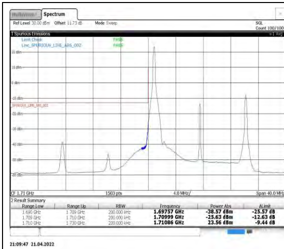
Band4-15MHz-16QAM-20025-1RB#0
