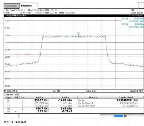
Band5-3MHz-16QAM-20525-15RB#0
