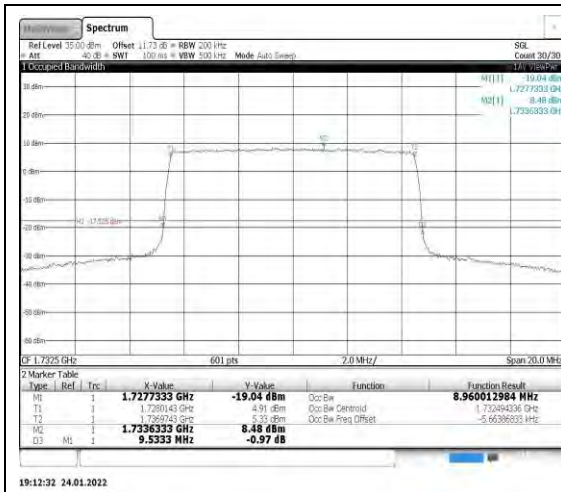
Band4-10MHz-QPSK-20175-50RB#0
