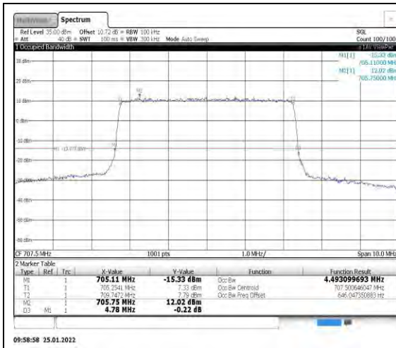
Band12-5MHz-QPSK-23095-25RB#0
