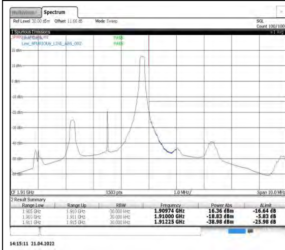
Band2-3MHz-16QAM-19185-1RB#14
