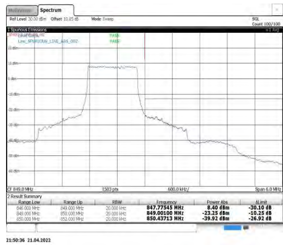
Band5-1.4MHz-QPSK-20643-6RB#0
