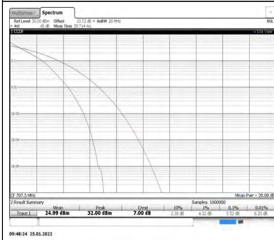
Band12-3MHz-QPSK-23095
