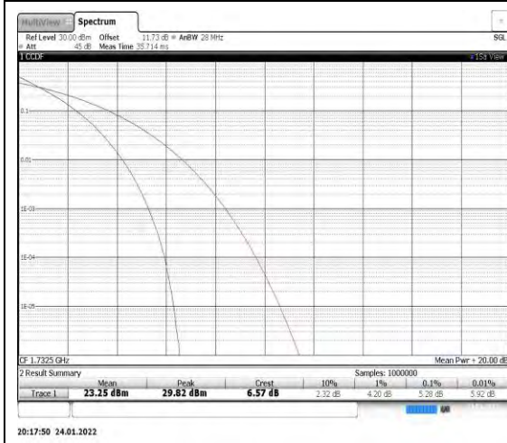
Band4-20MHz-QPSK-20175
