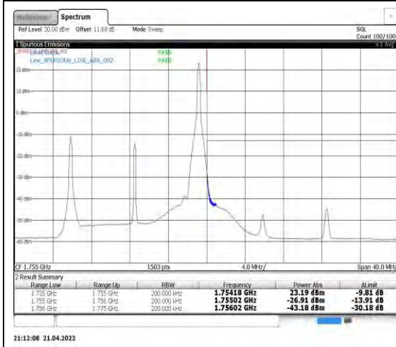
Band4-15MHz-16QAM-20325-1RB#74
