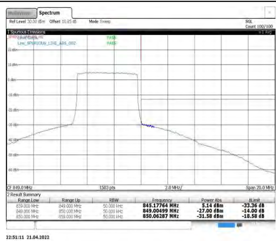
Band5-5MHz-16QAM-20625-25RB#0
