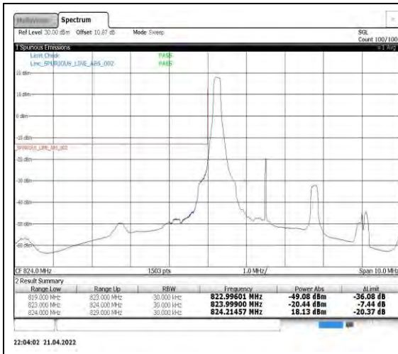
Band5-3MHz-16QAM-20415-1RB#0
