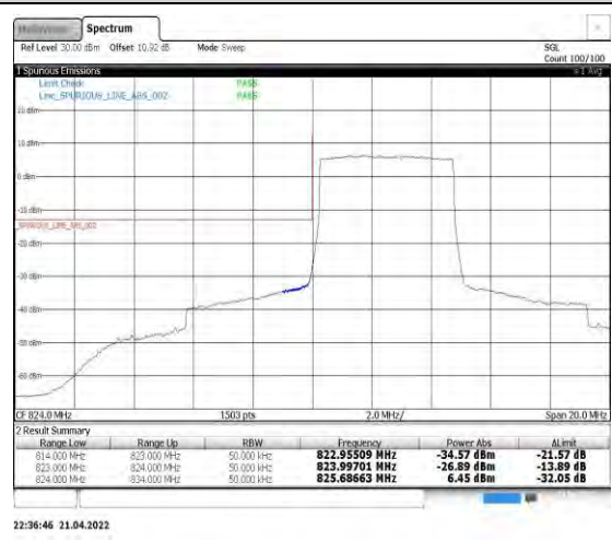
Band5-5MHz-QPSK-20425-25RB#0
