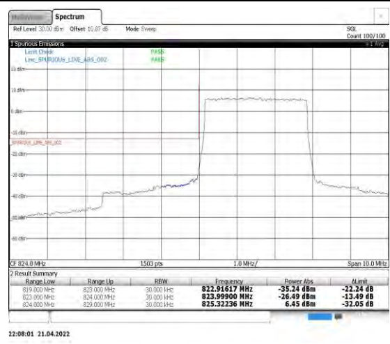
Band5-3MHz-QPSK-20415-15RB#0
