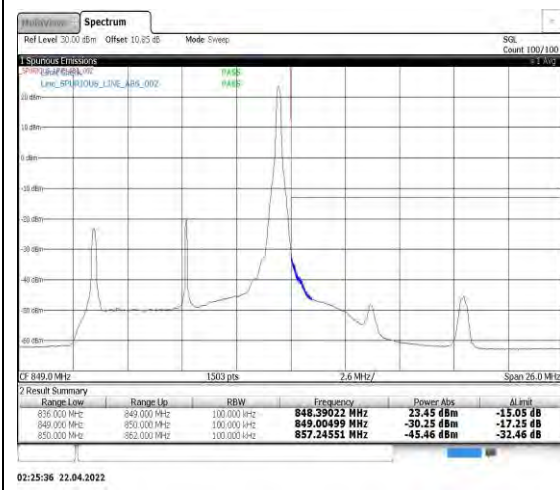
Band5-10MHz-QPSK-20600-1RB#49
