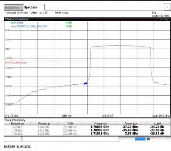
Band4-20MHz-16QAM-20050-100RB#0
