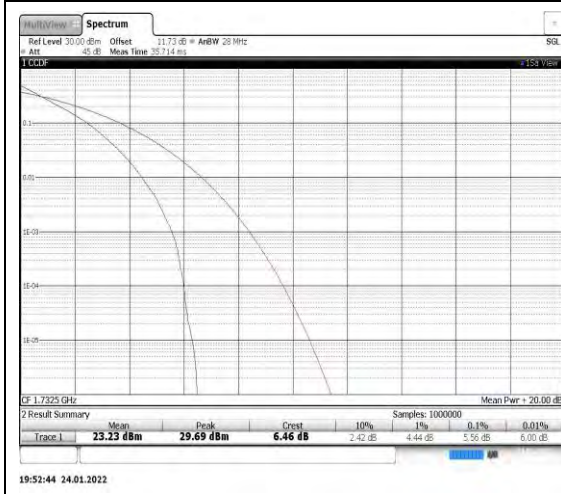
Band4-15MHz-QPSK-20175
