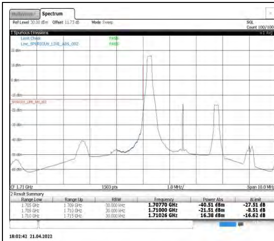
Band4-3MHz-16QAM-19965-1RB#0
