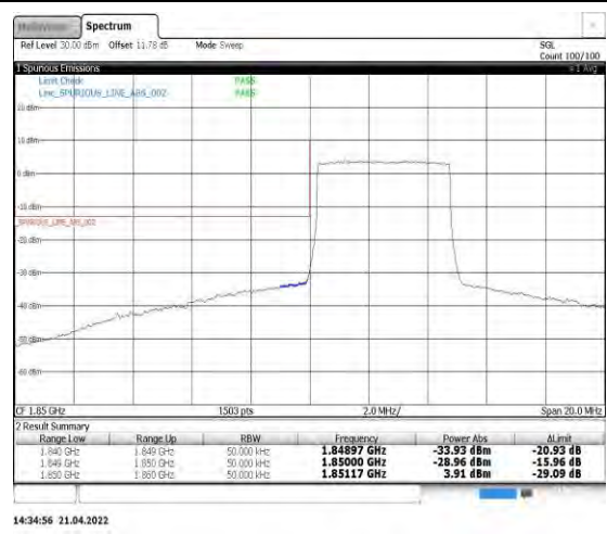
Band2-5MHz-16QAM-18625-25RB#0
