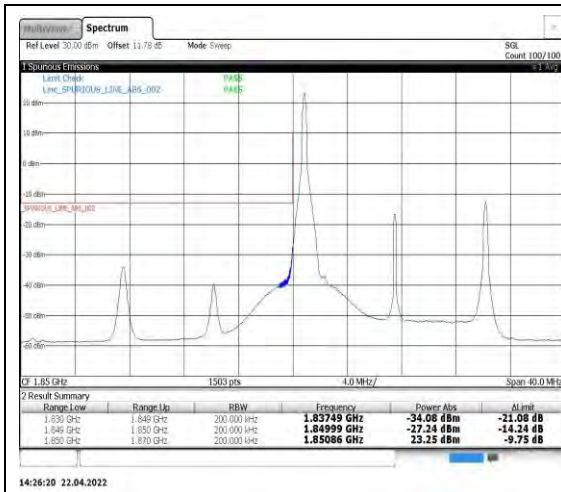
Band2-15MHz-16QAM-18675-1RB#0
