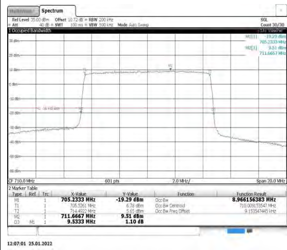
Band17-10MHz-16QAM-23790-50RB#0
