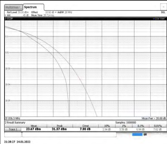
Band5-5MHz-16QAM-20525
