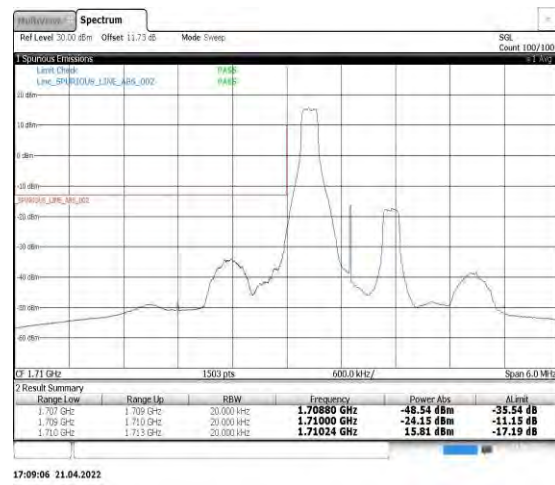
Band4-1.4MHz-QPSK-19957-1RB#0
