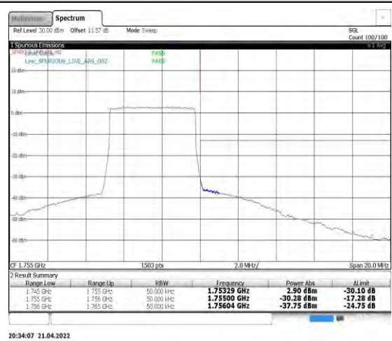
Band4-5MHz-16QAM-20375-25RB#0
