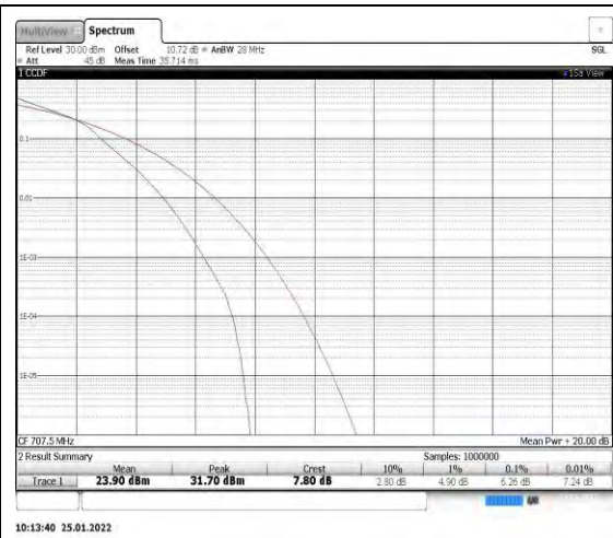
Band12-5MHz-16QAM-23095
