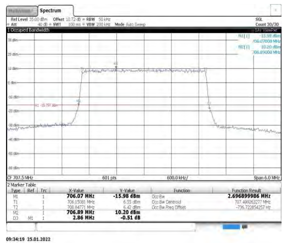
Band12-3MHz-16QAM-23095-15RB#0
