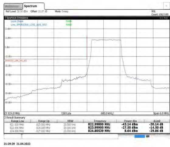
Band5-1.4MHz-QPSK-20407-6RB#0
