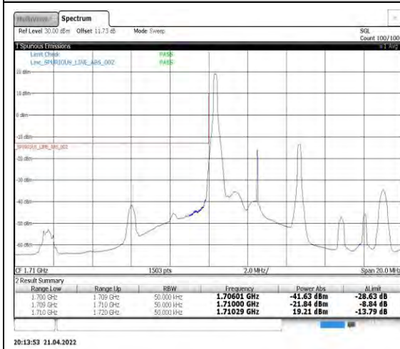
Band4-5MHz-QPSK-19975-1RB#0
