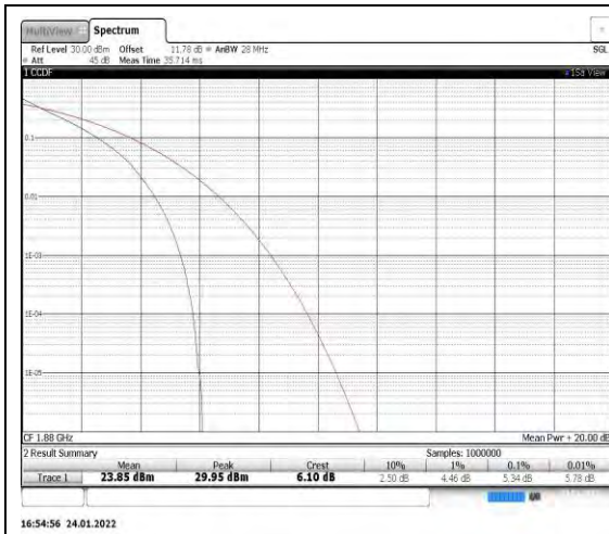
Band2-10MHz-QPSK-18900
