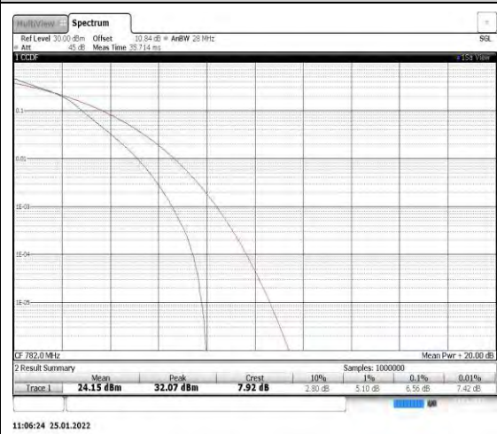
Band13-5MHz-16QAM-23230
