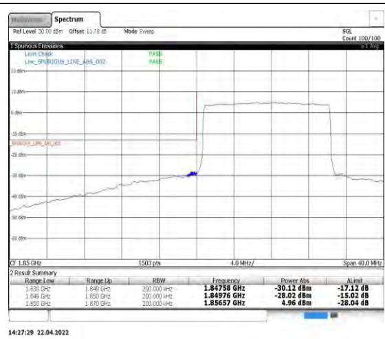
Band2-15MHz-16QAM-18675-75RB#0
