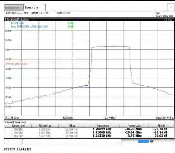
Band4-5MHz-16QAM-19975-25RB#0
