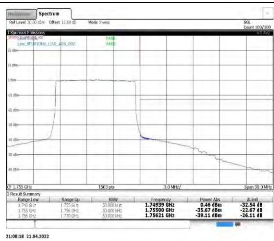
Band4-10MHz-16QAM-20350-50RB#0
