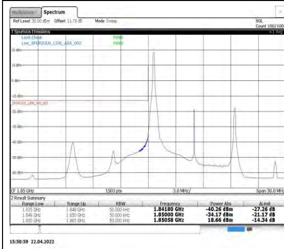
Band2-10MHz-16QAM-18650-1RB#0
