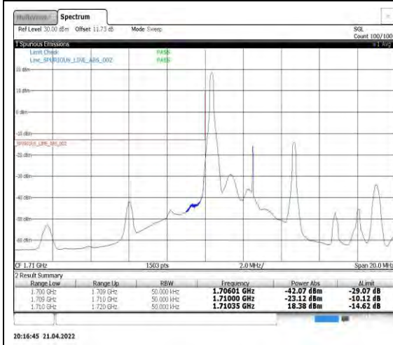
Band4-5MHz-16QAM-19975-1RB#0
