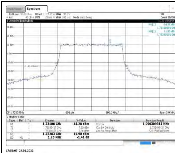
Band4-1.4MHz-QPSK-20175-6RB#0
