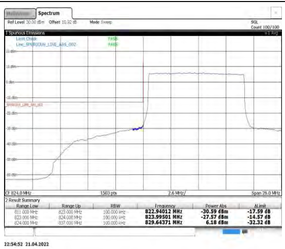
Band5-10MHz-QPSK-20450-50RB#0
