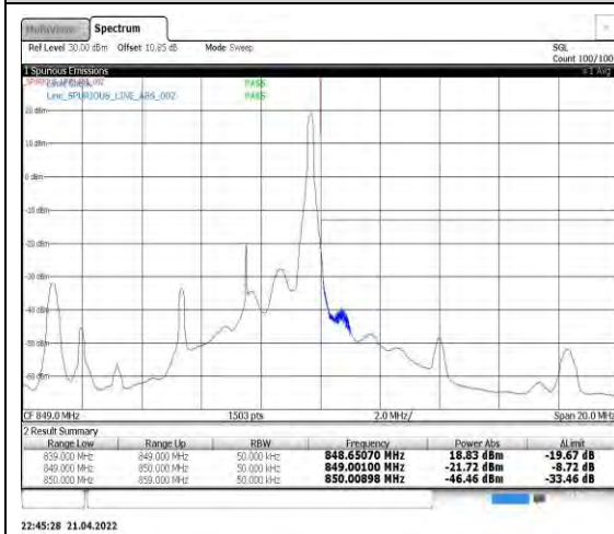
Band5-5MHz-16QAM-20625-1RB#24
