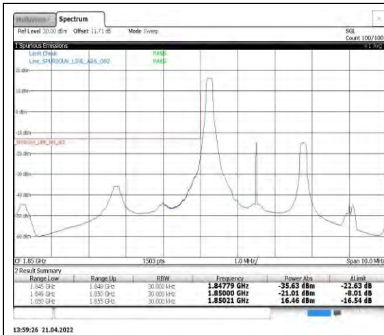
Band2-3MHz-16QAM-18615-1RB#0
