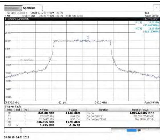
Band5-1.4MHz-16QAM-20525-6RB#0
