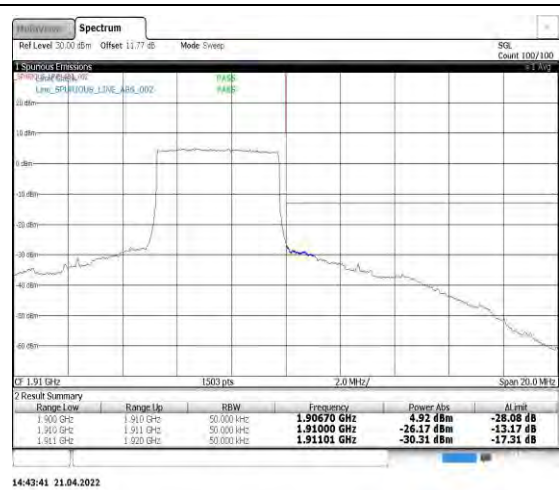
Band2-5MHz-QPSK-19175-25RB#0
