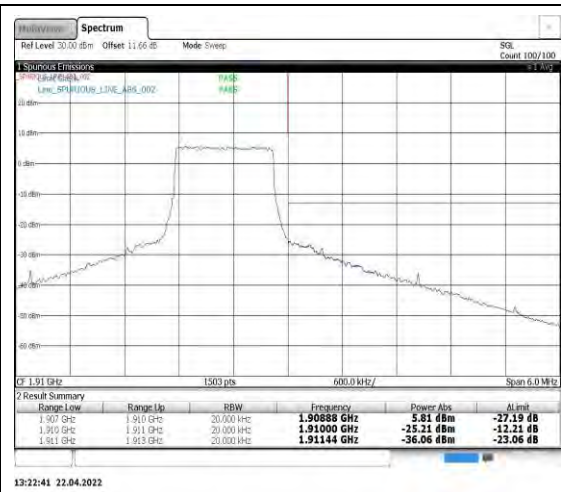
Band2-1.4MHz-16QAM-19193-6RB#0
