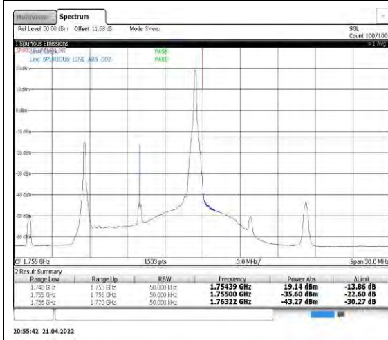
Band4-10MHz-QPSK-20350-1RB#49
