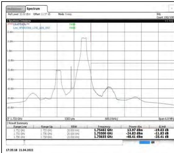
Band4-1.4MHz-16QAM-20393-1RB#5
