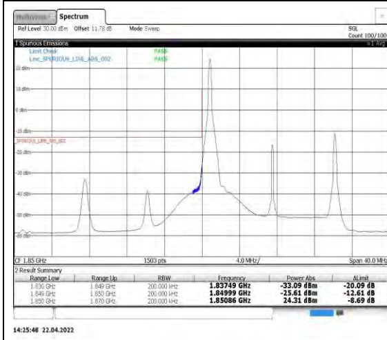
Band2-15MHz-QPSK-18675-1RB#0
