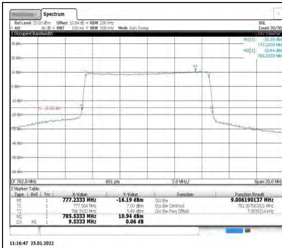
Band13-10MHz-QPSK-23230-50RB#0
