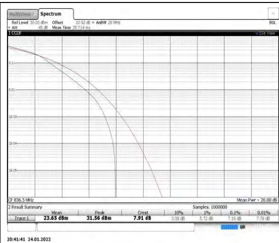
Band5-1.4MHz-16QAM-20525
