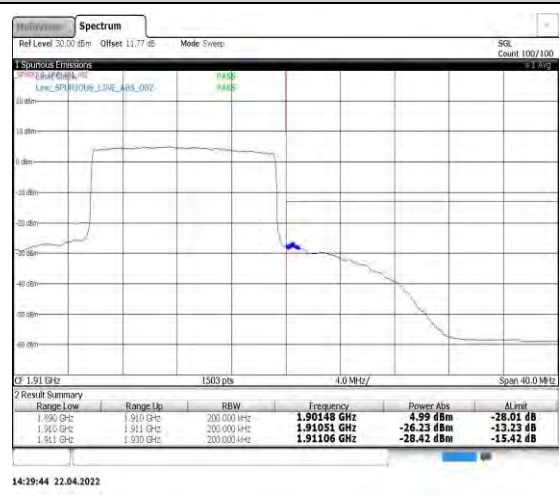
Band2-15MHz-16QAM-19125-75RB#0
