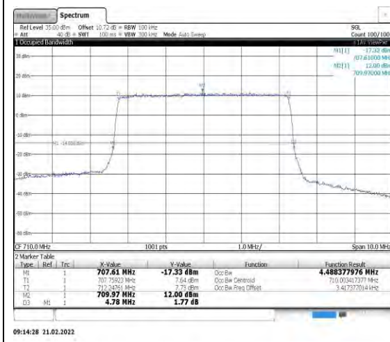
Band17-5MHz-QPSK-23790-25RB#0
