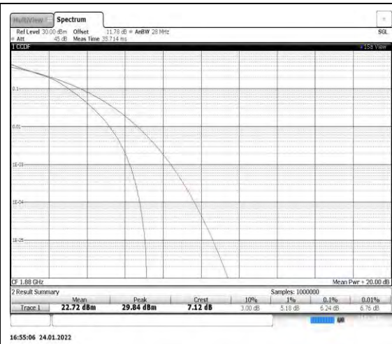
Band2-10MHz-16QAM-18900
