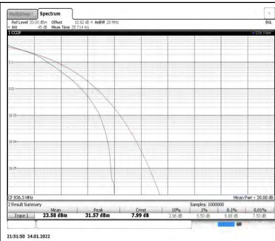
Band5-10MHz-16QAM-20525
