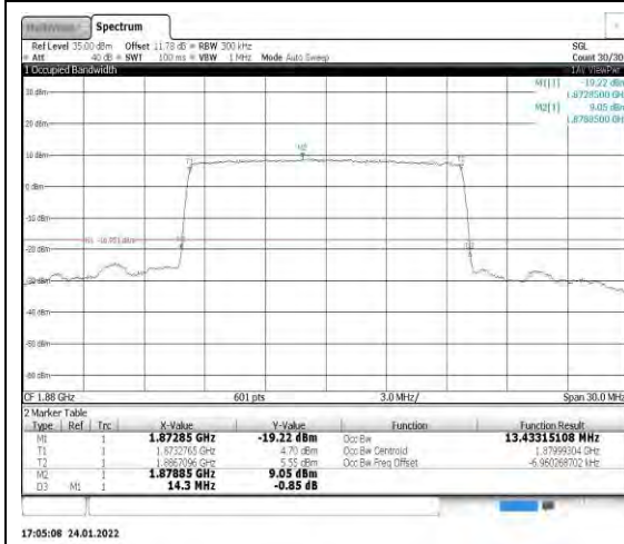
Band2-15MHz-QPSK-18900-75RB#0
