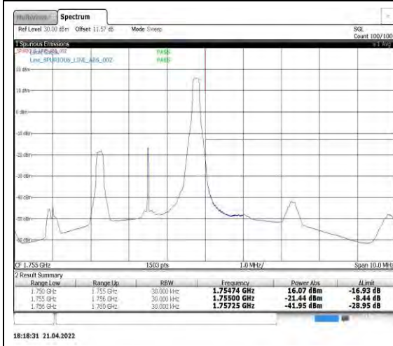
Band4-3MHz-16QAM-20385-1RB#14
