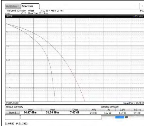
Band5-3MHz-QPSK-20525
