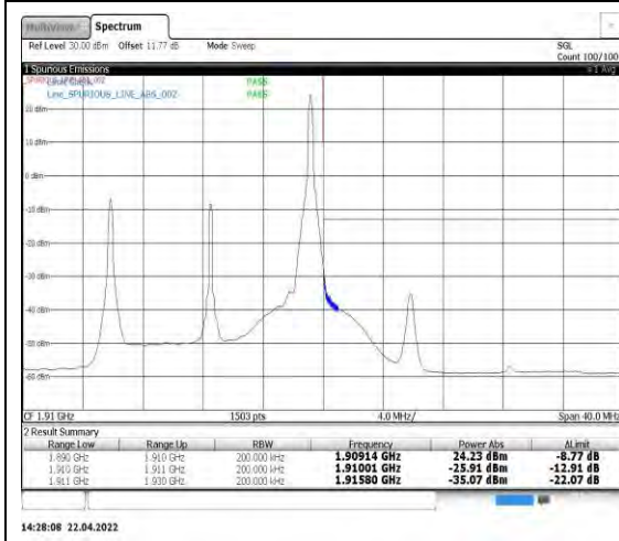
Band2-15MHz-QPSK-19125-1RB#74
