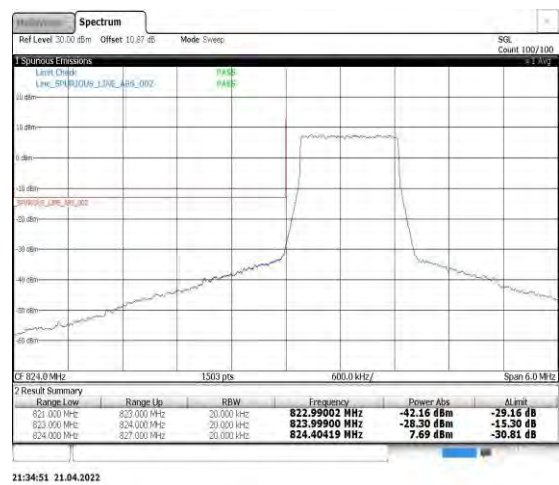
Band5-1.4MHz-16QAM-20407-6RB#0
