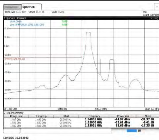
Band2-1.4MHz-QPSK-18607-1RB#0
