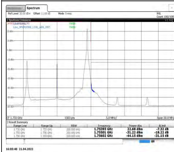
Band4-20MHz-16QAM-20300-1RB#99
