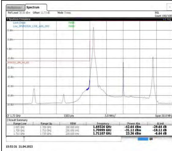
Band4-20MHz-16QAM-20050-1RB#0
