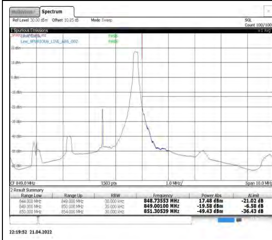
Band5-3MHz-16QAM-20635-1RB#14
