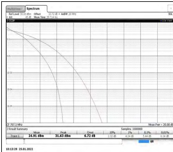
Band12-5MHz-QPSK-23095
