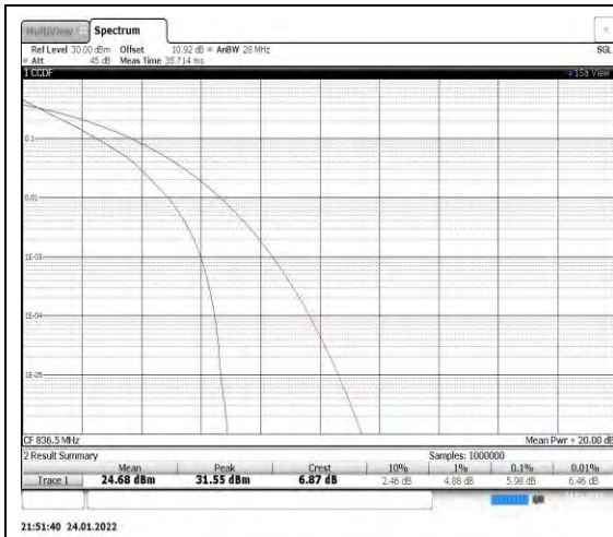
Band5-10MHz-QPSK-20525
