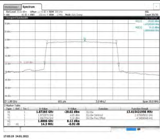
Band2-15MHz-16QAM-18900-75RB#0
