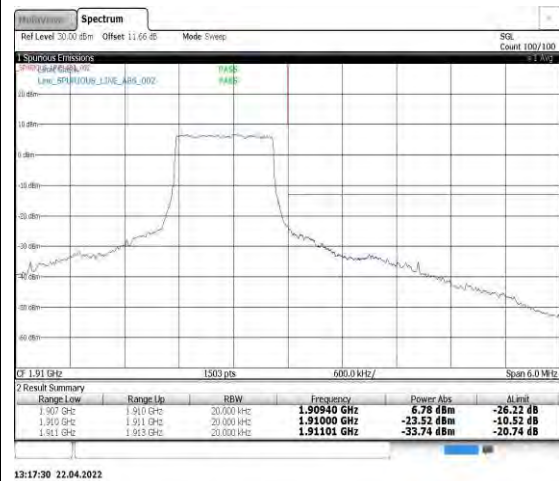
Band2-1.4MHz-QPSK-19193-6RB#0
