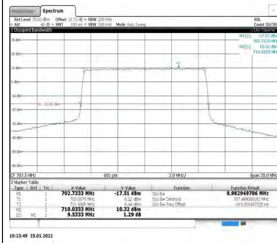
Band12-10MHz-QPSK-23095-50RB#0
