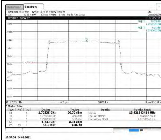
Band4-15MHz-QPSK-20175-75RB#0
