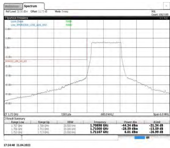
Band4-1.4MHz-16QAM-19957-6RB#0
