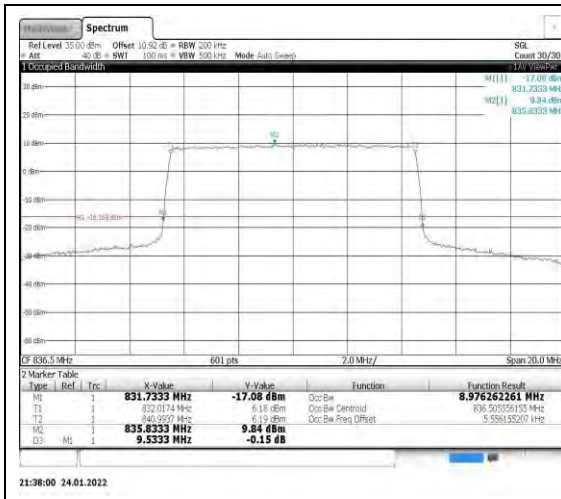
Band5-10MHz-QPSK-20525-50RB#0
