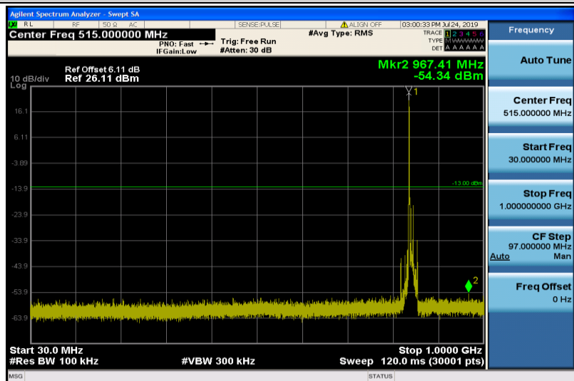
Band5-10MHz-QPSK-20600-1RB#0-30~1000MHz
