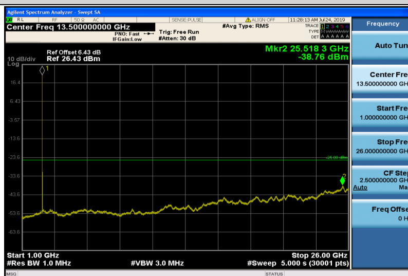
Band7-10MHz-QPSK-21400-1RB#0-1000~26000MHz
