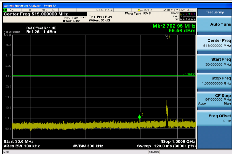
Band5-1.4MHz-16QAM-20643-1RB#0-30~1000MHz
