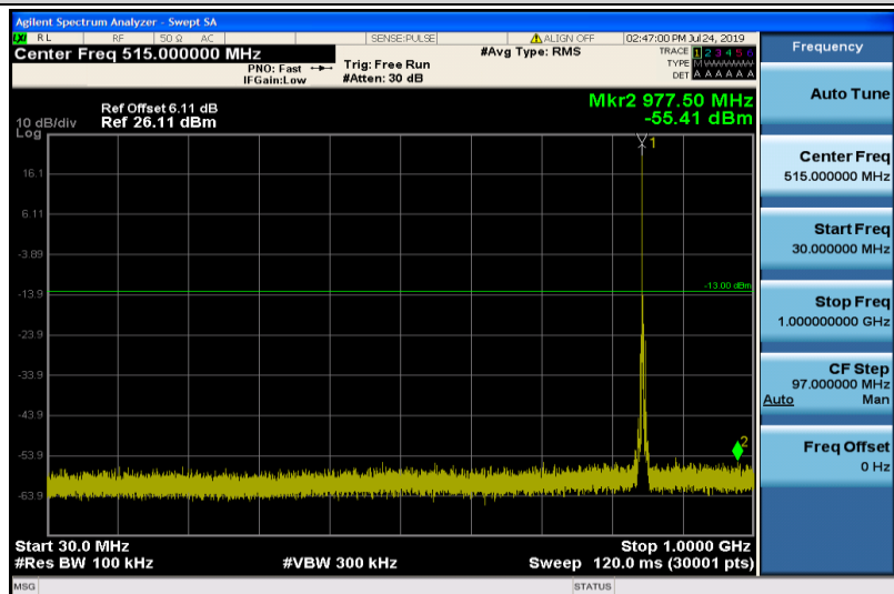
Band5-3MHz-16QAM-20635-1RB#0-30~1000MHz
