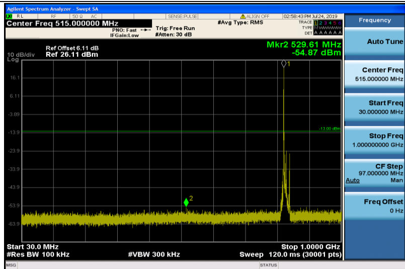
Band5-10MHz-16QAM-20450-1RB#0-30~1000MHz
