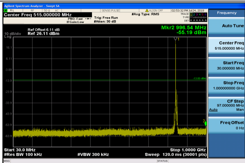
Band5-5MHz-QPSK-20625-1RB#0-30~1000MHz
