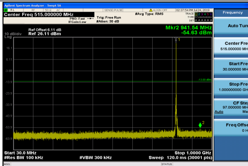
Band5-1.4MHz-QPSK-20407-1RB#0-30~1000MHz
