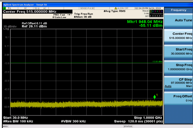
Band4-20MHz-16QAM-20300-1RB#0-30~1000MHz
