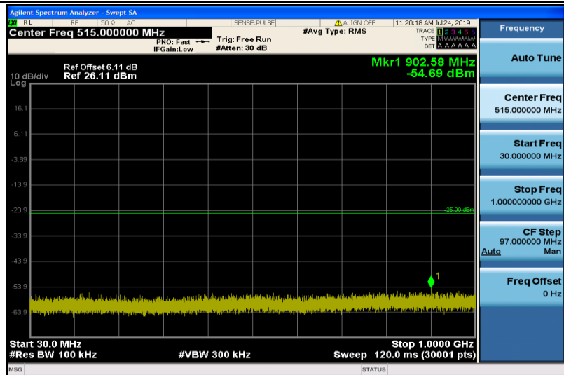
Band7-5MHz-16QAM-20775-1RB#0-30~1000MHz
