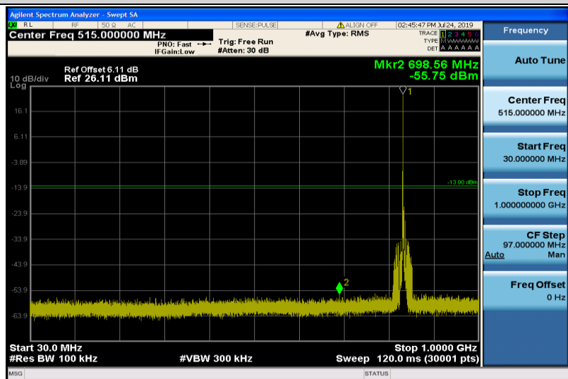
Band5-3MHz-16QAM-20525-1RB#0-30~1000MHz
