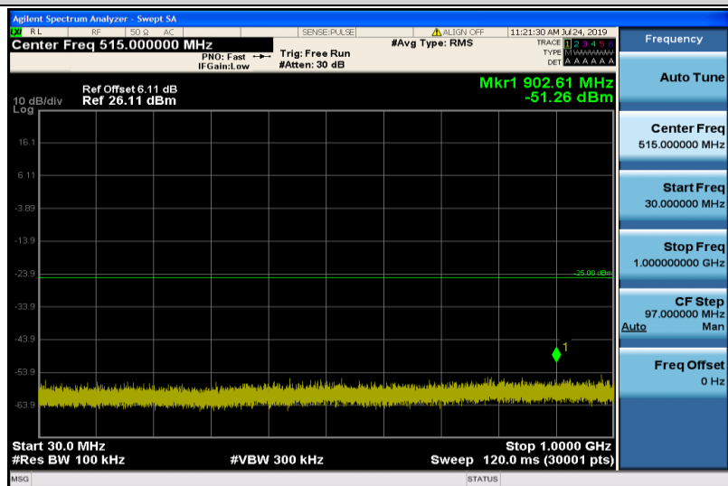
Band7-5MHz-16QAM-21100-1RB#0-30~1000MHz
