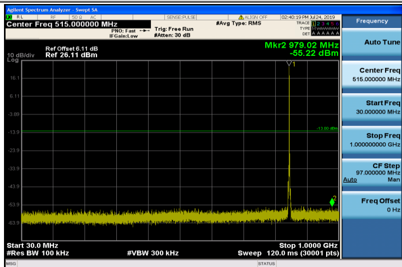
Band5-1.4MHz-QPSK-20643-1RB#0-30~1000MHz
