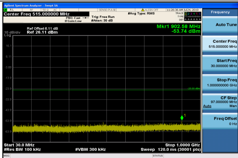
Band7-10MHz-QPSK-21100-1RB#0-30~1000MHz
