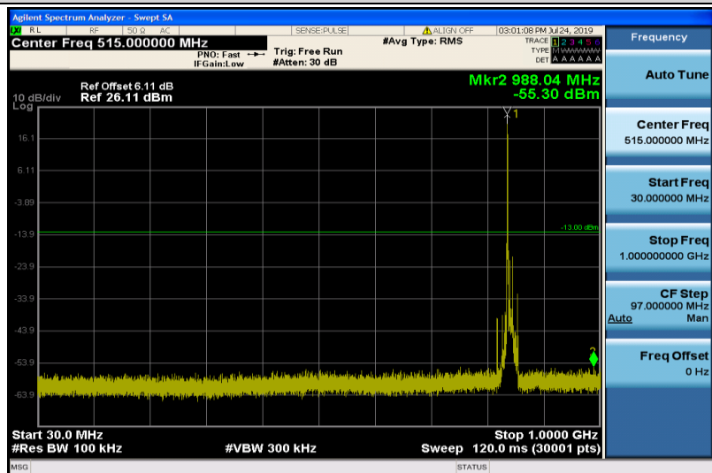
Band5-10MHz-16QAM-20600-1RB#0-30~1000MHz
