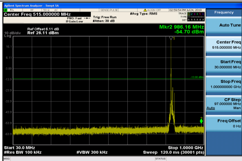
Band5-10MHz-16QAM-20525-1RB#0-30~1000MHz
