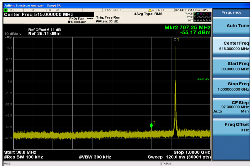
Band5-3MHz-16QAM-20415-1RB#0-30~1000MHz
