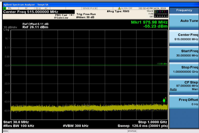
Band4-20MHz-QPSK-20175-1RB#0-30~1000MHz
