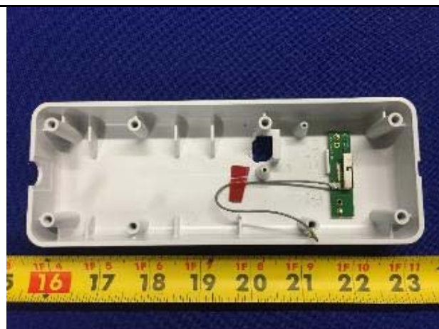
Antenna Inside EUT View
