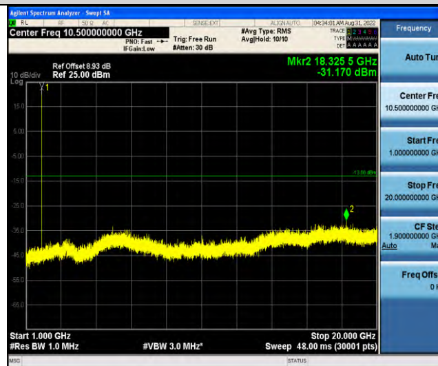
Band25-Stand-Alone-NaN-BPSK-26042-1@0-15kHz-1000-20000-1000~20000MHz@-31.17dBm--13-PASS
