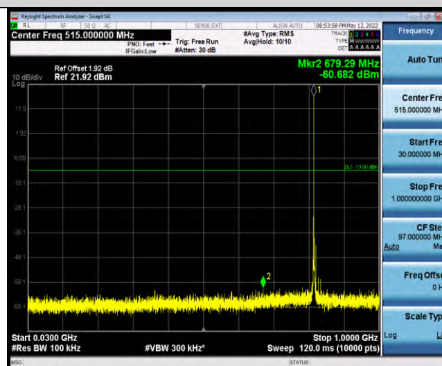
Band26-Stand-Alone-NaN-BPSK-26740-1@11-15kHz-30-1000-30~1000MHz@-60.68dBm--13-PASS
