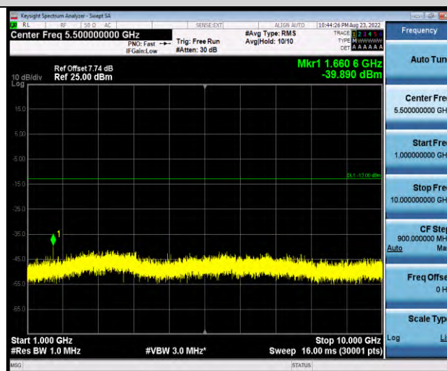
Band19-Stand-Alone-Na-N-QPSK-24002-12@0-15kHz-1000-10000-1000~10000MHz@-39.89dBm--13-PASS
