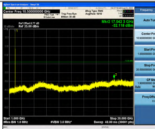
Band25-Stand-Alone-NaN-BPSK-26688-1@11-15kHz-1000-20000-1000~20000MHz@-32.12dBm--13-PASS
