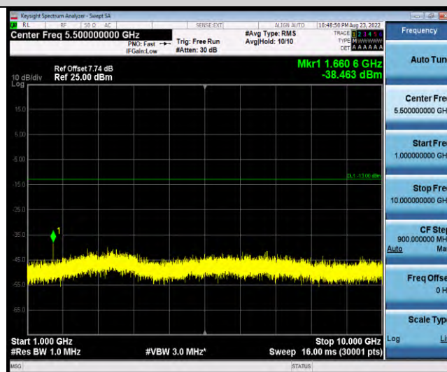
Band19-Stand-Alone-NaN-BPSK-24002-1@11-15kHz-1000-10000-1000~10000MHz@-38.46dBm--13-PASS
