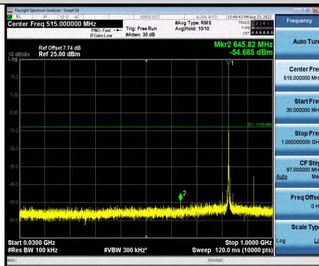
Band19-Stand-Alone-NaN-BPSK-24002-1@11-15kHz-30-1000-30~1000MHz@-54.69dBm--13-PASS
