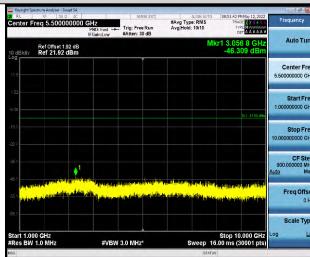
Band26-Stand-Alone-NaN-BPSK-26692-1@11-15kHz-1000-10000-1000~10000MHz@-46.31dBm--13-PASS
