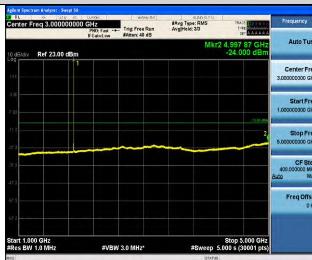
Band25-Stand-Alone-NaN-QPSK-26365-1@47-3.75kHz-1000-5000-1000~5000MHz@-24dBm--13-PASS
