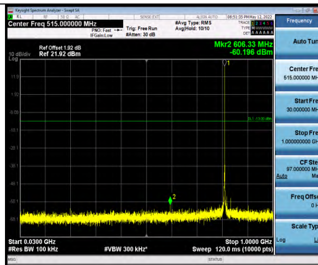
Band26-Stand-Alone-NaN-BPSK-26692-1@11-15kHz-30-1000-30~1000MHz@-60.2dBm--13-PASS
