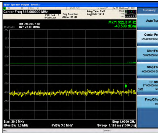
Band25-Stand-Alone-NaN-BPSK-26688-1@11-15kHz-30-1000-30~1000MHz@-40.6dBm--13-PASS
