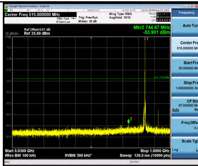
Band19-Stand-Alone-Na-N-BPSK-24148-1@11-15kHz-30-1000-30~1000MHz@-53.9dBm--13-PASS
