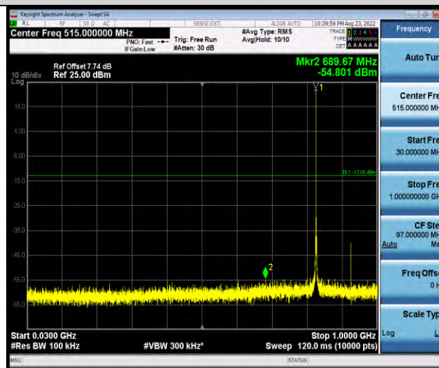
Band19-Stand-Alone-Na-N-QPSK-24002-1@47-3.75kHz-30-1000-30~1000MHz@-54.8dBm--13-PASS
