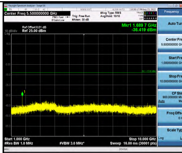
Band19-Stand-Alone-Na-N-BPSK-24148-1@0-15kHz-1000-10000-1000~10000MHz@-36.42dBm--13-PASS
