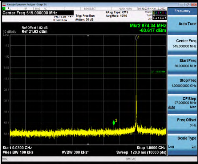
Band26-Stand-Alone-NaN-BPSK-26692-1@0-15kHz-30-1000-30~1000MHz@-60.62dBm--13-PASS
