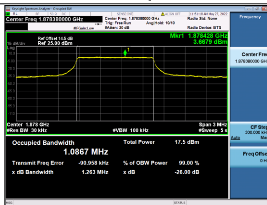
B2-5M-Mid CH-OBW-QPSK
