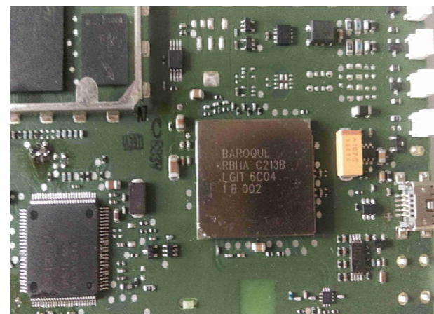
FLEXCM-WLAN and BT Module
