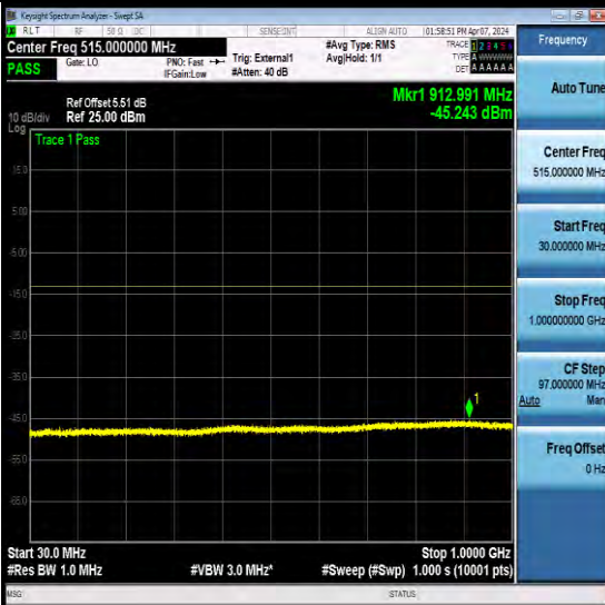
NTN-N78-3450-3550-PC2-30-60-M-CP-QPSK-Edge_1RB_ Left-Ant3-PASS
