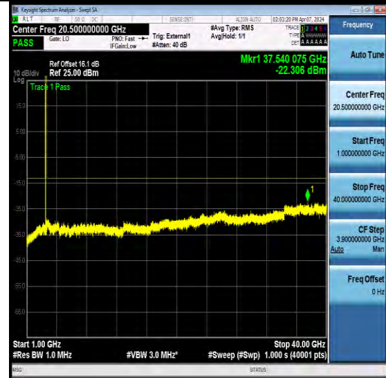
NTNV-N78-3450-3550-PC2-30-100-M-CP-QPSK-Edge_1RB_1RB Left-Ant3-PASS
