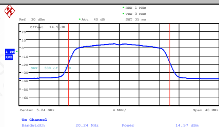
11AC20MIMO-Ant1-5240-PASS
