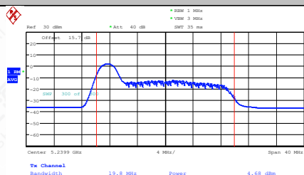
11AX20MIMO-Ant1-5240-26Tone-RU0-PASS
