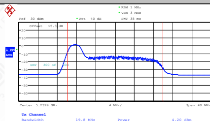
11AX20MIMO-Ant2-5240-26Tone-RU0-PASS
