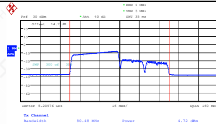
11AX80SISO-Ant2-5210-484Tone-RU65-PASS
