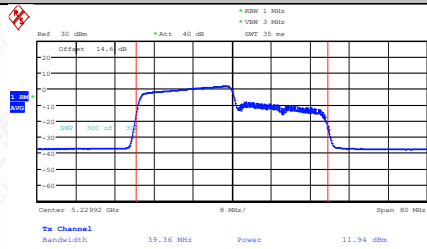
11AX40MIMO-Ant1-5230-242Tone-RU61-PASS
