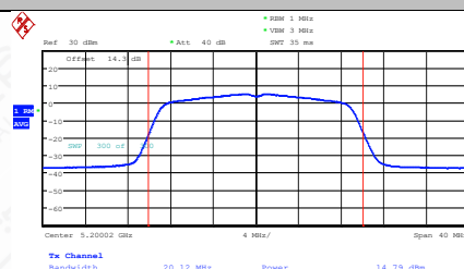
11AC20MIMO-Ant2-5200-PASS
