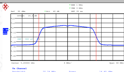
11AC20MIMO-Ant1-5200-PASS
