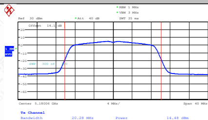
11AC20MIMO-Ant1-5180-PASS
