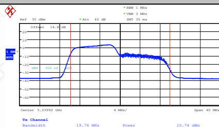
11AX20MIMO-Ant2-5240-106Tone-RU53-PASS
