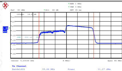
11AX40MIMO-Ant1-5230-242Tone-RU62-PASS
