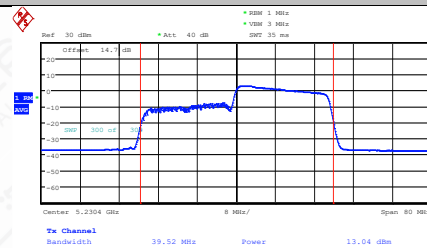
11AX40MIMO-Ant2-5230-242Tone-RU62-PASS
