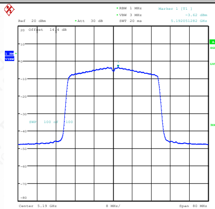
11AC40MIMO-Ant1-5190-PASS
