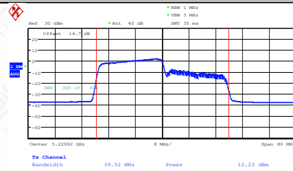
11AX40MIMO-Ant2-5230-242Tone-RU61-PASS
