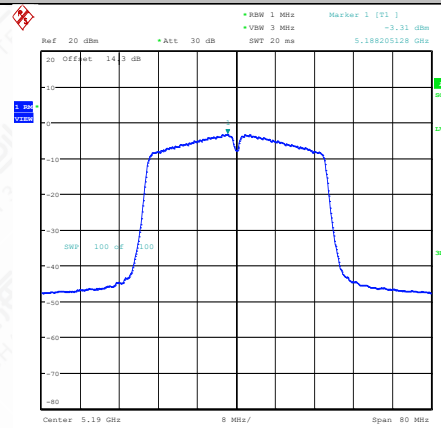
11AC40SISO-Ant2-5190-PASS
