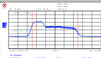
11AX20MIMO-Ant1-5240-52Tone-RU37-PASS
