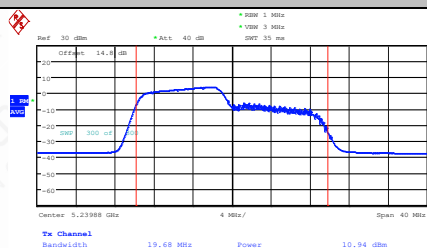
11AX20MIMO-Ant1-5240-106Tone-RU53-PASS
