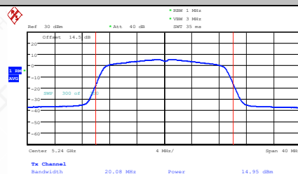
11AC20MIMO-Ant2-5240-PASS
