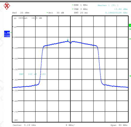
11AC40MIMO-Ant2-5190-PASS
