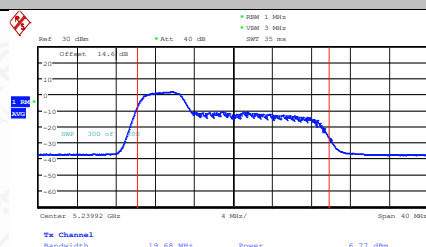
11AX20MIMO-Ant2-5240-52Tone-RU37-PASS
