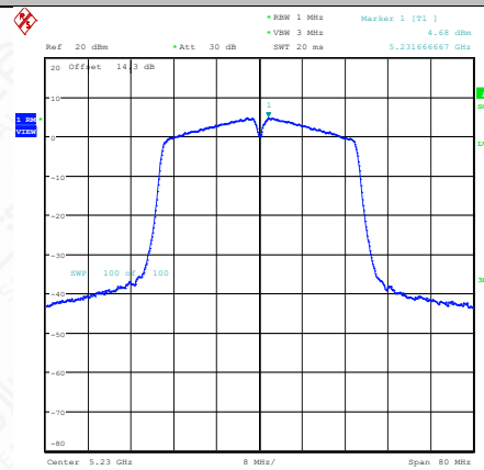
11AC40SISO-Ant2-5230-PASS
