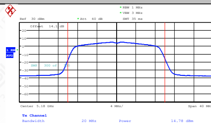
11AC20MIMO-Ant2-5180-PASS
