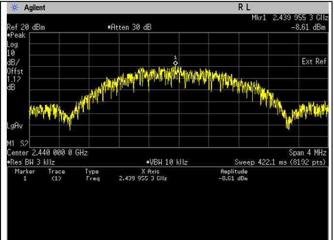
Maximum Power Spectral Density. Bluetooth LE Frequency 2440 MHz
