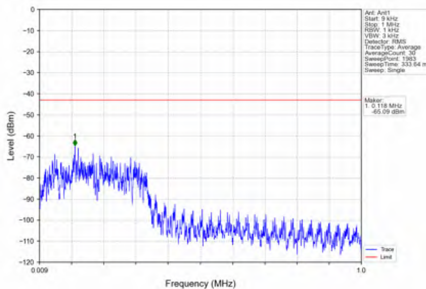
n7_30kHz_SISO_NTNV_10MHz_DFT-s-OFDM QPSK_2505MHz_Edge_1RB_Left
