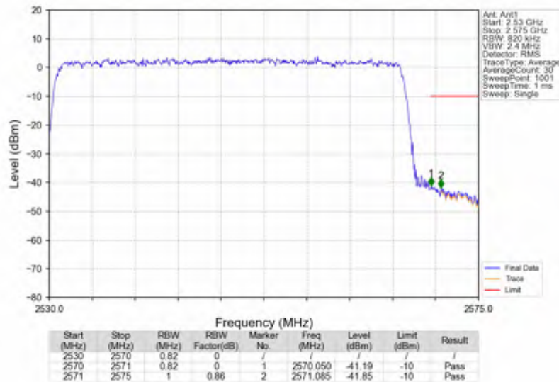
n7_30kHz_SISO_NTNV_40MHz_DFT-s-OFDM PI/2 BPSK_2550MHz_Outer_Full
