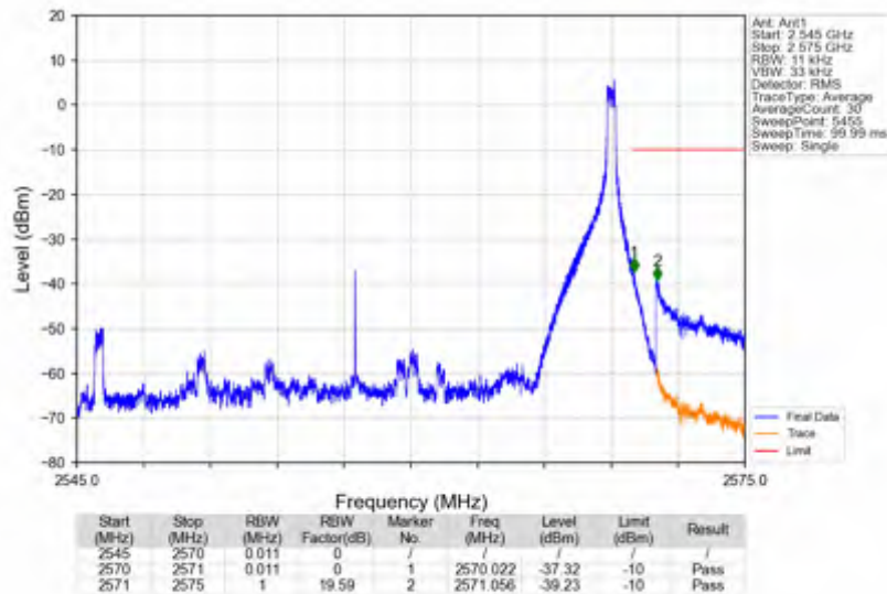
n7_30kHz_SISO_NTNV_25MHz_DFT-s-OFDM QPSK_2557.5MHz_Edge_1RB_Right
