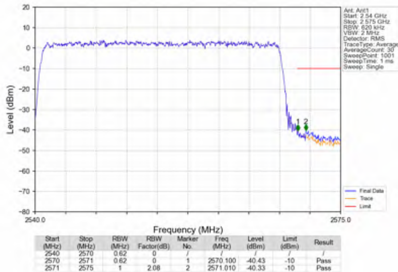
n7_30kHz_SISO_NTNV_30MHz_DFT-s-OFDM PI/2 BPSK_2555MHz_Outer_Full
