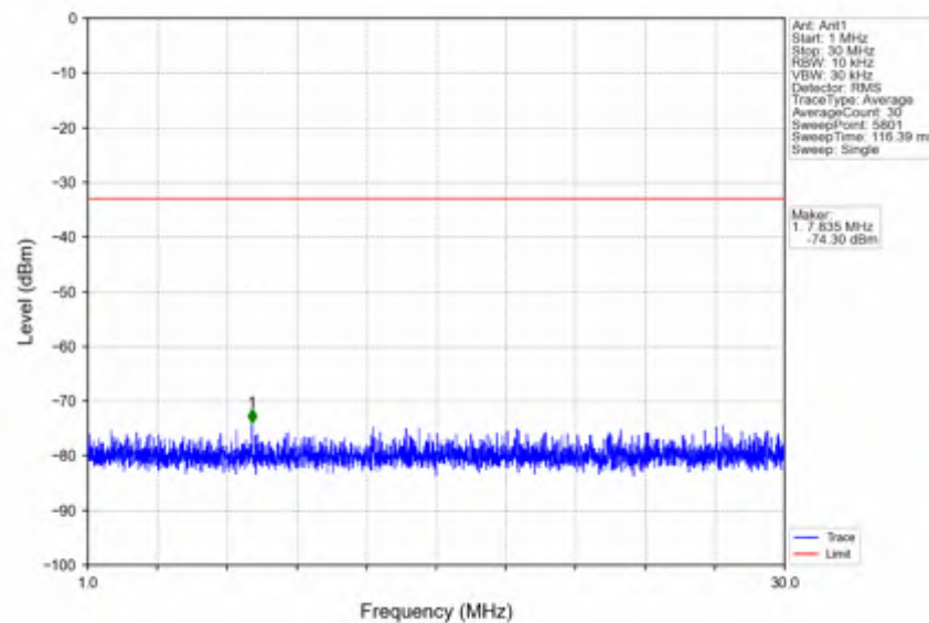
n7_30kHz_SISO_NTNV_20MHz_DFT-s-OFDM QPSK_2535MHz_Edge_1RB_Left
