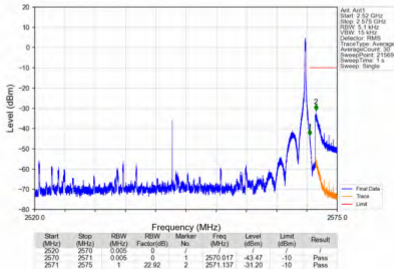
n7_15kHz_SISO_NTNV_50MHz_DFT-s-OFDM QPSK_2545MHz_Edge_1RB_Right
