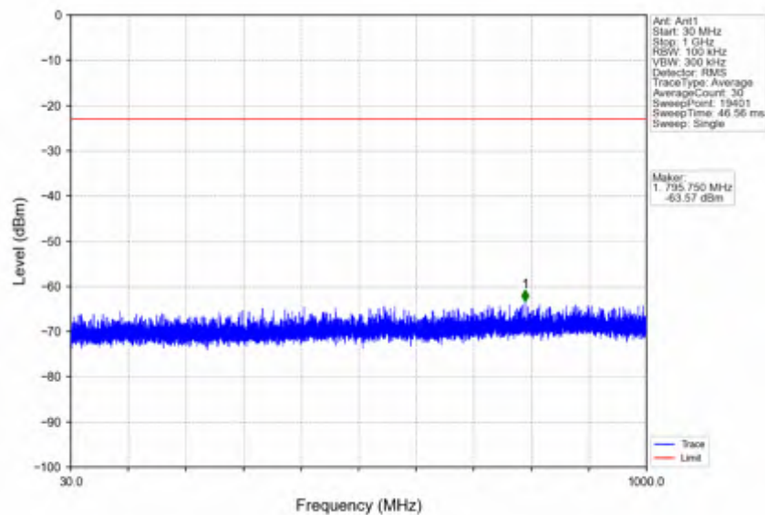
n7_30kHz_SISO_NTNV_30MHz_CP-OFDM QPSK_2535MHz_Edge_1RB_Left
