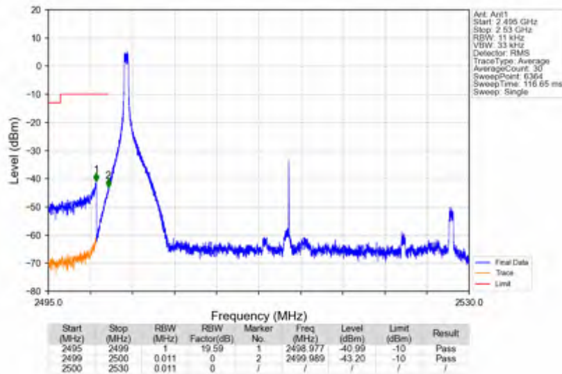
n7_30kHz_SISO_NTNV_30MHz_DFT-s-OFDM QPSK_2515MHz_Inner_1RB_Left
