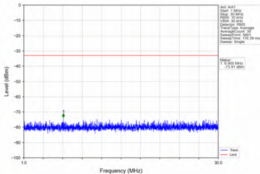
n7_30kHz_SISO_NTNV_10MHz_DFT-s-OFDM PI/2 BPSK_2505MHz_Edge_1RB_Left
