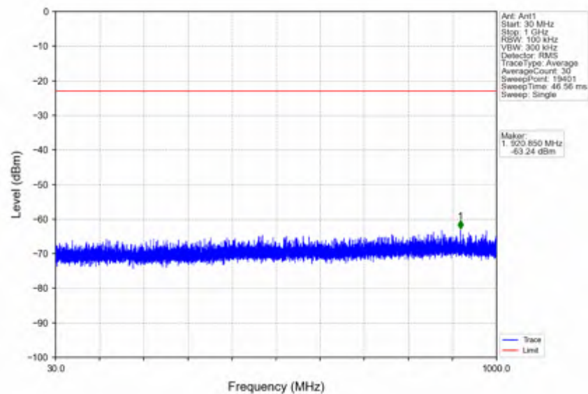
n7_30kHz_SISO_NTNV_20MHz_DFT-s-OFDM_PI/2_BPSK_2560MHz_Edge_1RB_Right
