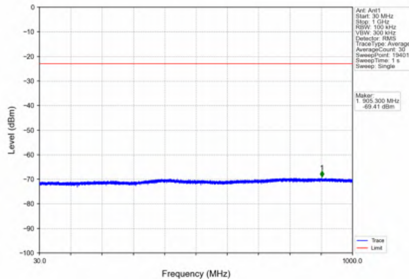
n7_15kHz_SISO_NTNV_50MHz_DFT-s-OFDM QPSK_2535MHz_Edge_1RB_Left
