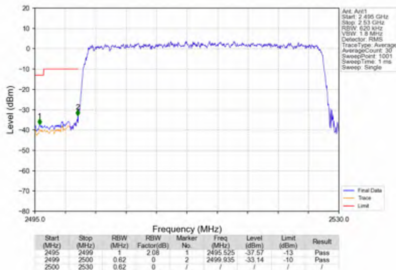
n7_30kHz_SISO_NTNV_30MHz_DFT-s-OFDM QPSK_2515MHz_Outer_Full
