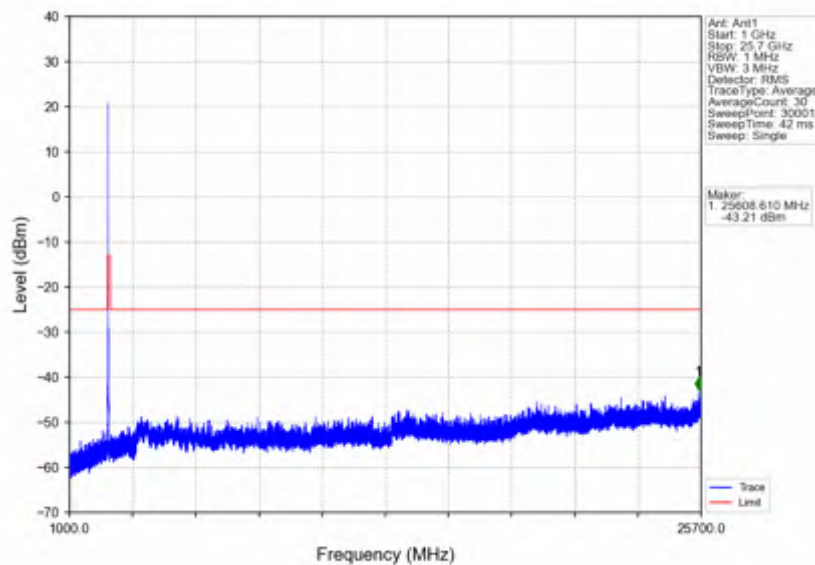
n7_30kHz_SISO_NTNV_20MHz_DFT-s-OFDM QPSK_2510MHz_Outer_Full
