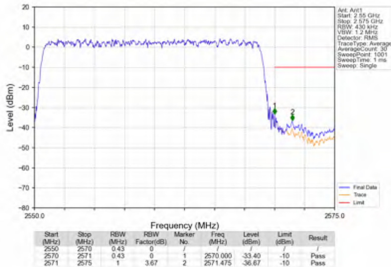
n7_30kHz_SISO_NTNV_20MHz_DFT-s-OFDM PI/2 BPSK_2560MHz_Outer_Full
