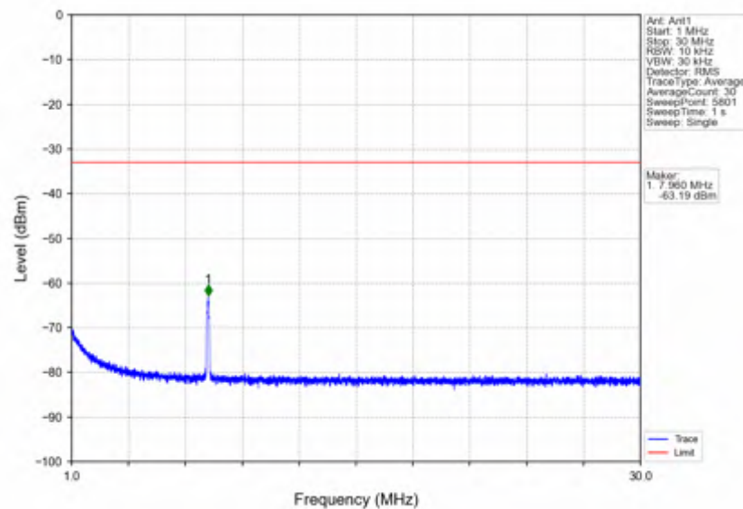
n7_15kHz_SISO_NTNV_50MHz_CP-OFDM_QPSK_2545MHz_Edge_1RB_Right
