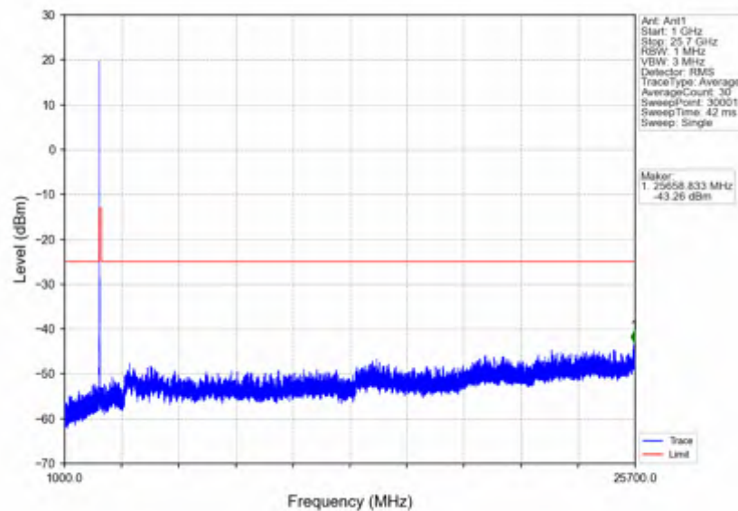
n7_30kHz_SISO_NTNV_15MHz_CP-OFDM QPSK_2507.5MHz_Outer_Full
