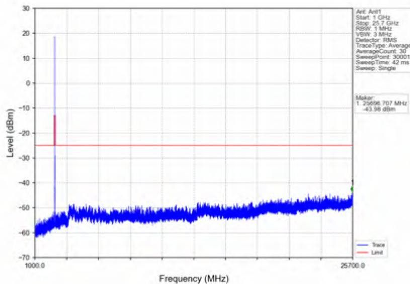
n7_30kHz_SISO_NTNV_15MHz_CP-OFDM QPSK_2562.5MHz_Edge_1RB_Right
