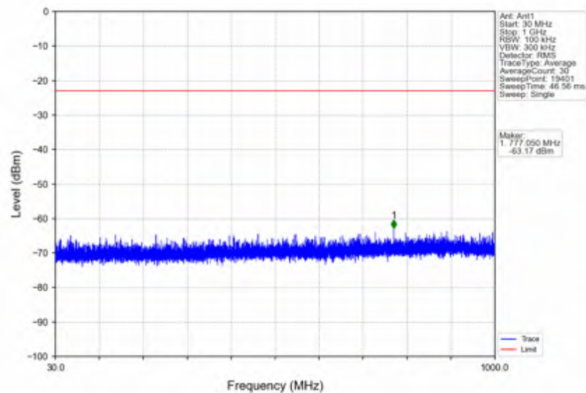
n7_30kHz_SISO_NTNV_20MHz_DFT-s-OFDM_QPSK_2560MHz_Edge_1RB_Right
