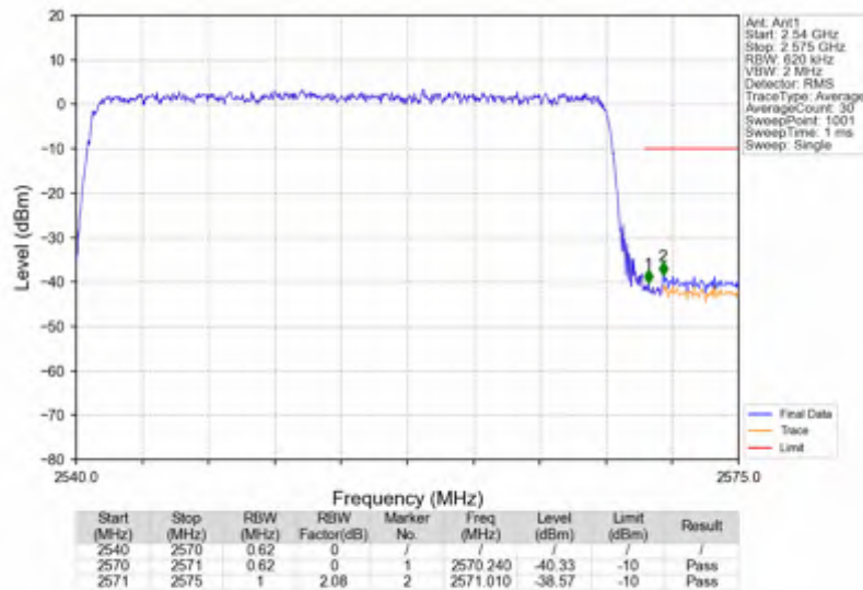
n7_30kHz_SISO_NTNV_30MHz_DFT-s-OFDM_QPSK_2555MHz_Outer_Full
