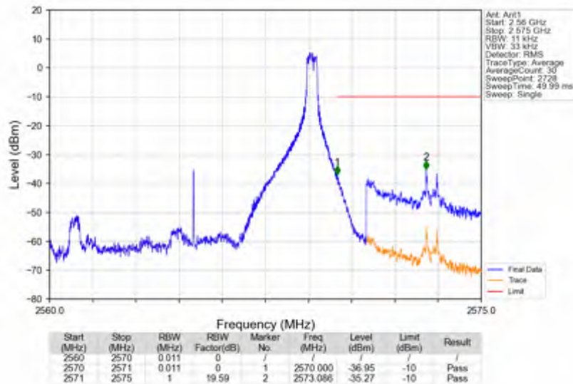
n7_30kHz_SISO_NTNV_10MHz_DFT-s-OFDM PI/2 BPSK_2565MHz_Edge_1RB_Right
