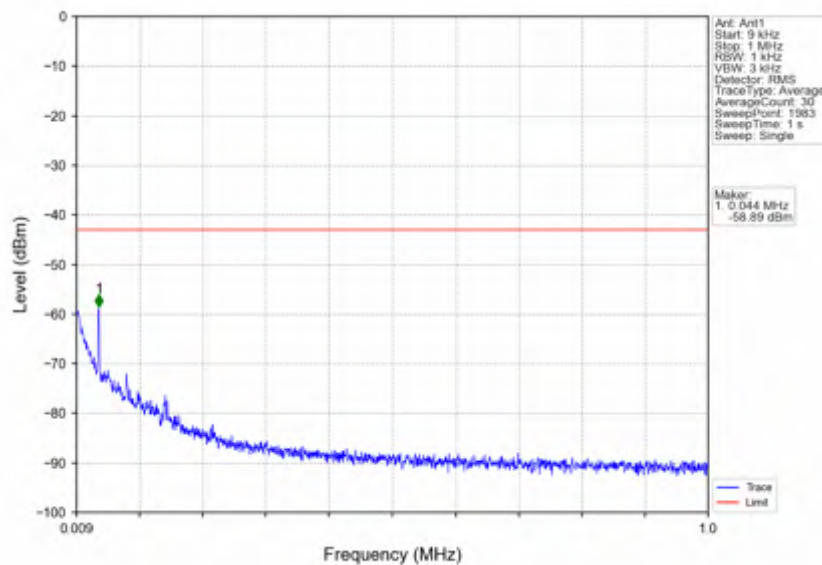
n7_15kHz_SISO_NTNV_50MHz_DFT-s-OFDM QPSK_2545MHz_Edge_1RB_Right
