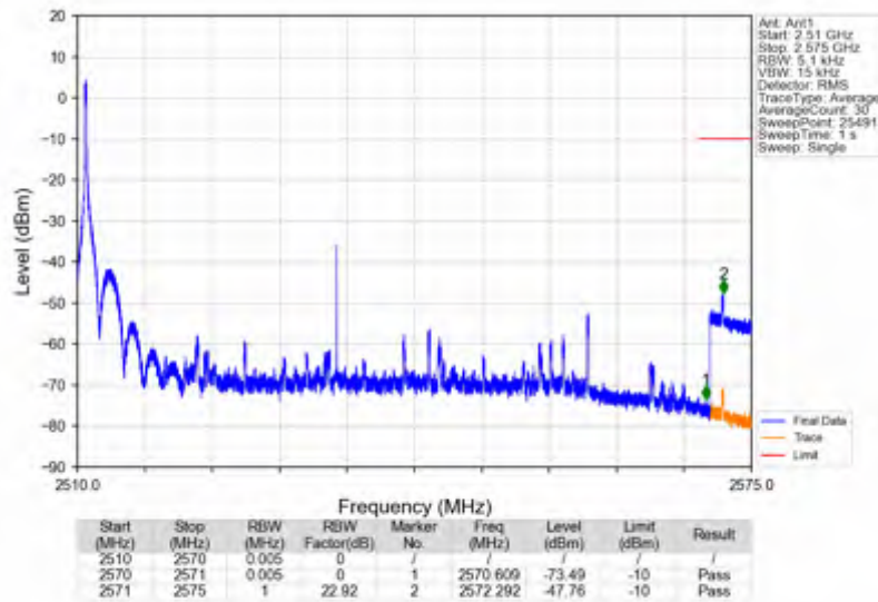
n7_15kHz_SISO_NTNV_50MHz_DFT-s-OFDM_QPSK_2535MHz_Edge_1RB_Left
