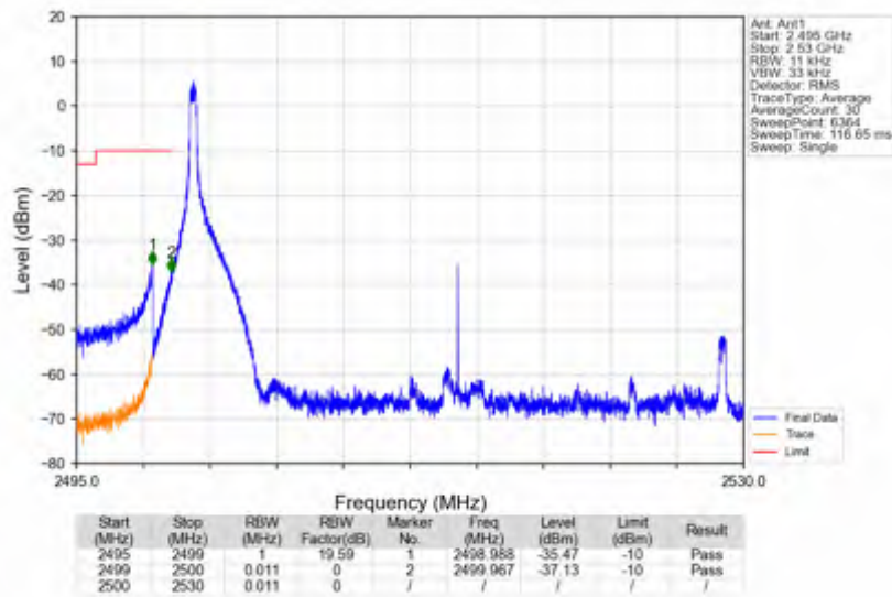
n7_30kHz_SISO_NTNV_30MHz_DFT-s-OFDM_PI/2_BPSK_2515MHz_Edge_1RB_Left
