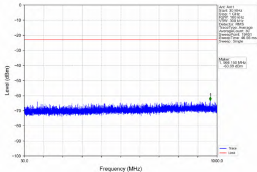
n7_30kHz_SISO_NTNV_10MHz_CP-OFDM QPSK_2565MHz_Edge_1RB_Right
