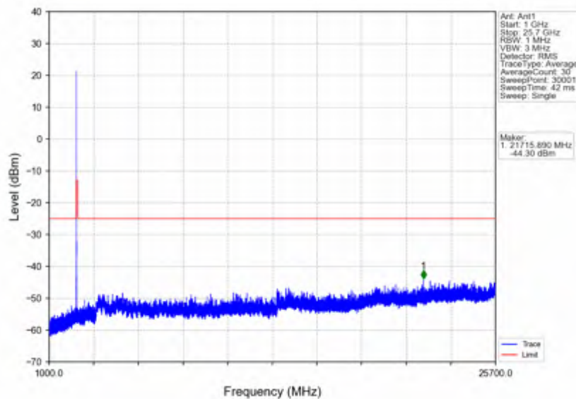
n7_30kHz_SISO_NTNV_10MHz_DFT-s-OFDM QPSK_2505MHz_Outer_Full
