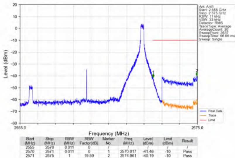
n7_30kHz_SISO_NTNV_15MHz_CP-OFDM QPSK_2562.5MHz_Inner_1RB_Right
