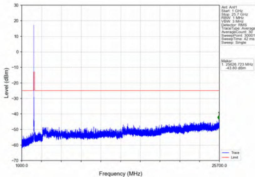
n7_30kHz_SISO_NTNV_30MHz_CP-OFDM QPSK_2515MHz_Outer_Full
