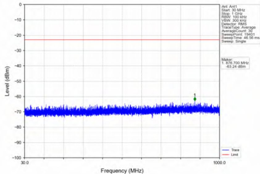
n7_30kHz_SISO_NTNV_40MHz_DFT-s-OFDM QPSK_2520MHz_Edge_1RB_Left
