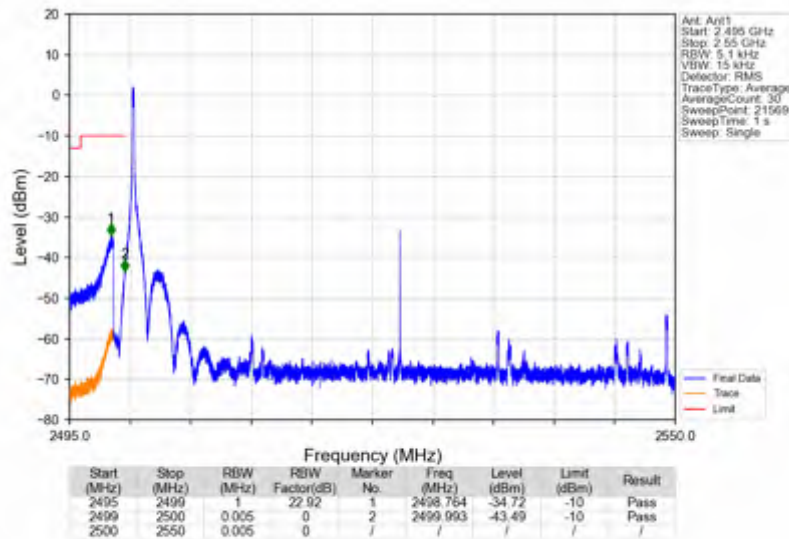
n7_15kHz_SISO_NTNV_50MHz_CP-OFDM QPSK_2525MHz_Edge_1RB_Left
