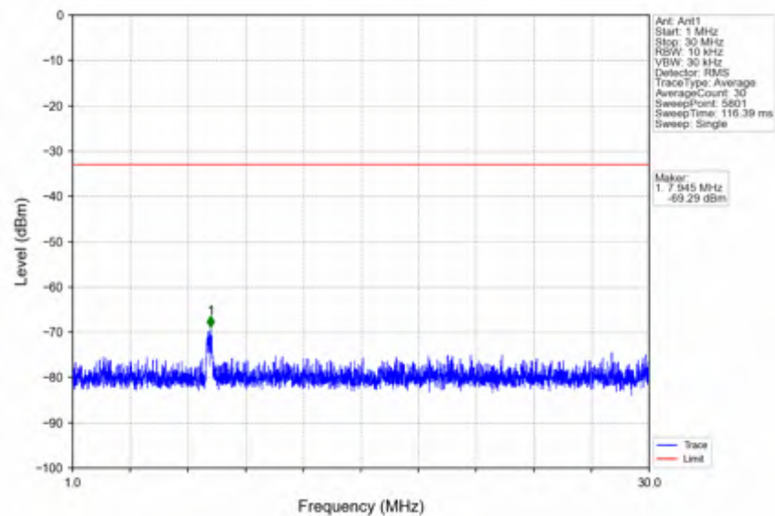
n7_30kHz_SISO_NTNV_15MHz_DFT-s-OFDM_QPSK_2562.5MHz_Edge_1RB_Right
