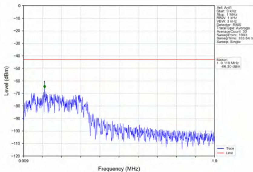
n7_30kHz_SISO_NTNV_25MHz_DFT-s-OFDM_QPSK_2535MHz_Edge_1RB_Left
