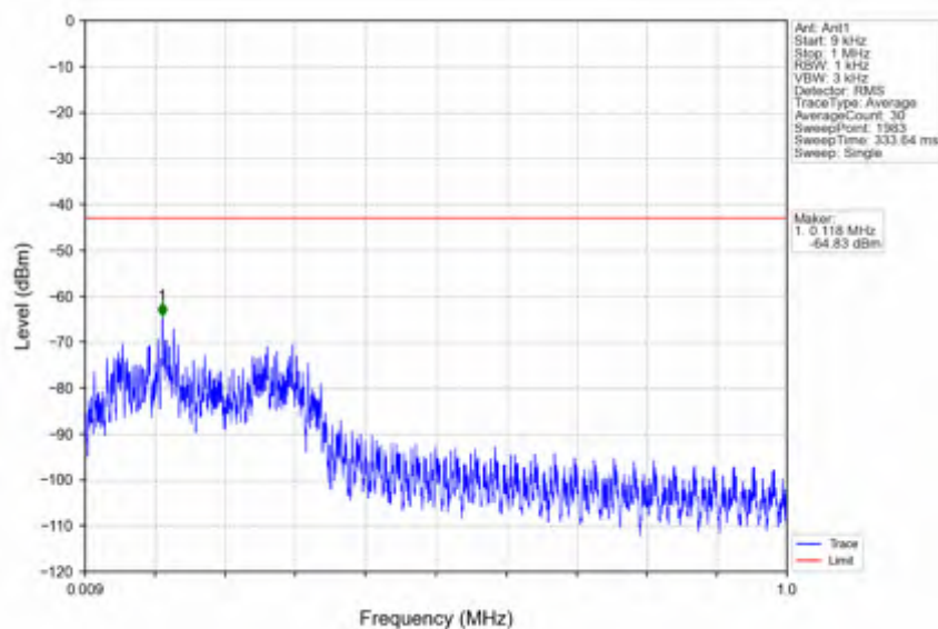
n7_30kHz_SISO_NTNV_15MHz_DFT-s-OFDM_PI/2_BPSK_2507.5MHz_Edge_1RB_Left
