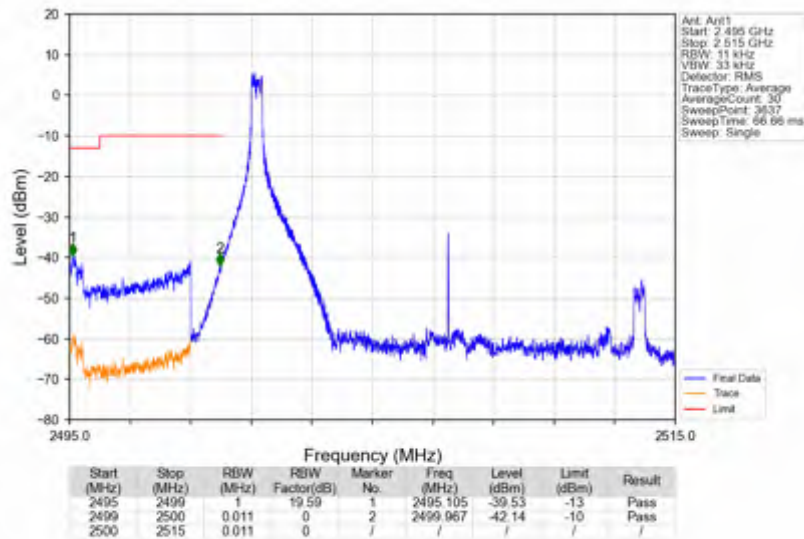
n7_30kHz_SISO_NTNV_15MHz_DFT-s-OFDM QPSK_2507.5MHz_Inner_1RB_Left
