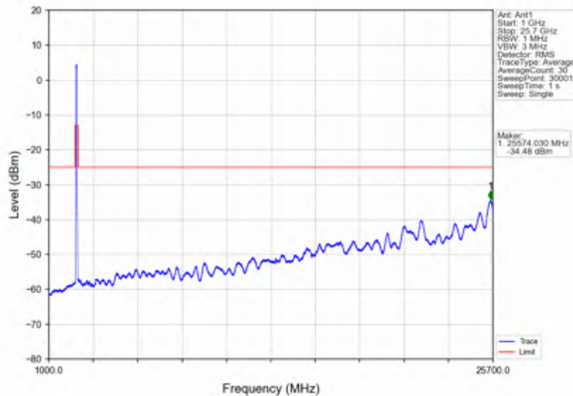
n7_15kHz_SISO_NTNV_50MHz_CP-OFDM_QPSK_2525MHz_Outer_Full
