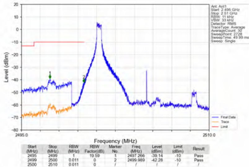
n7_30kHz_SISO_NTNV_10MHz_DFT-s-OFDM_QPSK_2505MHz_Inner_1RB_Left
