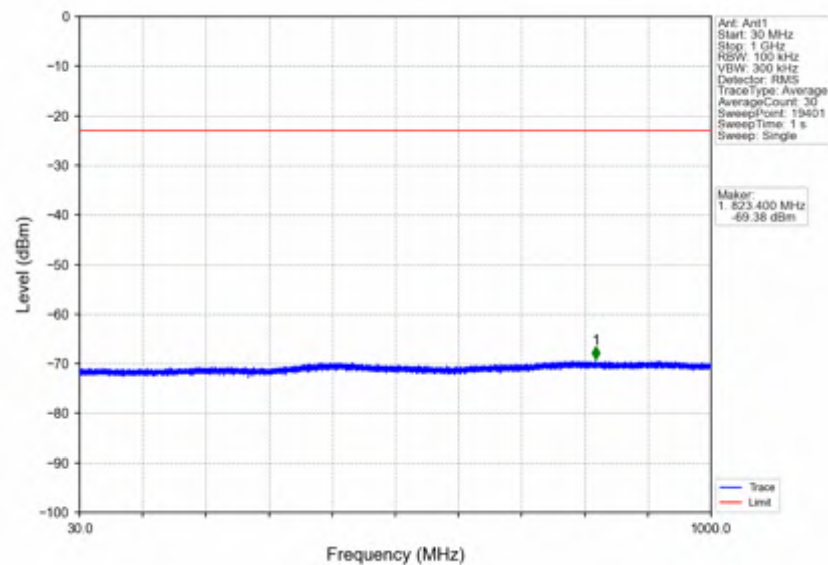
n7 15kHz SISO NTN 50MHz DFT-s-OFDM QPSK 2545MHz Inner 1RB Right
