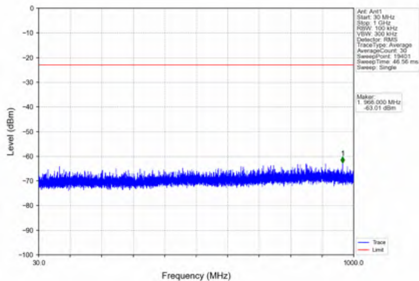
n7_30kHz_SISO_NTNV_30MHz_CP-OFDM QPSK_2515MHz_Edge_1RB_Left
