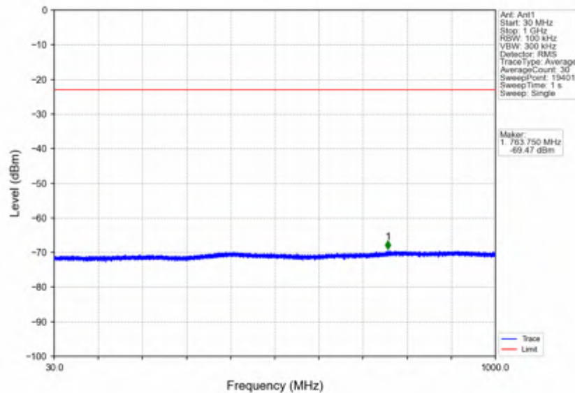
n7_15kHz_SISO_NTNV_50MHz_CP-OFDM_QPSK_2545MHz_Outer_Full
