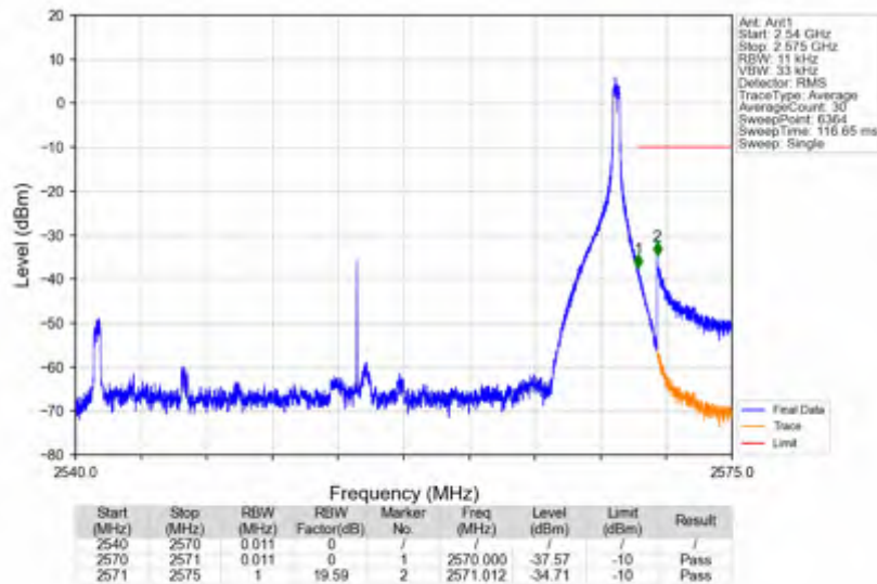
n7_30kHz_SISO_NTNV_30MHz_DFT-s-OFDM_PI/2_BPSK_2555MHz_Edge_1RB_Right
