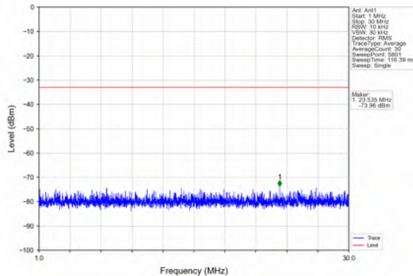
n7_30kHz_SISO_NTNV_25MHz_DFT-s-OFDM QPSK_2535MHz_Edge_1RB_Left
