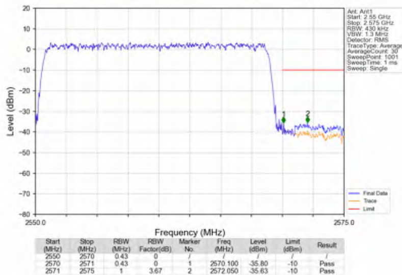
n7_30kHz_SISO_NTNV_20MHz_DFT-s-OFDM QPSK_2560MHz_Outer_Full
