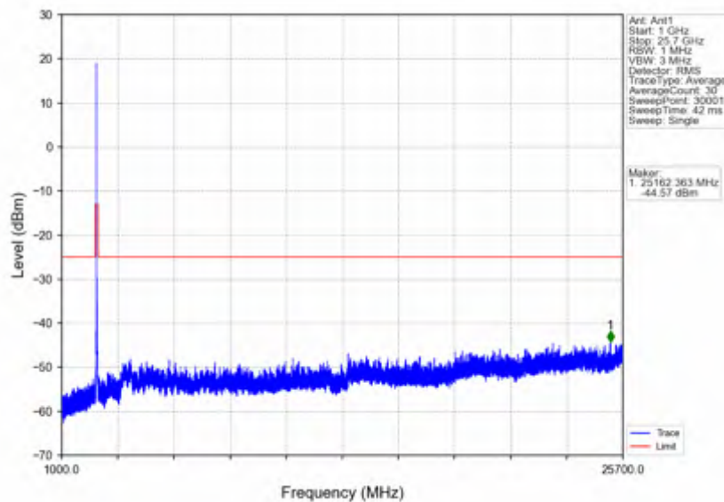
n7_30kHz_SISO_NTNV_30MHz_CP-OFDM QPSK_2555MHz_Edge_1RB_Right
