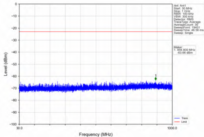
n7_30kHz_SISO_NTNV_20MHz_CP-OFDM QPSK_2560MHz_Edge_1RB_Right
