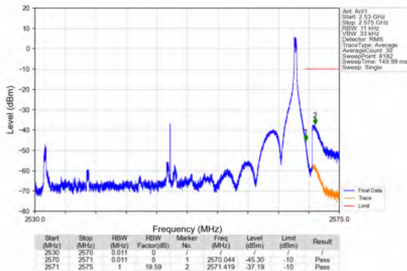
n7_30kHz_SISO_NTNV_40MHz_DFT-s-OFDM PI/2 BPSK_2550MHz_Inner_1RB_Right
