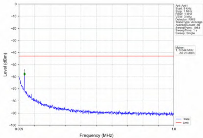
n7_15kHz_SISO_NTNV_50MHz_CP-OFDM_QPSK_2525MHz_Outer_Full
