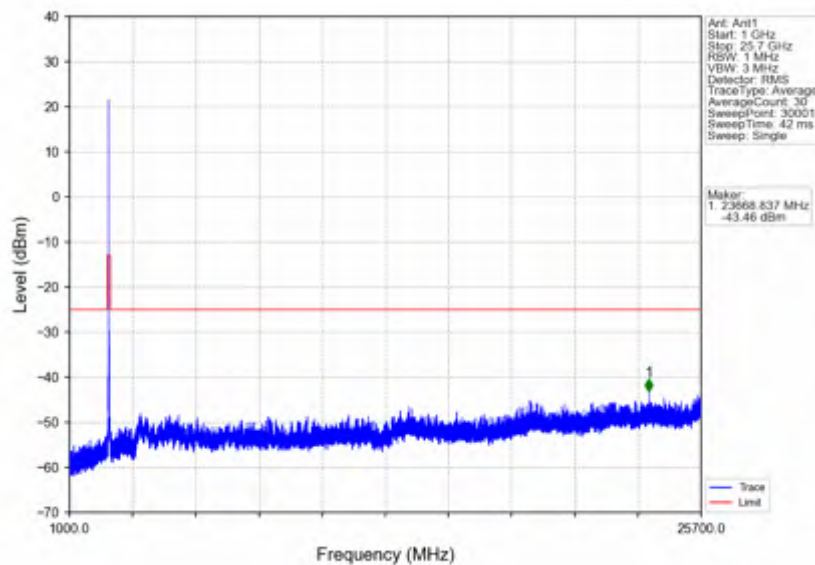
n7_30kHz_SISO_NTNV_25MHz_DFT-s-OFDM QPSK_2557.5MHz_Edge_1RB_Right
