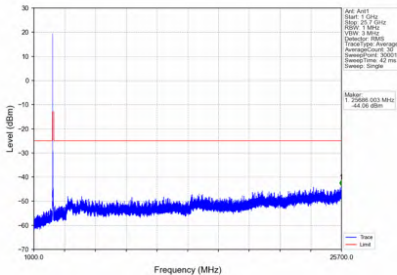
n7_30kHz_SISO_NTNV_25MHz_CP-OFDM_QPSK_2512.5MHz_Outer_Full
