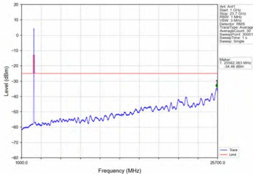
n7_15kHz_SISO_NTNV_50MHz_CP-OFDM_QPSK_2545MHz_Outer_Full
