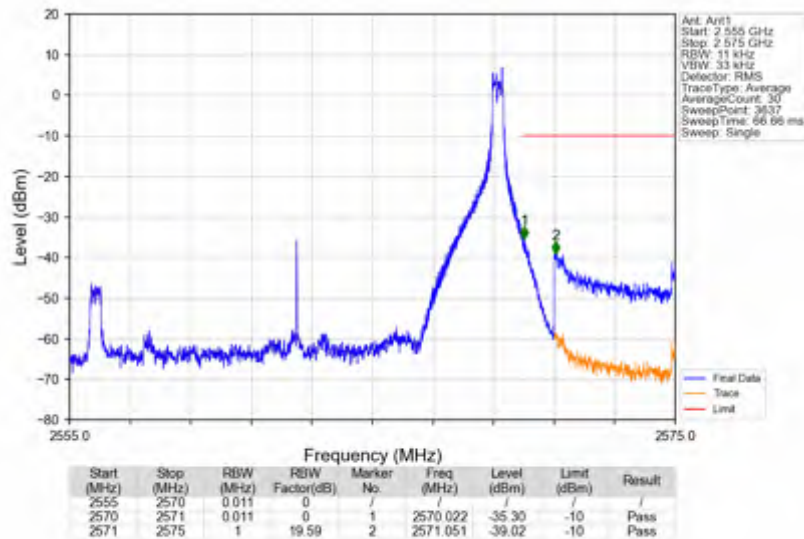
n7_30kHz_SISO_NTNV_15MHz_DFT-s-OFDM_QPSK_2562.5MHz_Edge_1RB_Right
