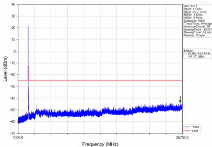
n7_30kHz_SISO_NTNV_40MHz_DFT-s-OFDM QPSK_2550MHz_Edge_1RB_Right
