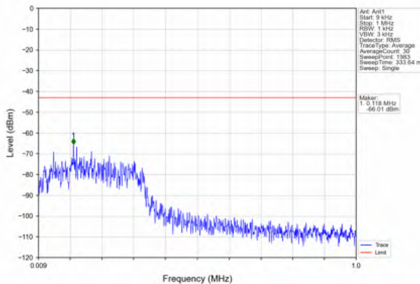
n7_30kHz_SISO_NTNV_30MHz_DFT-s-OFDM_QPSK_2515MHz_Edge_1RB_Left
