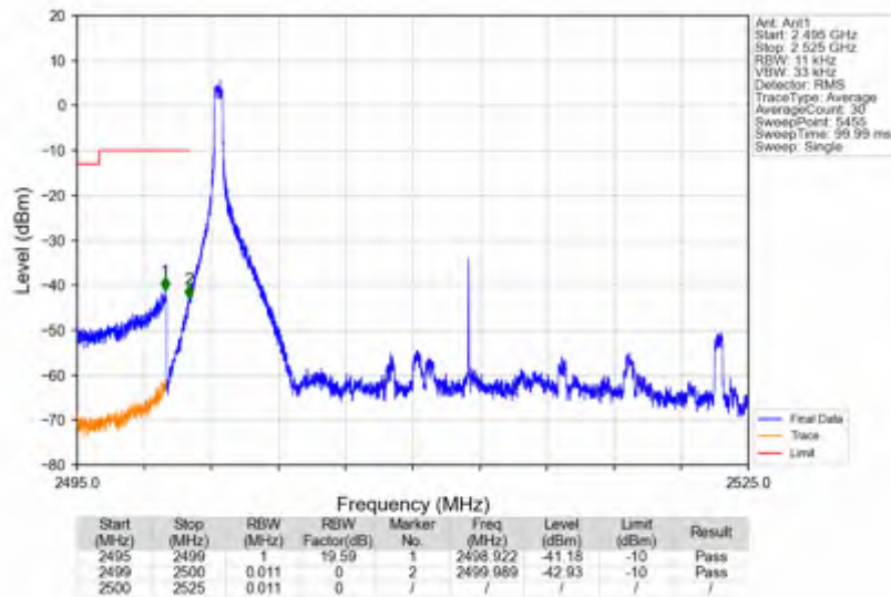
n7_30kHz_SISO_NTNV_25MHz_DFT-s-OFDM_QPSK_2512.5MHz_Inner_1RB_Left
