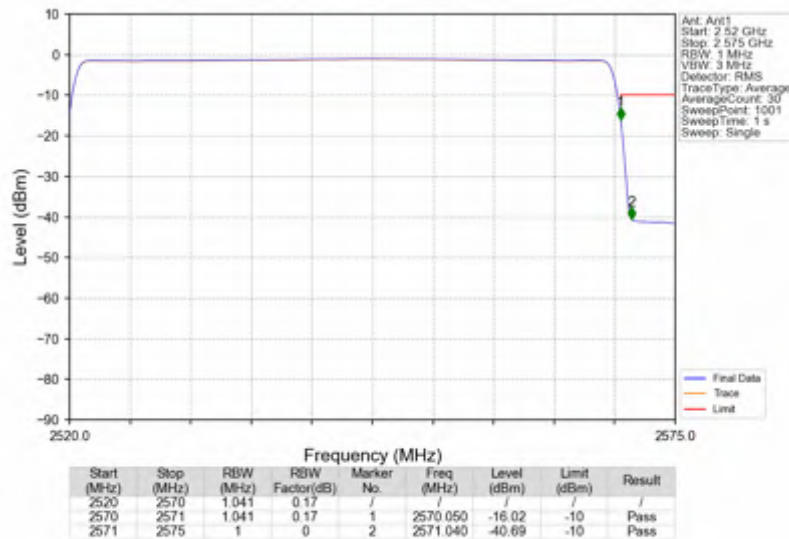
n7_15kHz_SISO_NTNV_50MHz_CP-OFDM QPSK_2545MHz_Outer_Full
