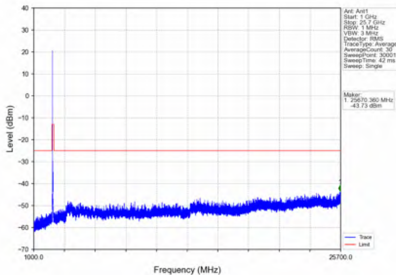
n7_30kHz_SISO_NTNV_40MHz_DFT-s-OFDM QPSK_2520MHz_Outer_Full
