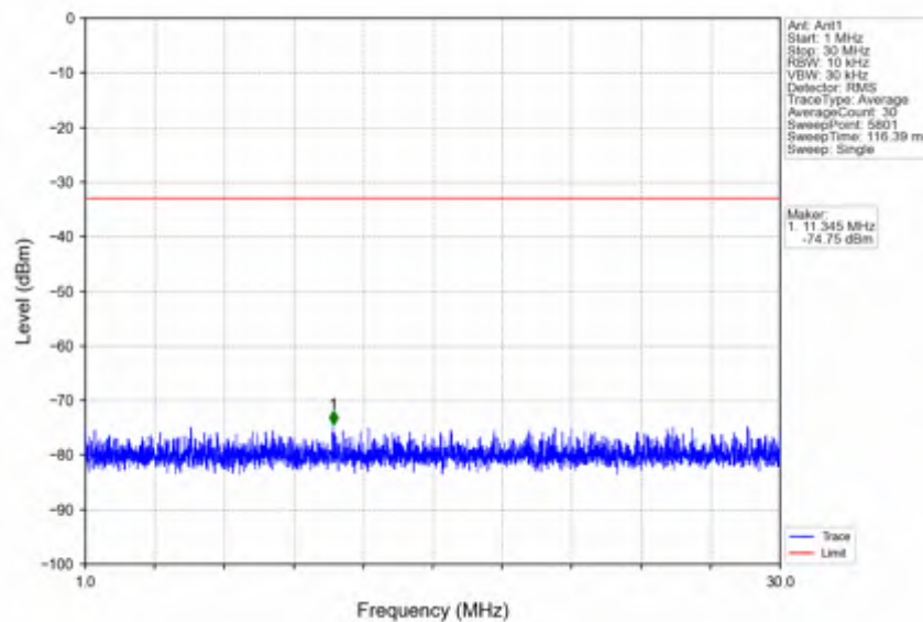
n7_30kHz_SISO_NTNV_10MHz_CP-OFDM QPSK_2535MHz_Edge_1RB_Left
