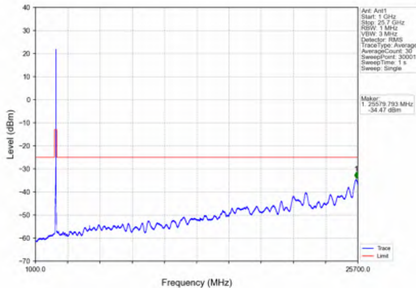
n7_15kHz_SISO_NTNV_50MHz_DFT-s-OFDM QPSK_2545MHz_Edge_1RB_Right
