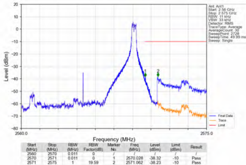
n7_30kHz_SISO_NTNV_10MHz_DFT-s-OFDM QPSK_2565MHz_Edge_1RB_Right
