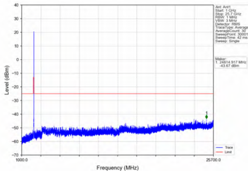
n7_30kHz_SISO_NTNV_20MHz_CP-OFDM QPSK_2560MHz_Edge_1RB_Right
