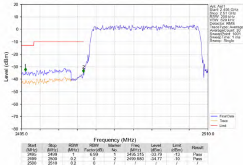
n7_30kHz_SISO_NTNV_10MHz_DFT-s-OFDM QPSK_2505MHz_Outer_Full
