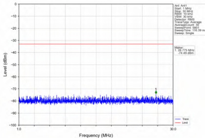
n7_30kHz_SISO_NTNV_25MHz_CP-OFDM QPSK_2535MHz_Edge_1RB_Left
