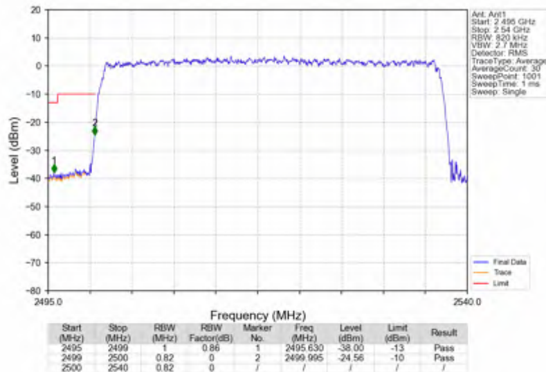
n7_30kHz_SISO_NTNV_40MHz_DFT-s-OFDM QPSK_2520MHz_Outer_Full
