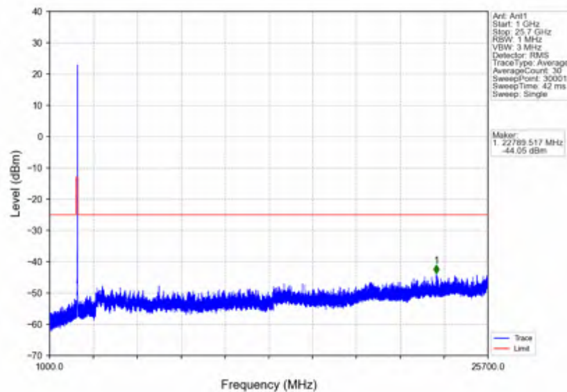
n7_30kHz_SISO_NTNV_20MHz_DFT-s-OFDM_PI/2_BPSK_2560MHz_Edge_1RB_Right
