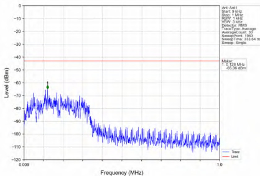
n7_30kHz_SISO_NTNV_10MHz_DFT-s-OFDM_QPSK_2535MHz_Edge_1RB_Left
