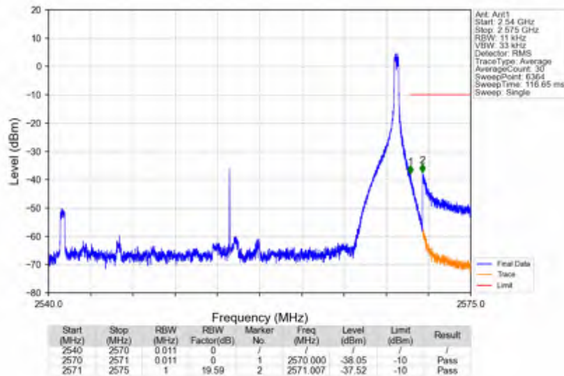
n7_30kHz_SISO_NTNV_30MHz_DFT-s-OFDM QPSK_2555MHz_Edge_1RB_Right
