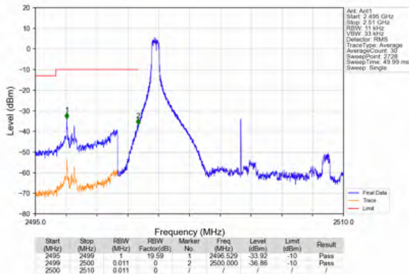
n7_30kHz_SISO_NTNV_10MHz_DFT-s-OFDM_PI/2_BPSK_2505MHz_Edge_1RB_Left
