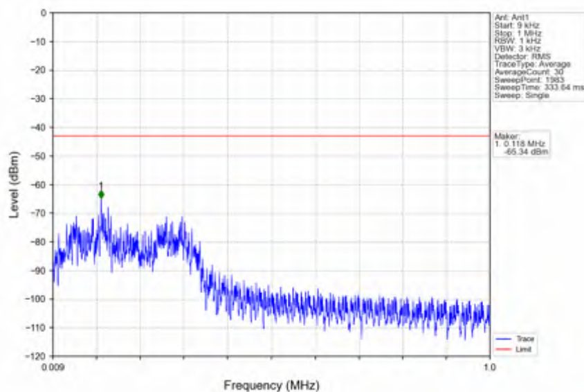
n7_30kHz_SISO_NTNV_25MHz_DFT-s-OFDM_PI/2_BPSK_2512.5MHz_Edge_1RB_Left
