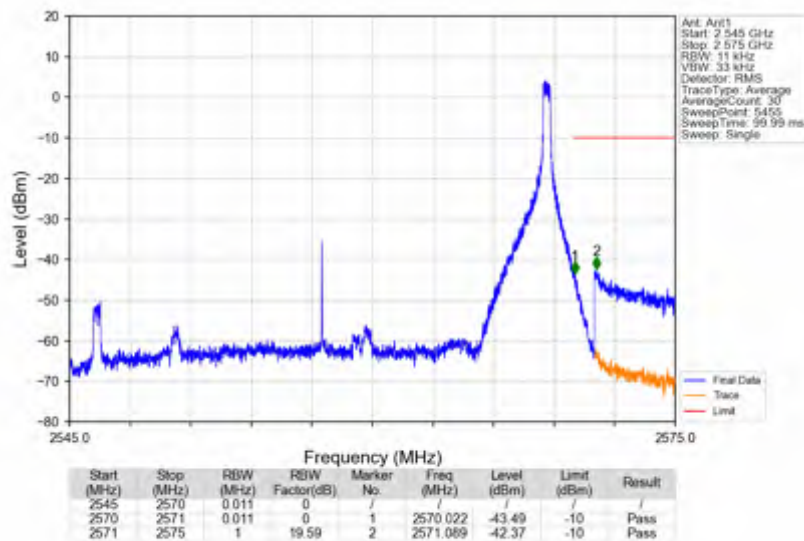
n7_30kHz_SISO_NTNV_25MHz_CP-OFDM QPSK_2557.5MHz_Inner_1RB_Right
