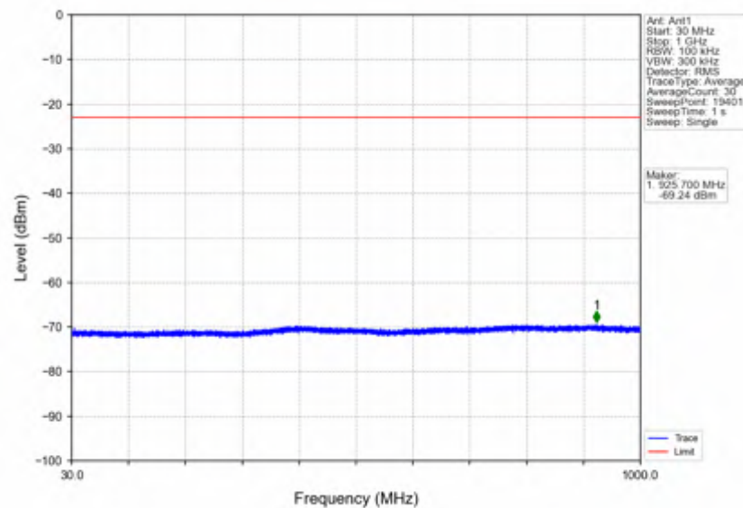
n7_15kHz_SISO_NTNV_50MHz_DFT-s-OFDM_QPSK_2545MHz_Outer_Full
