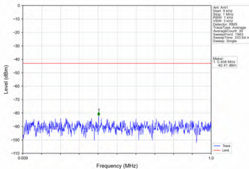
n7_30kHz_SISO_NTNV_20MHz_CP-OFDM QPSK_2535MHz_Edge_1RB_Left
