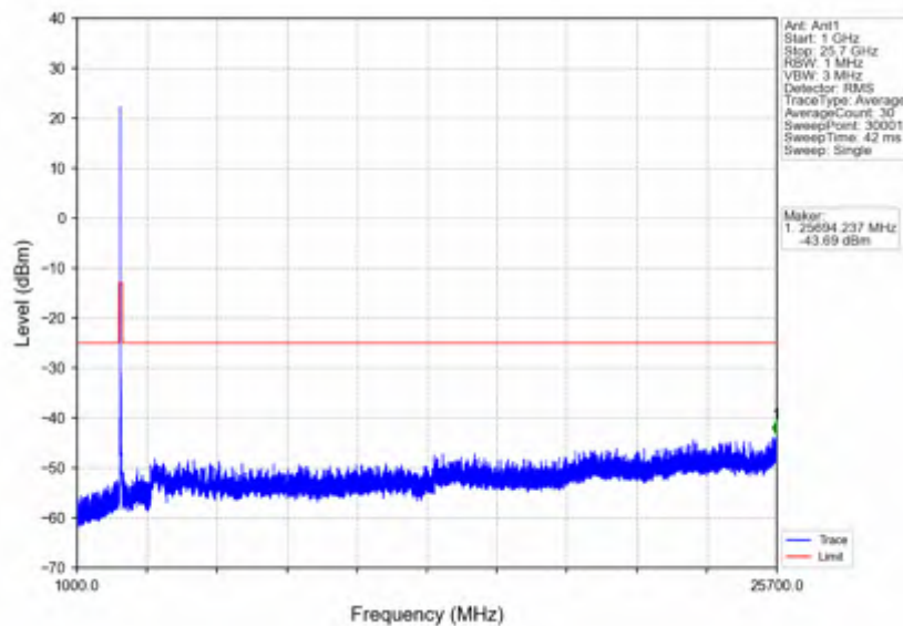
n7_30kHz_SISO_NTNV_30MHz_DFT-s-OFDM QPSK_2555MHz_Edge_1RB_Right
