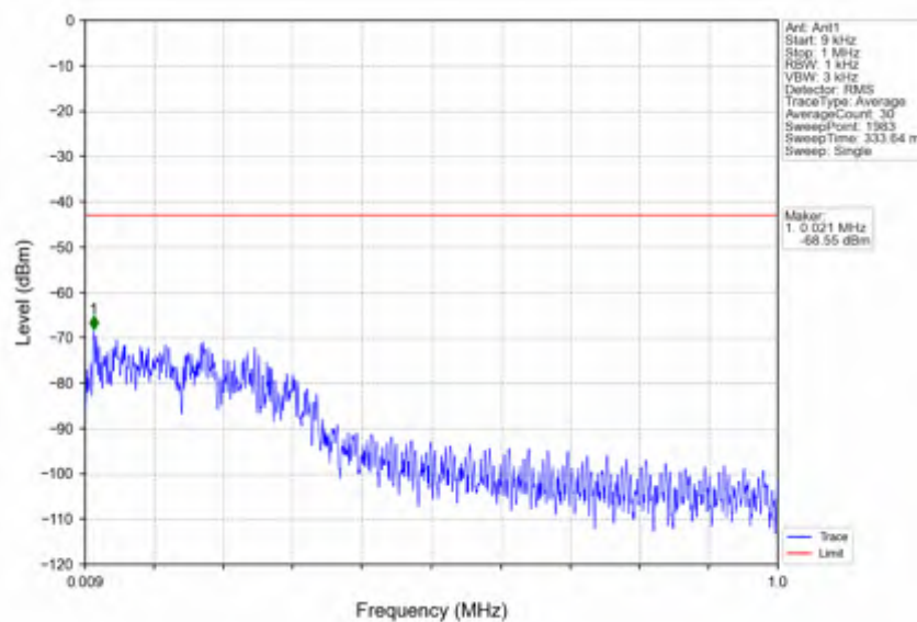
n7_30kHz_SISO_NTNV_15MHz_CP-OFDM_QPSK_2507.5MHz_Edge_1RB_Left
