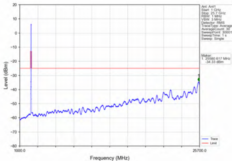
n7_15kHz_SISO_NTNV_50MHz_DFT-s-OFDM QPSK_2545MHz_Inner_1RB_Right
