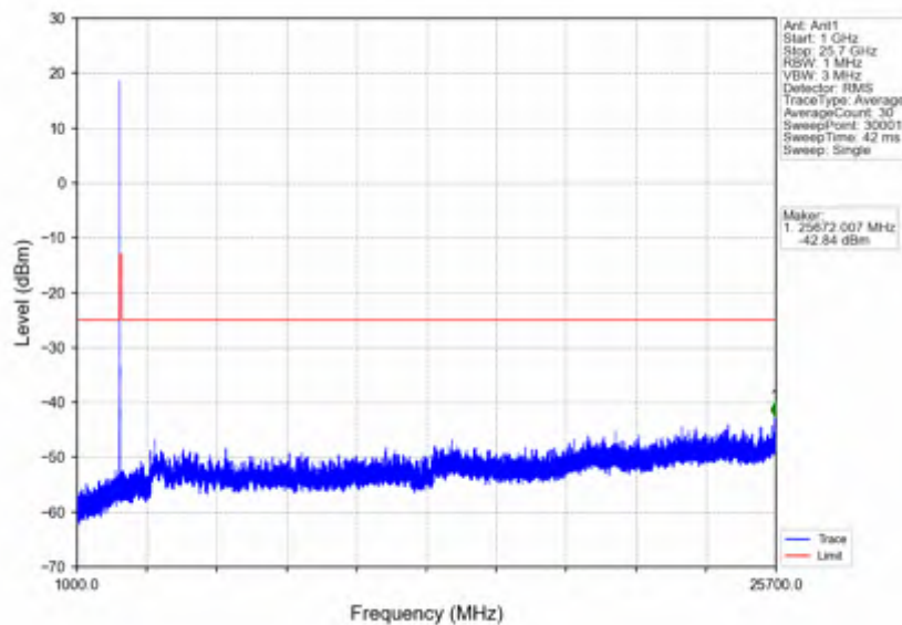
n7_30kHz_SISO_NTNV_10MHz_CP-OFDM QPSK_2505MHz_Outer_Full
