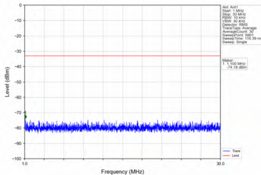
n7_30kHz_SISO_NTNV_25MHz_DFT-s-OFDM QPSK_2512.5MHz_Edge_1RB_Left
