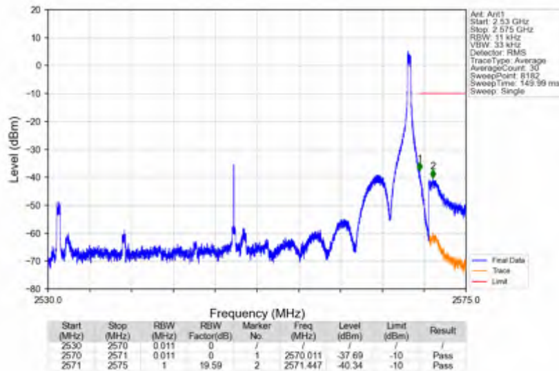
n7_30kHz_SISO_NTNV_40MHz_DFT-s-OFDM QPSK_2550MHz_Edge_1RB_Right
