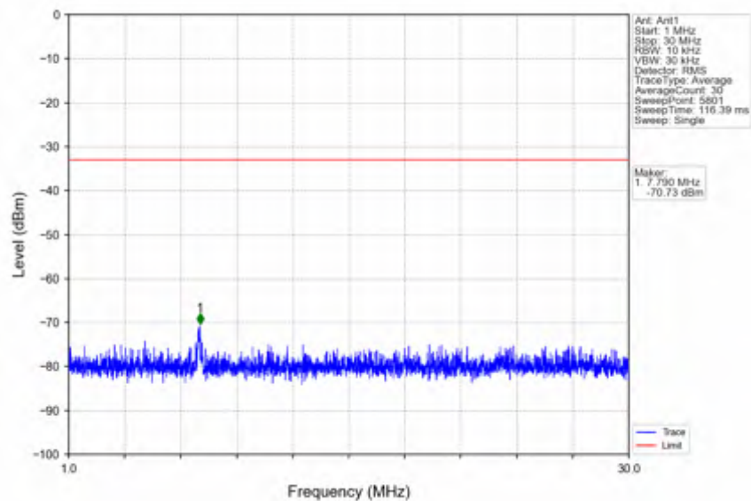
n7_30kHz_SISO_NTNV_25MHz_CP-OFDM_QPSK_2557.5MHz_Edge_1RB_Right
