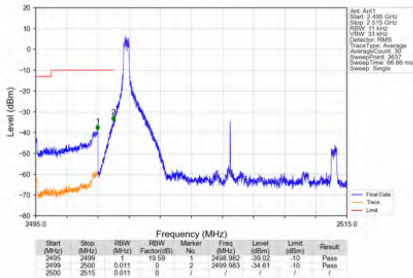
n7_30kHz_SISO_NTNV_15MHz_DFT-s-OFDM_PI/2_BPSK_2507.5MHz_Edge_1RB_Left
