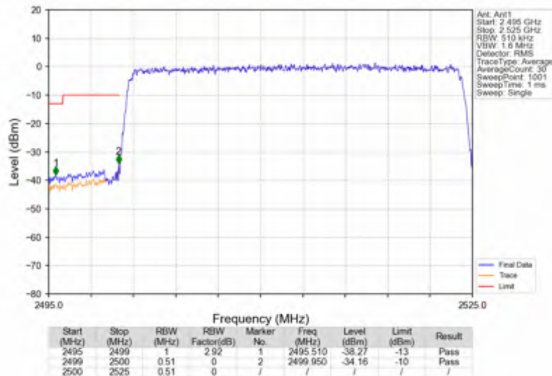
n7_30kHz_SISO_NTNV_25MHz_CP-OFDM_QPSK_2512.5MHz_Outer_Full
