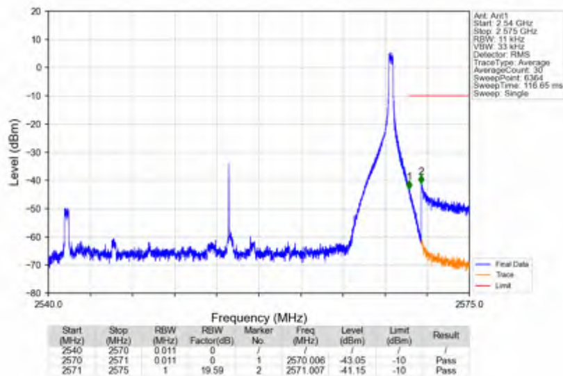
n7_30kHz_SISO_NTNV_30MHz_DFT-s-OFDM_QPSK_2555MHz_Inner_1RB_Right
