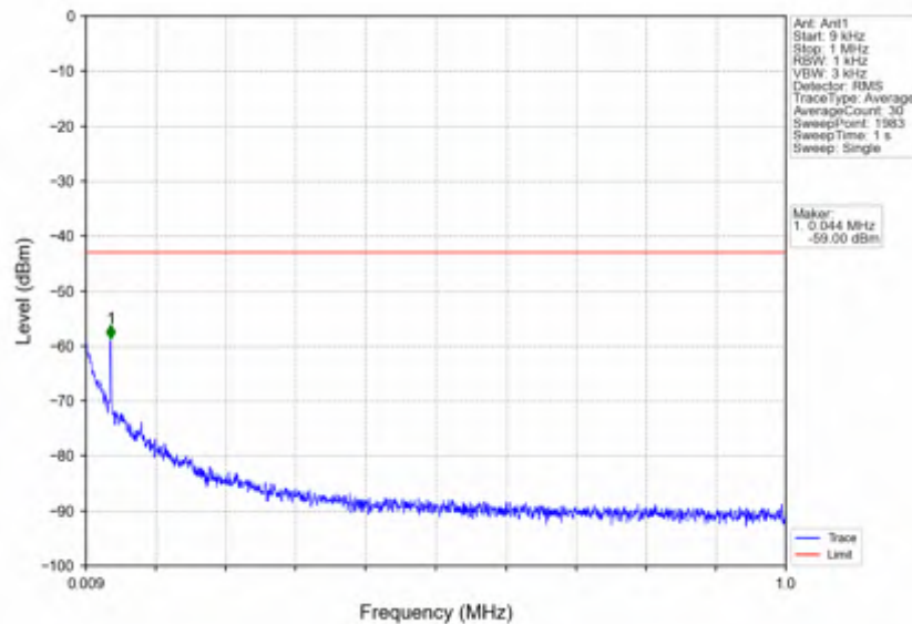
n7_15kHz_SISO_NTNV_50MHz_CP-OFDM QPSK_2535MHz_Edge_1RB_Left
