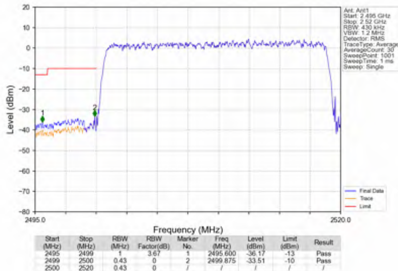
n7_30kHz_SISO_NTNV_20MHz_DFT-s-OFDM QPSK_2510MHz_Outer_Full
