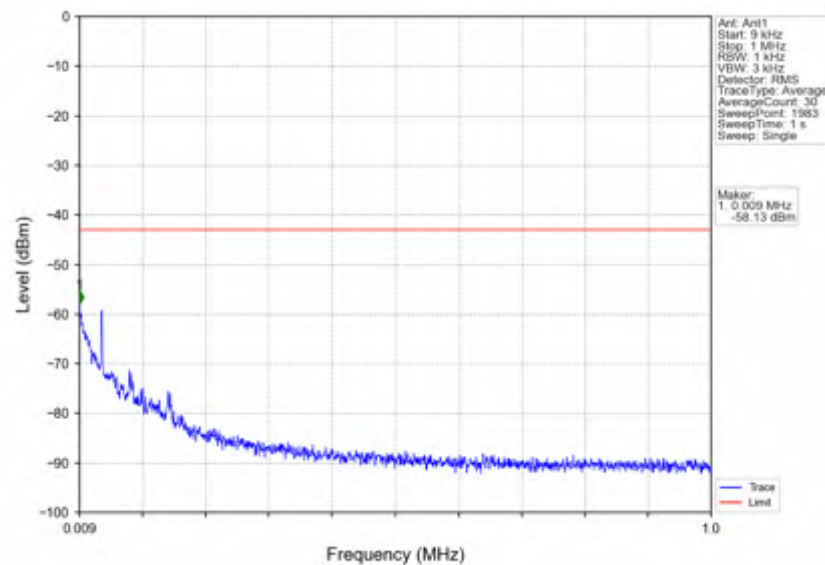
n7_15kHz_SISO_NTNV_50MHz_DFT-s-OFDM_QPSK_2545MHz_Inner_1RB_Right
