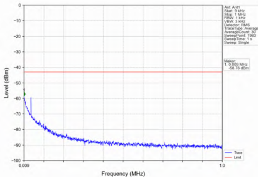
n7_15kHz_SISO_NTNV_50MHz_CP-OFDM QPSK_2525MHz_Edge_1RB_Left
