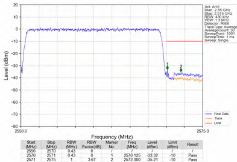
n7_30kHz_SISO_NTNV_20MHz_CP-OFDM QPSK_2560MHz_Outer_Full
