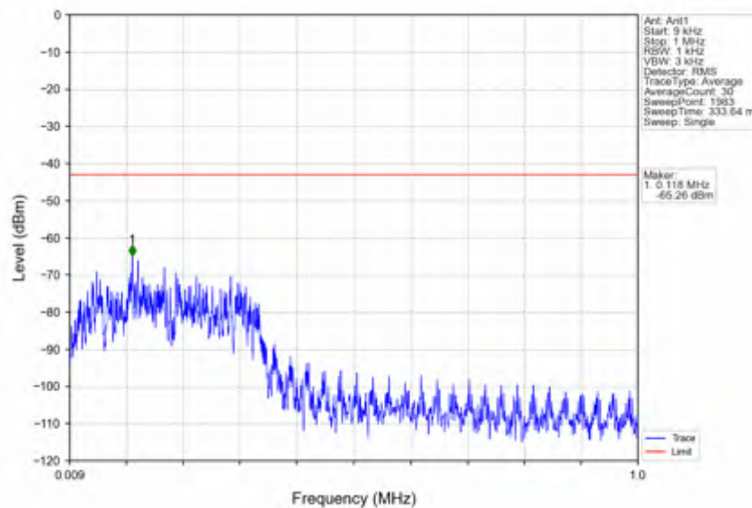
n7_30kHz_SISO_NTNV_20MHz_DFT-s-OFDM_QPSK_2510MHz_Edge_1RB_Left
