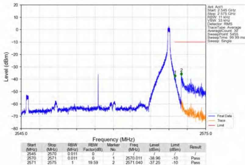
n7_30kHz_SISO_NTNV_25MHz_CP-OFDM QPSK_2557.5MHz_Edge_1RB_Right
