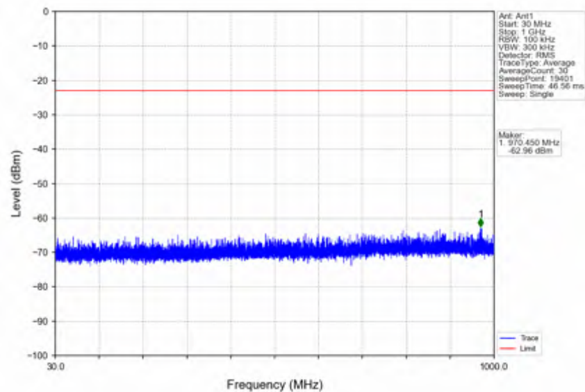
n7_30kHz_SISO_NTNV_15MHz_DFT-s-OFDM_QPSK_2562.5MHz_Edge_1RB_Right
