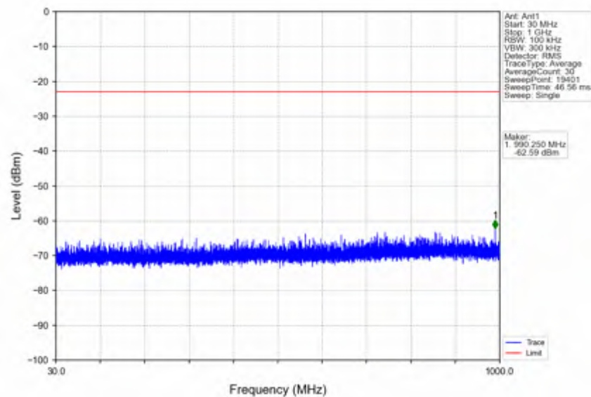
n7_30kHz_SISO_NTNV_15MHz_CP-OFDM QPSK_2507.5MHz_Edge_1RB_Left
