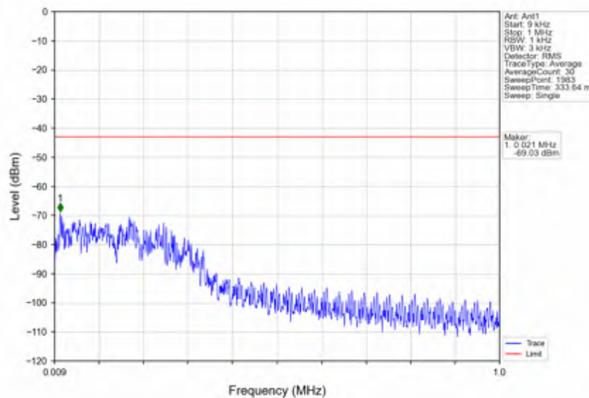
n7_30kHz_SISO_NTNV_25MHz_CP-OFDM_QPSK_2512.5MHz_Edge_1RB_Left
