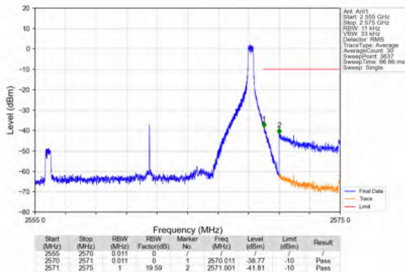
n7_30kHz_SISO_NTNV_15MHz_CP-OFDM QPSK_2562.5MHz_Edge_1RB_Right
