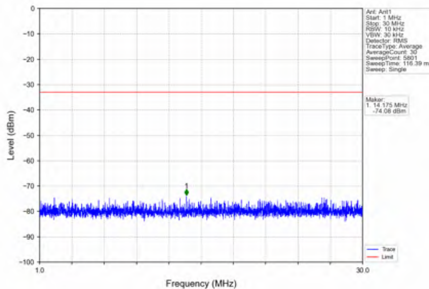
n7_30kHz_SISO_NTNV_15MHz_CP-OFDM QPSK_2535MHz_Edge_1RB_Left
