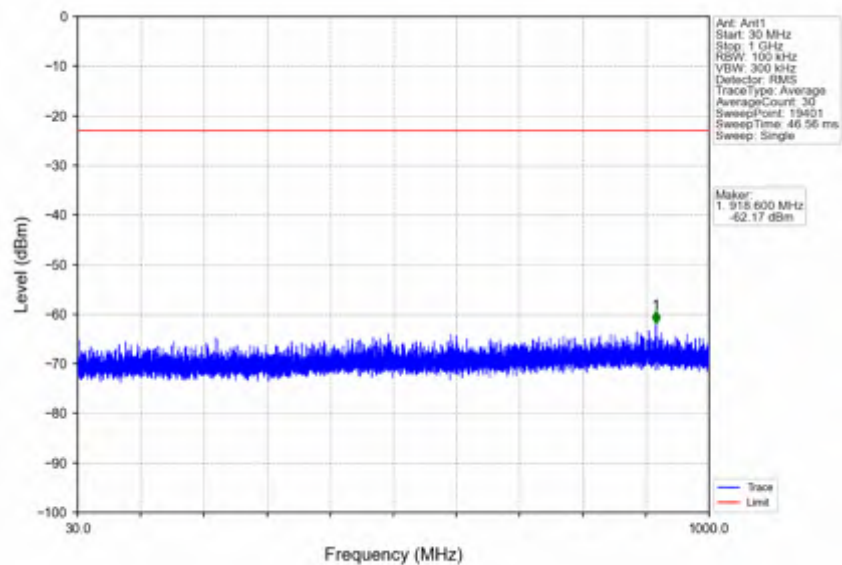
n7_30kHz_SISO_NTNV_40MHz_CP-OFDM QPSK_2520MHz_Edge_1RB_Left
