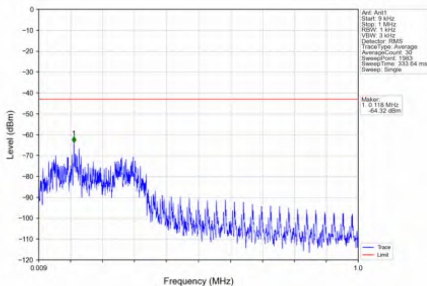
n7_30kHz_SISO_NTNV_10MHz_DFT-s-OFDM_PI/2_BPSK_2505MHz_Edge_1RB_Left
