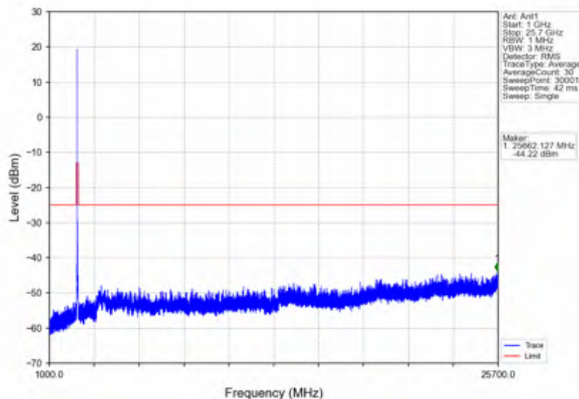
n7_30kHz_SISO_NTNV_25MHz_CP-OFDM QPSK_2557.5MHz_Edge_1RB_Right
