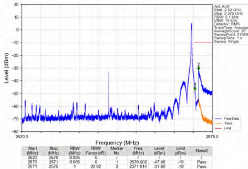
n7_15kHz_SISO_NTNV_50MHz_DFT-s-OFDM QPSK_2545MHz_Inner_1RB_Right
