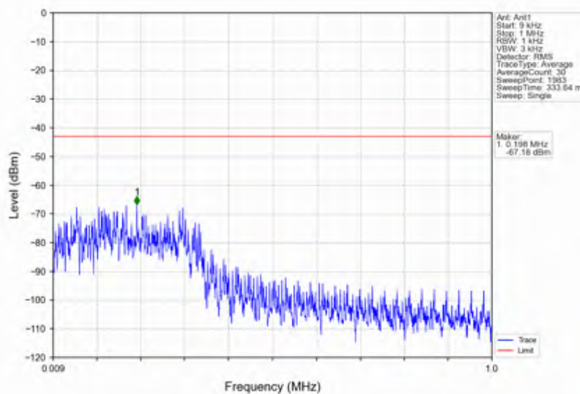
n7_30kHz_SISO_NTNV_40MHz_DFT-s-OFDM_QPSK_2535MHz_Edge_1RB_Left
