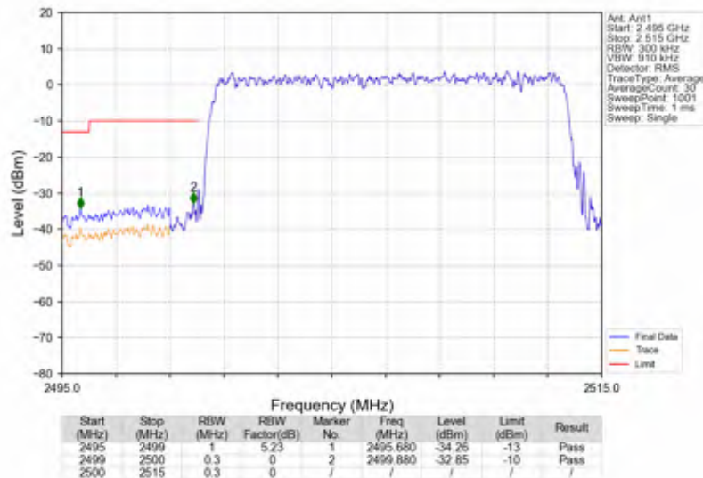
n7_30kHz_SISO_NTNV_15MHz_DFT-s-OFDM QPSK_2507.5MHz_Outer_Full
