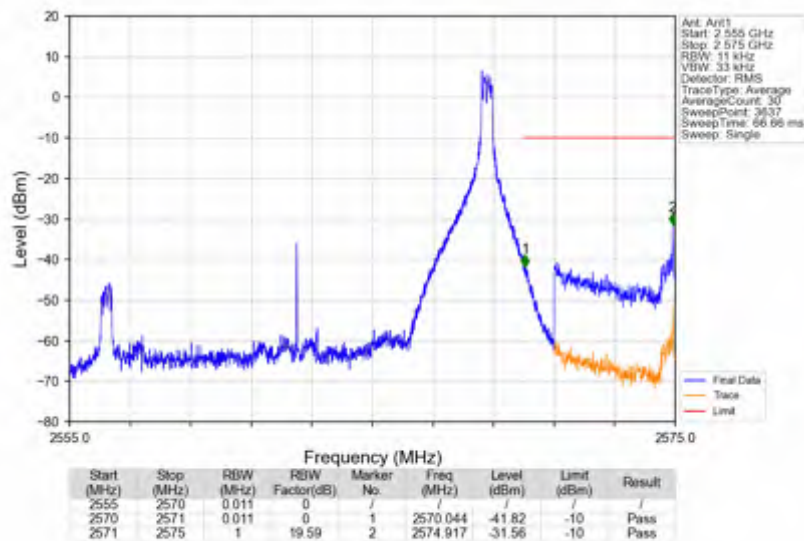
n7_30kHz_SISO_NTNV_15MHz_DFT-s-OFDM PI/2 BPSK_2562.5MHz_Inner_1RB_Right
