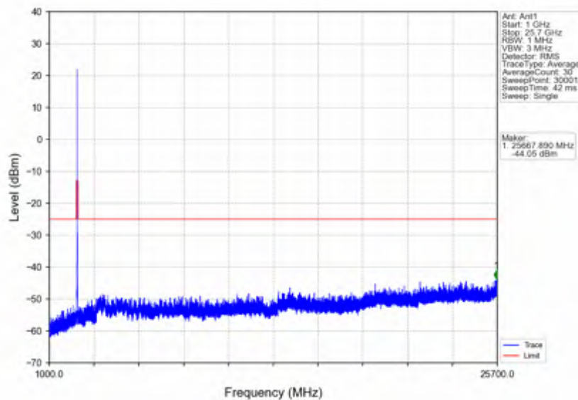
n7_30kHz_SISO_NTNV_15MHz_DFT-s-OFDM_QPSK_2562.5MHz_Edge_1RB_Right
