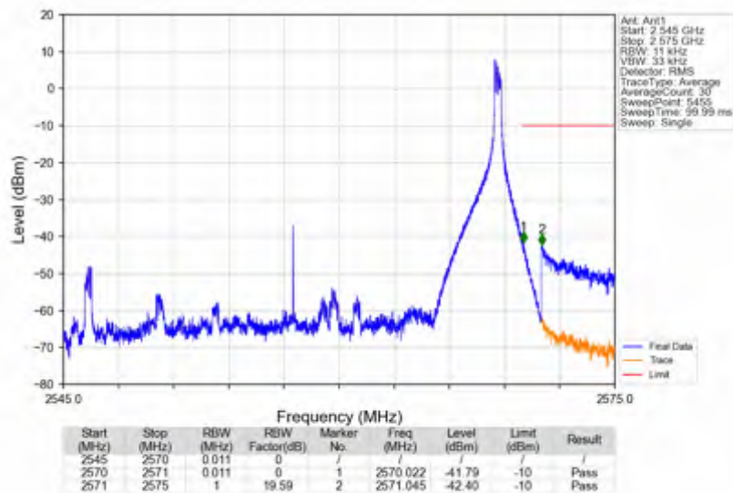
n7_30kHz_SISO_NTNV_25MHz_DFT-s-OFDM PI/2 BPSK_2557.5MHz_Inner_1RB_Right
