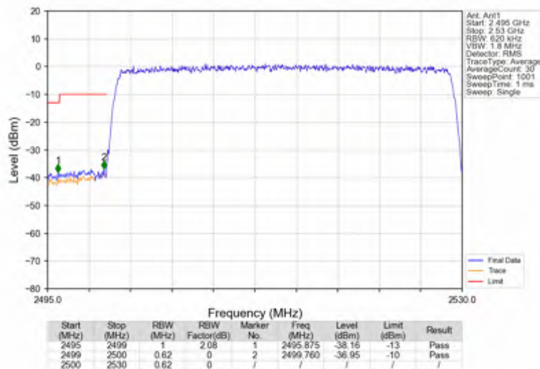
n7_30kHz_SISO_NTNV_30MHz_CP-OFDM QPSK_2515MHz_Outer_Full
