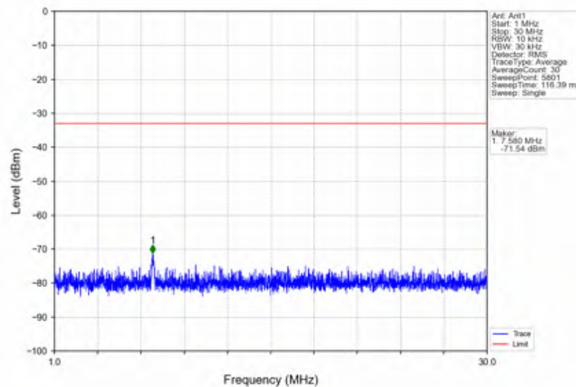
n7_30kHz_SISO_NTNV_30MHz_CP-OFDM_QPSK_2555MHz_Edge_1RB_Right
