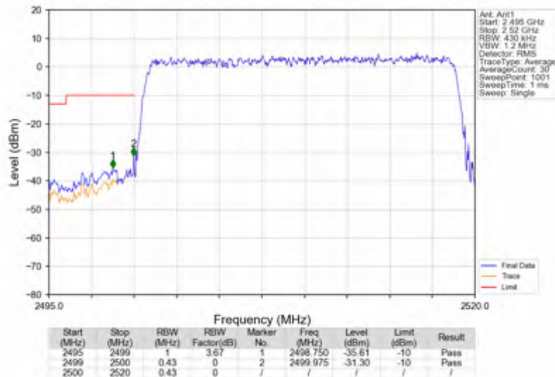
n7_30kHz_SISO_NTNV_20MHz_DFT-s-OFDM PI/2 BPSK_2510MHz_Outer_Full
