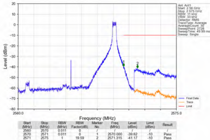
n7_30kHz_SISO_NTNV_10MHz_CP-OFDM QPSK_2565MHz_Edge_1RB_Right
