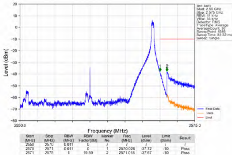
n7_30kHz_SISO_NTNV_20MHz_DFT-s-OFDM PI/2 BPSK_2560MHz_Edge_1RB_Right
