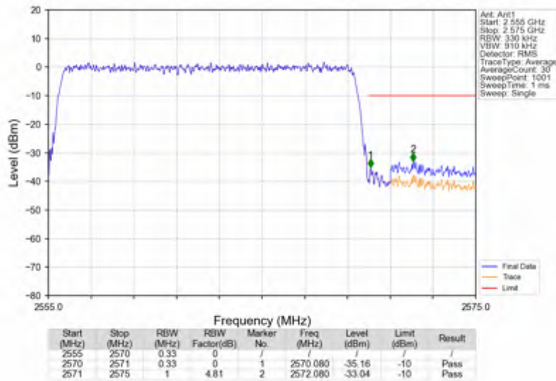
n7_30kHz_SISO_NTNV_15MHz_CP-OFDM QPSK_2562.5MHz_Outer_Full
