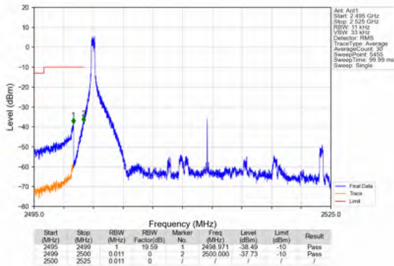
n7_30kHz_SISO_NTNV_25MHz_DFT-s-OFDM_PI/2_BPSK_2512.5MHz_Edge_1RB_Left
