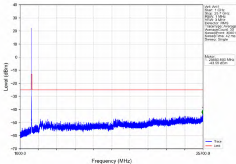
n7_30kHz_SISO_NTNV_30MHz_DFT-s-OFDM_PI/2_BPSK_2555MHz_Edge_1RB_Right
