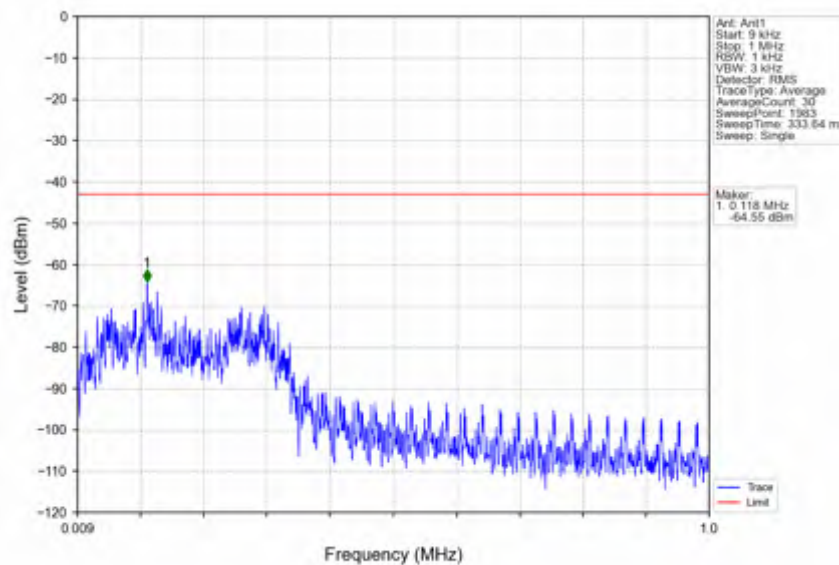
n7_30kHz_SISO_NTNV_15MHz_DFT-s-OFDM_PI/2_BPSK_2535MHz_Edge_1RB_Left
