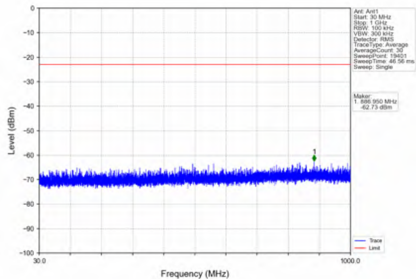
n7_30kHz_SISO_NTNV_30MHz_DFT-s-OFDM QPSK_2535MHz_Edge_1RB_Left
