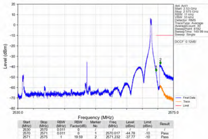
n7_30kHz_SISO_NTNV_40MHz_DFT-s-OFDM_QPSK_2550MHz_Inner_1RB_Right
