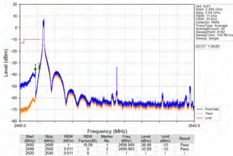
n7_30kHz_SISO_NTNV_40MHz_DFT-s-OFDM_PI/2_BPSK_2520MHz_Edge_1RB_Left
