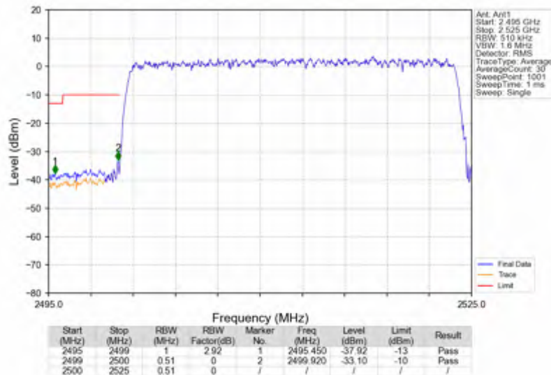
n7_30kHz_SISO_NTNV_25MHz_DFT-s-OFDM QPSK_2512.5MHz_Outer_Full
