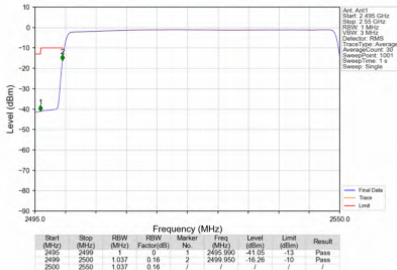
n7_15kHz_SISO_NTNV_50MHz_CP-OFDM QPSK_2525MHz_Outer_Full
