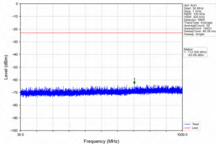
n7_30kHz_SISO_NTNV_30MHz_DFT-s-OFDM QPSK_2515MHz_Edge_1RB_Left
