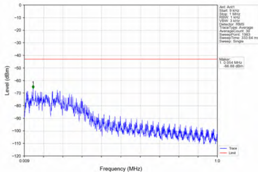
n7_30kHz_SISO_NTNV_15MHz_CP-OFDM_QPSK_2562.5MHz_Edge_1RB_Right
