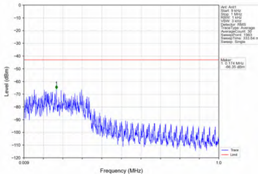
n7_30kHz_SISO_NTNV_15MHz_DFT-s-OFDM QPSK_2535MHz_Edge_1RB_Left
