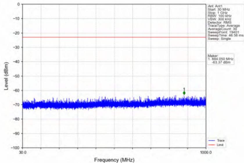
n7_30kHz_SISO_NTNV_25MHz_DFT-s-OFDM_QPSK_2557.5MHz_Edge_1RB_Right
