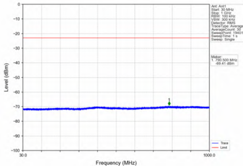
n7_15kHz_SISO_NTNV_50MHz_CP-OFDM_QPSK_2525MHz_Outer_Full
