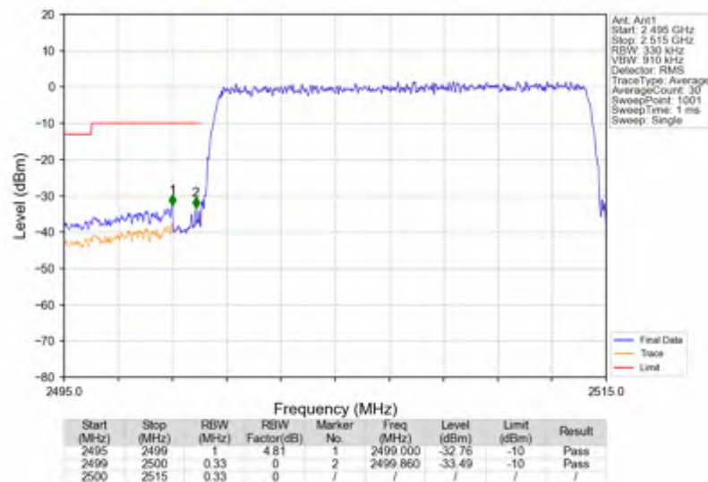
n7_30kHz_SISO_NTNV_15MHz_CP-OFDM QPSK_2507.5MHz_Outer_Full
