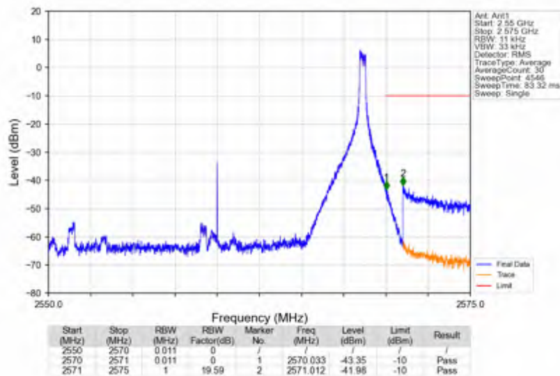
n7_30kHz_SISO_NTNV_20MHz_DFT-s-OFDM QPSK_2560MHz_Inner_1RB_Right
