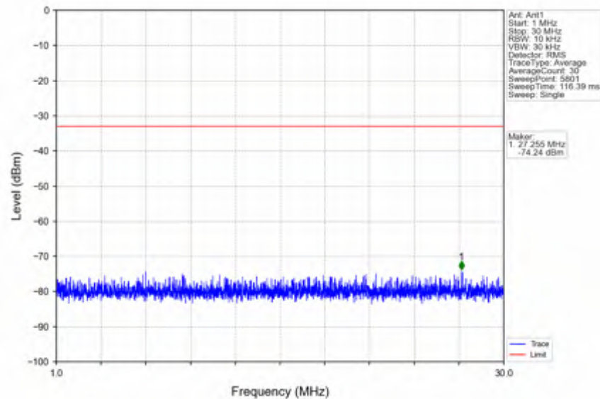
n7_30kHz_SISO_NTNV_15MHz_DFT-s-OFDM QPSK_2507.5MHz_Edge_1RB_Left
