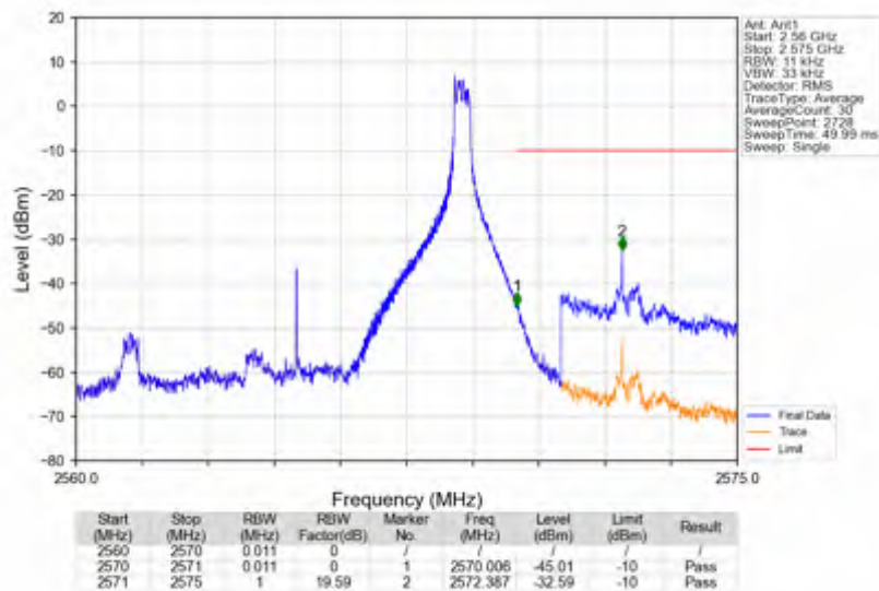
n7_30kHz_SISO_NTNV_10MHz_DFT-s-OFDM PI/2 BPSK_2565MHz_Inner_1RB_Right
