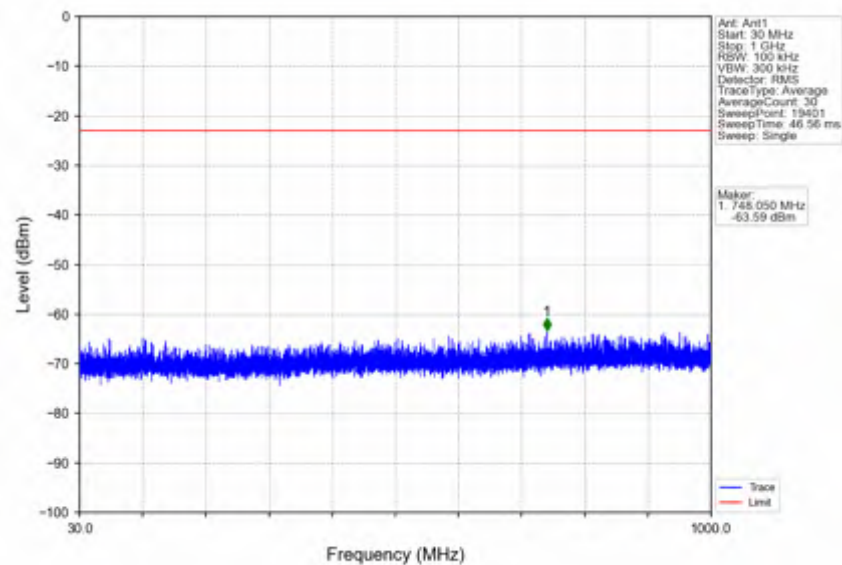
n7_30kHz_SISO_NTNV_10MHz_DFT-s-OFDM QPSK_2535MHz_Edge_1RB_Left
