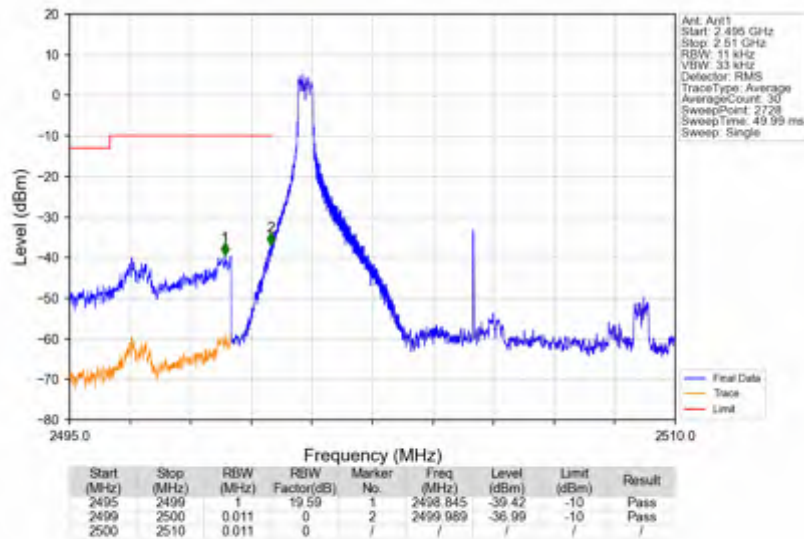
n7_30kHz_SISO_NTNV_10MHz_DFT-s-OFDM QPSK_2505MHz_Edge_1RB_Left
