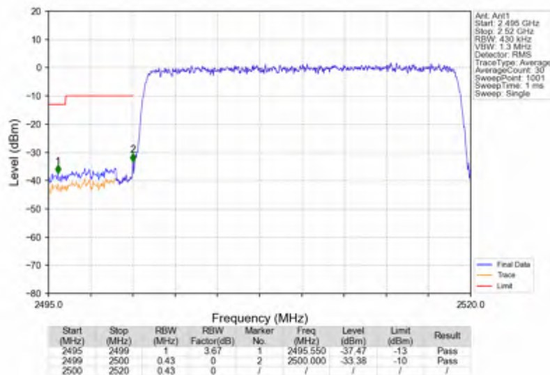
n7_30kHz_SISO_NTNV_20MHz_CP-OFDM QPSK_2510MHz_Outer_Full
