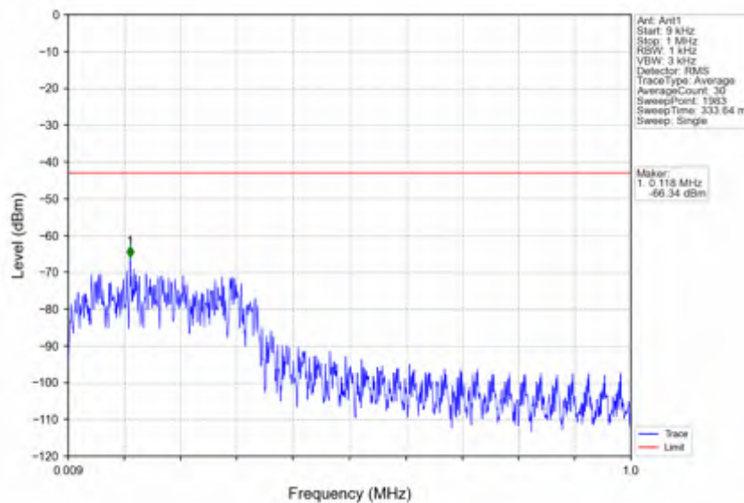
n7_30kHz_SISO_NTNV_30MHz_DFT-s-OFDM QPSK_2535MHz_Edge_1RB_Left
