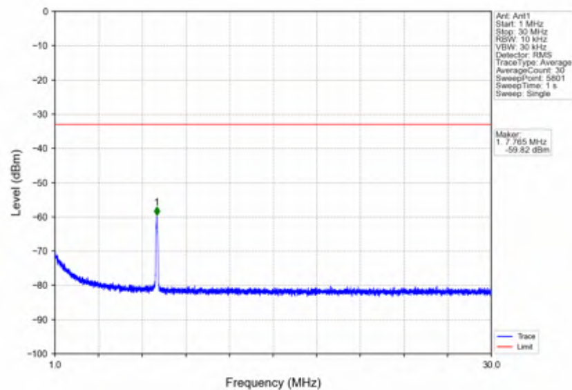
n7_15kHz_SISO_NTNV_50MHz_CP-OFDM QPSK_2545MHz_Inner_1RB_Right
