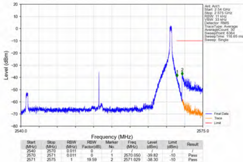
n7_30kHz_SISO_NTNV_30MHz_CP-OFDM QPSK_2555MHz_Edge_1RB_Right
