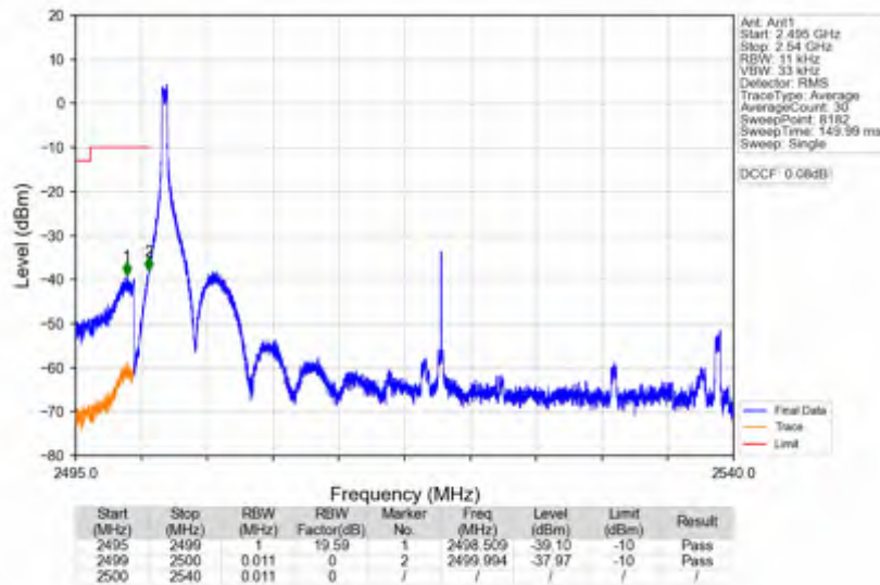
n7_30kHz_SISO_NTNV_40MHz_DFT-s-OFDM_QPSK_2520MHz_Edge_1RB_Left
