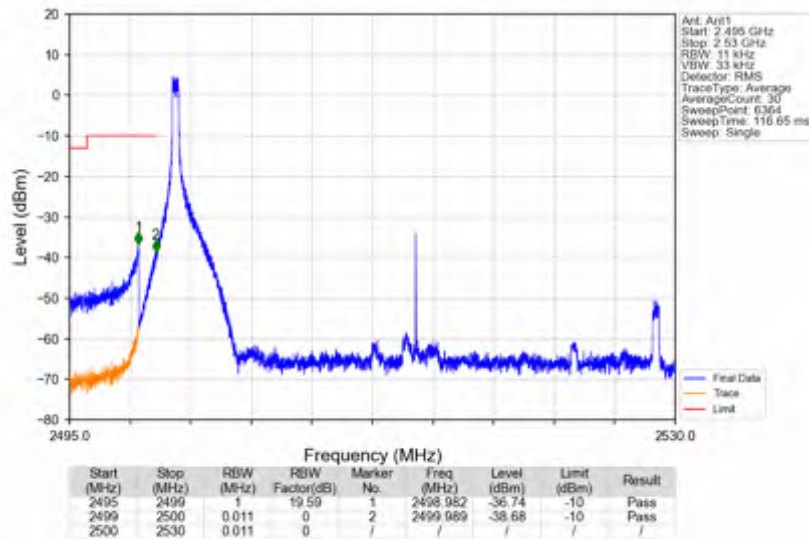
n7_30kHz_SISO_NTNV_30MHz_DFT-s-OFDM_QPSK_2515MHz_Edge_1RB_Left
