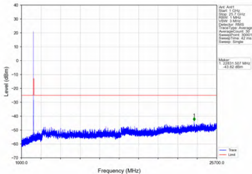
n7_30kHz_SISO_NTNV_15MHz_DFT-s-OFDM QPSK_2507.5MHz_Outer_Full
