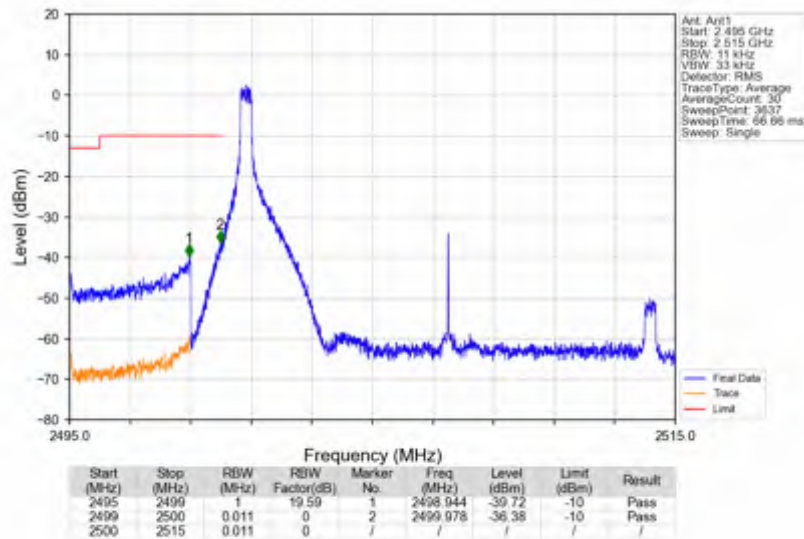
n7_30kHz_SISO_NTNV_15MHz_CP-OFDM_QPSK_2507.5MHz_Edge_1RB_Left
