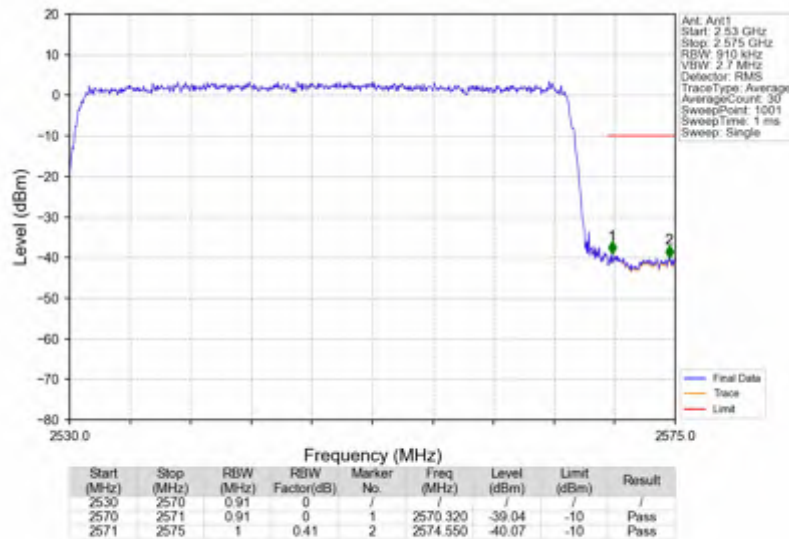
n7_30kHz_SISO_NTNV_40MHz_DFT-s-OFDM_QPSK_2550MHz_Outer_Full
