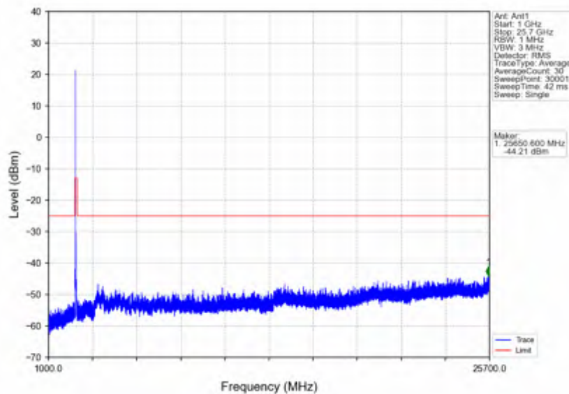
n7_30kHz_SISO_NTNV_30MHz_DFT-s-OFDM QPSK_2515MHz_Outer_Full
