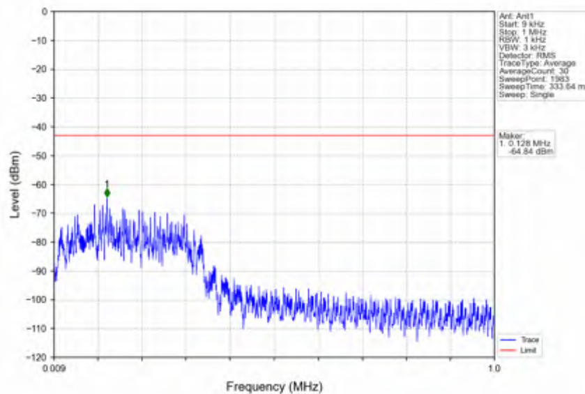
n7_30kHz_SISO_NTNV_20MHz_DFT-s-OFDM_QPSK_2535MHz_Edge_1RB_Left
