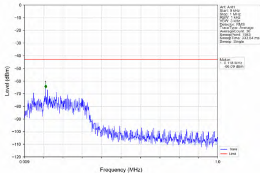
n7_30kHz_SISO_NTNV_40MHz_DFT-s-OFDM QPSK_2550MHz_Edge_1RB_Right
