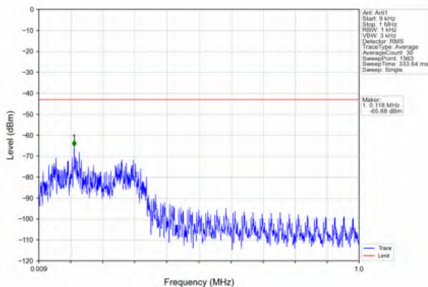
n7_30kHz_SISO_NTNV_40MHz_DFT-s-OFDM_PI/2_BPSK_2520MHz_Edge_1RB_Left
