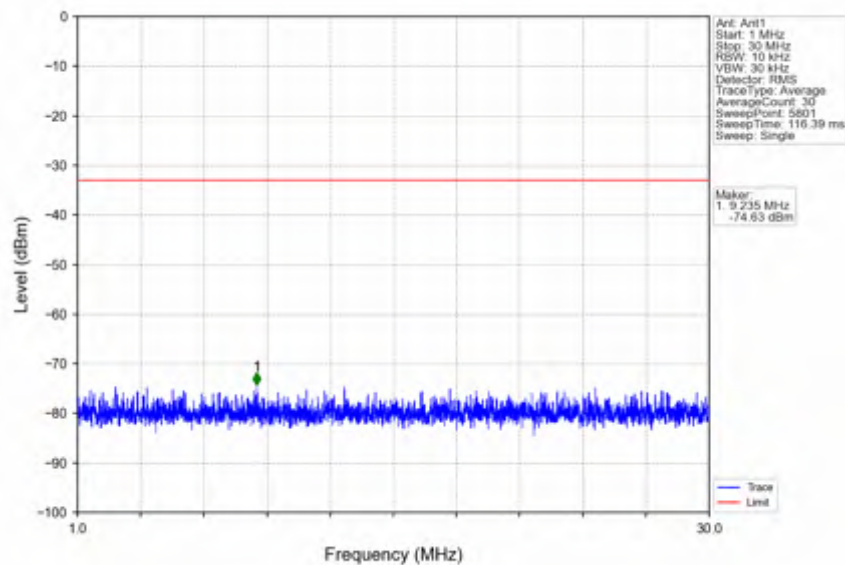
n7_30kHz_SISO_NTNV_40MHz_DFT-s-OFDM PI/2 BPSK_2520MHz_Edge_1RB_Left
