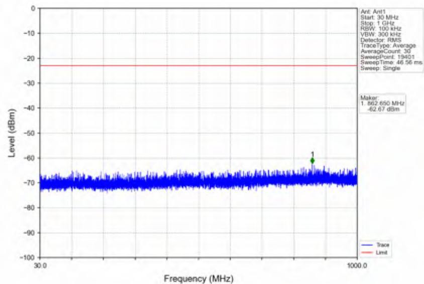
n7_30kHz_SISO_NTNV_15MHz_DFT-s-OFDM QPSK_2535MHz_Edge_1RB_Left
