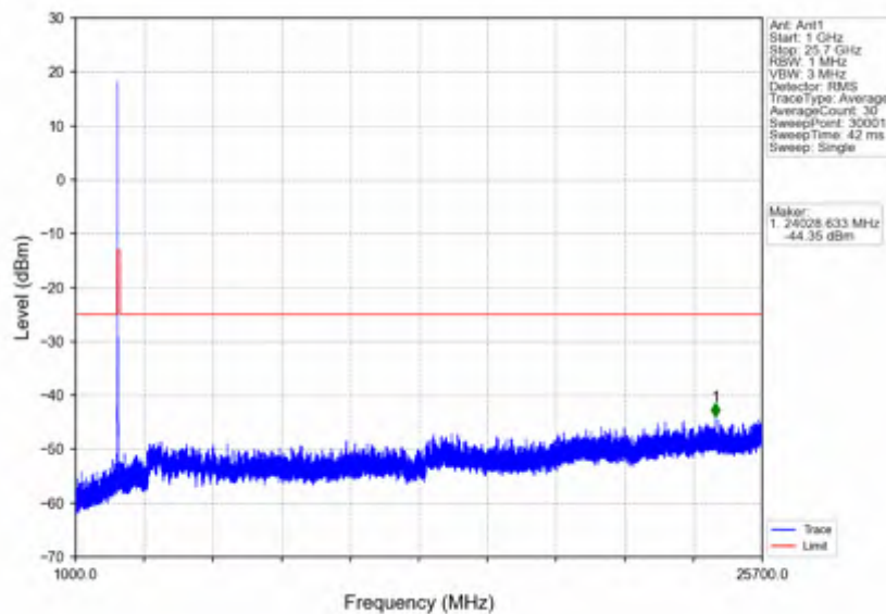
n7_30kHz_SISO_NTNV_20MHz_CP-OFDM QPSK_2510MHz_Outer_Full
