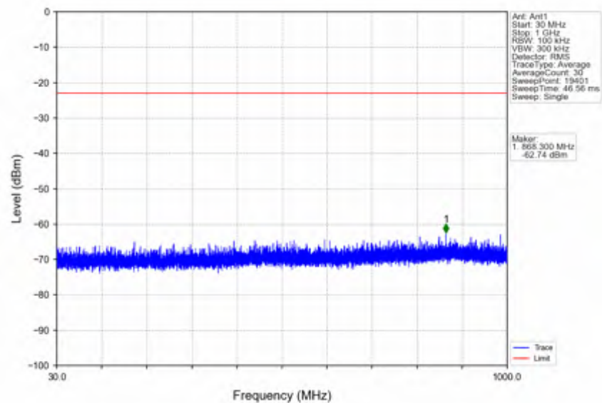
n7_30kHz_SISO_NTNV_20MHz_DFT-s-OFDM QPSK_2510MHz_Edge_1RB_Left
