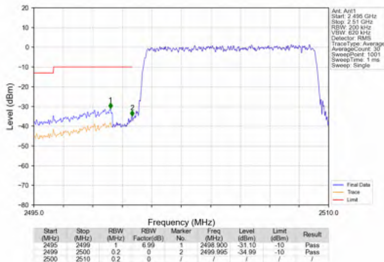
n7_30kHz_SISO_NTNV_10MHz_CP-OFDM QPSK_2505MHz_Outer_Full
