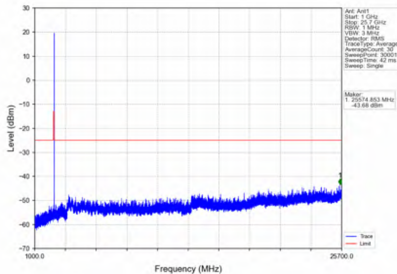
n7_30kHz_SISO_NTNV_10MHz_CP-OFDM QPSK_2565MHz_Edge_1RB_Right
