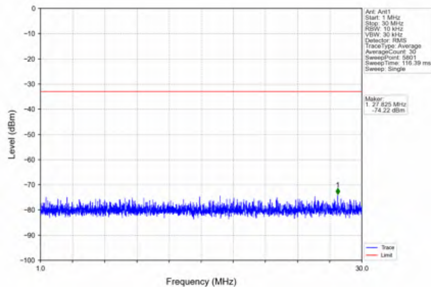
n7_30kHz_SISO_NTNV_10MHz_DFT-s-OFDM QPSK_2535MHz_Edge_1RB_Left
