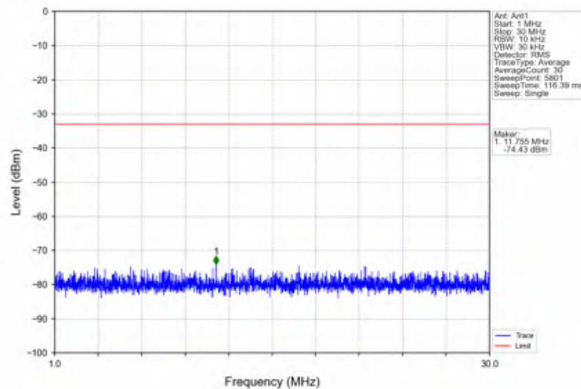
n7_30kHz_SISO_NTNV_10MHz_DFT-s-OFDM QPSK_2505MHz_Edge_1RB_Left
