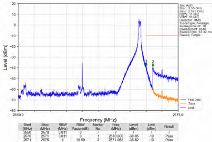
n7_30kHz_SISO_NTNV_20MHz_DFT-s-OFDM QPSK_2560MHz_Edge_1RB_Right
