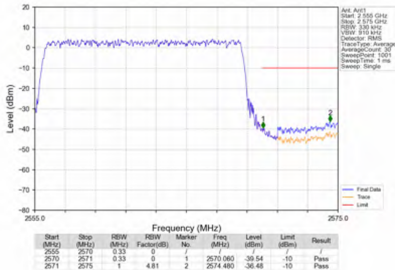
n7_30kHz_SISO_NTNV_15MHz_DFT-s-OFDM PI/2 BPSK_2562.5MHz_Outer_Full
