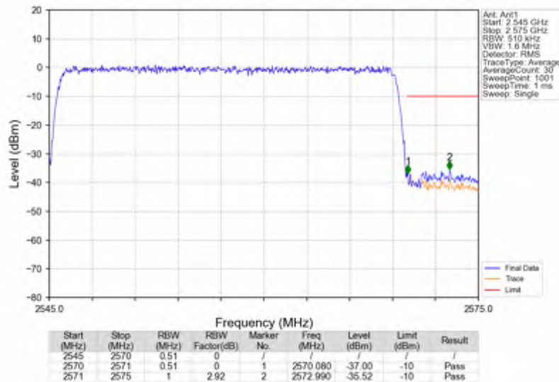
n7_30kHz_SISO_NTNV_25MHz_CP-OFDM QPSK_2557.5MHz_Outer_Full
