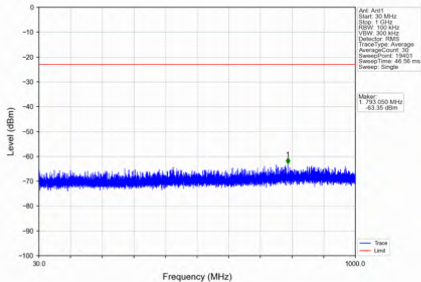
n7_30kHz_SISO_NTNV_40MHz_DFT-s-OFDM QPSK_2535MHz_Edge_1RB_Left
