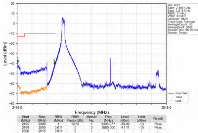
n7_30kHz_SISO_NTNV_15MHz_DFT-s-OFDM_PI/2_BPSK_2507.5MHz_Inner_1RB_Left
