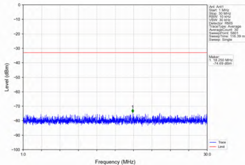
n7_30kHz_SISO_NTNV_25MHz_CP-OFDM QPSK_2512.5MHz_Edge_1RB_Left
