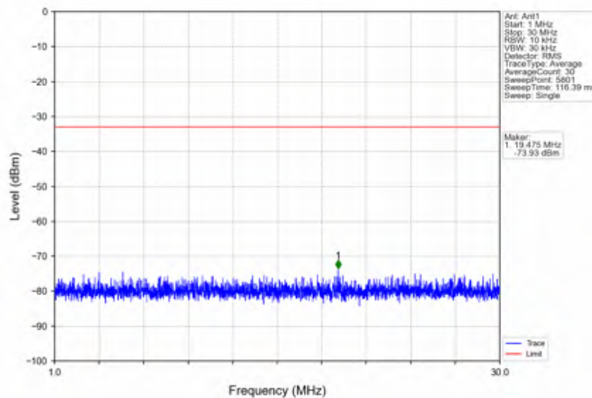
n7_30kHz_SISO_NTNV_10MHz_CP-OFDM QPSK_2505MHz_Edge_1RB_Left
