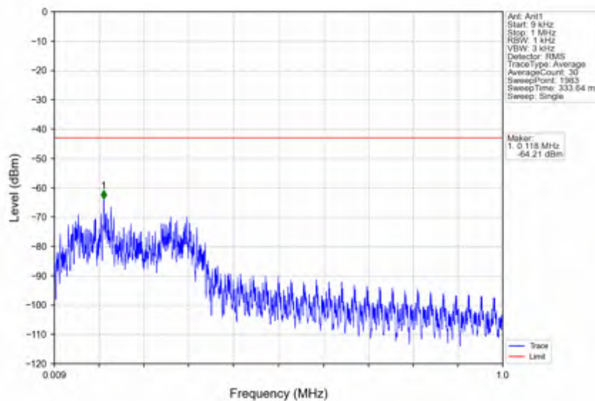
n7_30kHz_SISO_NTNV_10MHz_DFT-s-OFDM PI/2 BPSK_2535MHz_Edge_1RB_Left
