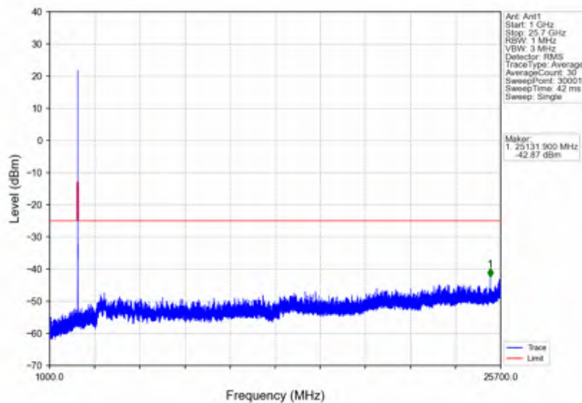
n7_30kHz_SISO_NTNV_10MHz_DFT-s-OFDM QPSK_2565MHz_Edge_1RB_Right
