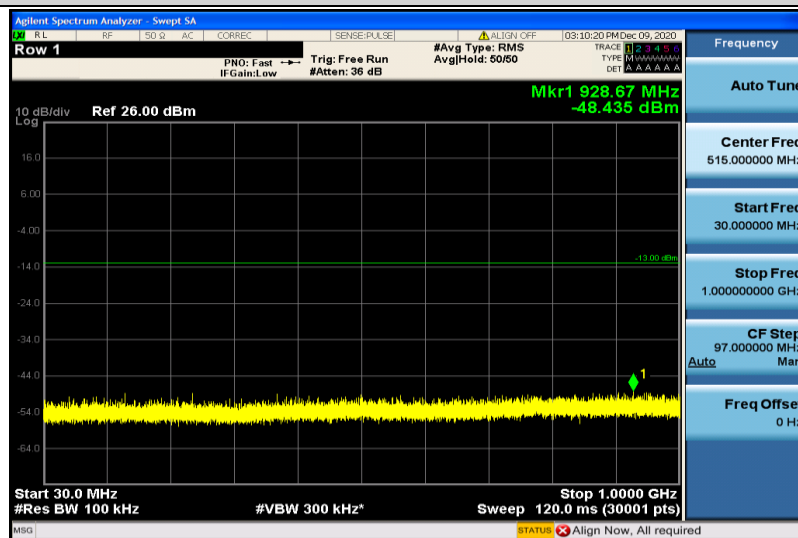
Band4-20MHz-16QAM-20175-1RB#0-30~1000MHz
