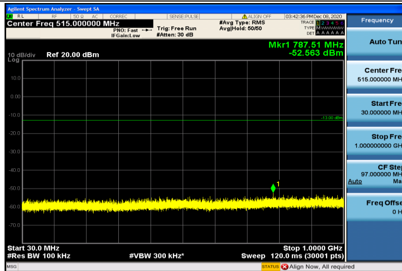
Band66-1.4MHz-QPSK-131979-1RB#0-30~1000MHz
