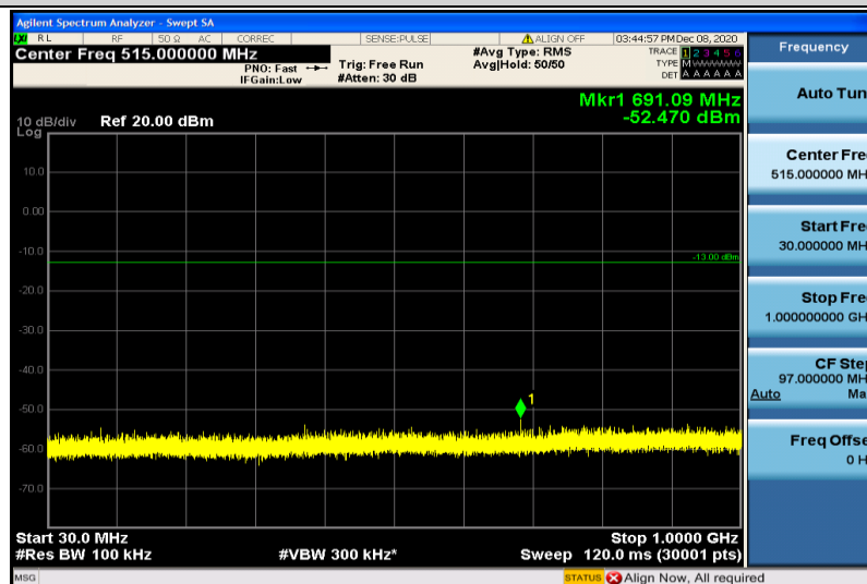
Band66-1.4MHz-QPSK-132322-1RB#0-30~1000MHz
