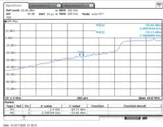
802.11ax-20 MHz (SU) LOW CHANNEL, Reference level
