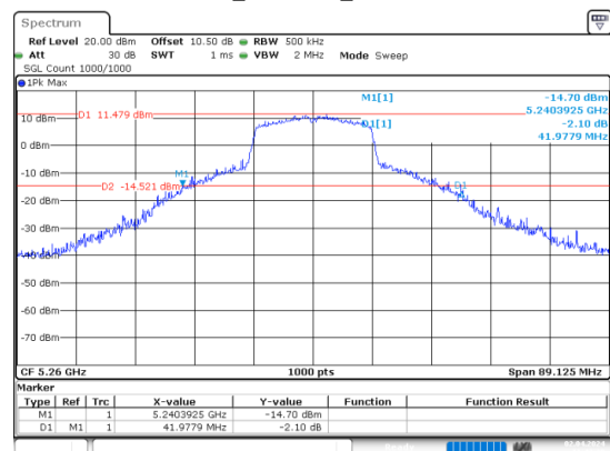
n20_5260MHz_Chain 0
