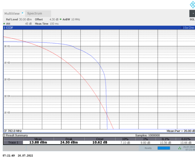
Band13-5MHz-QPSK-23230-6RB#0
