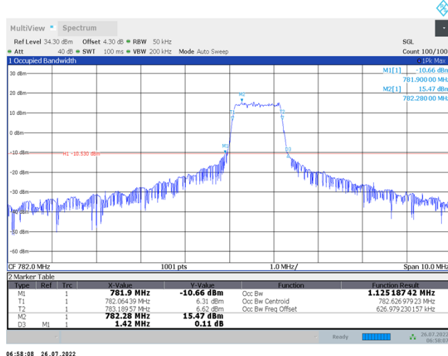
Band13-5MHz-QPSK-23230-6RB#0
