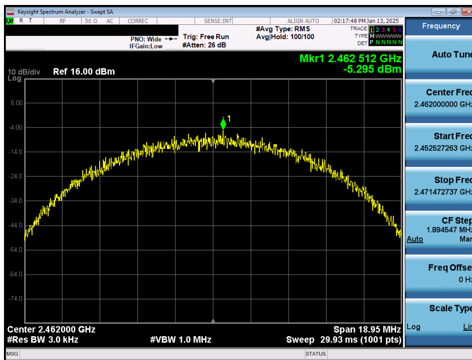
Plot 7-13. Power Spectral Density Plot Antenna WF8 (Common) (802.11b – Ch. 11)
