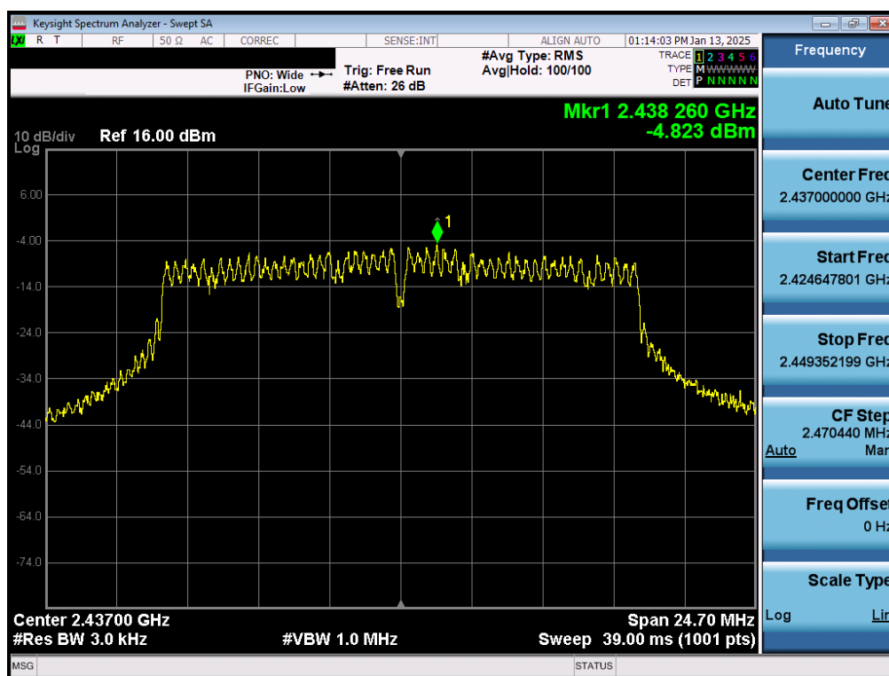
Plot 7-10. Power Spectral Density Plot Antenna WF8 (Dedicated) (802.11g – Ch. 6)
