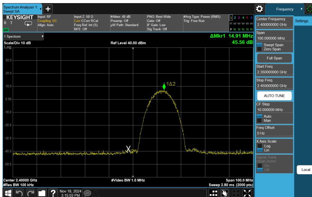
Plot 7-78. Band Edge Plot Antenna WF7b (802.11b – Ch. 1)
