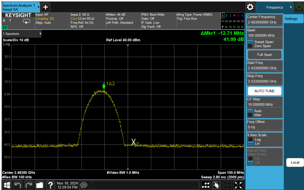
Plot 7-36. Band Edge Plot Antenna WF8 (802.11b – Ch. 13)
