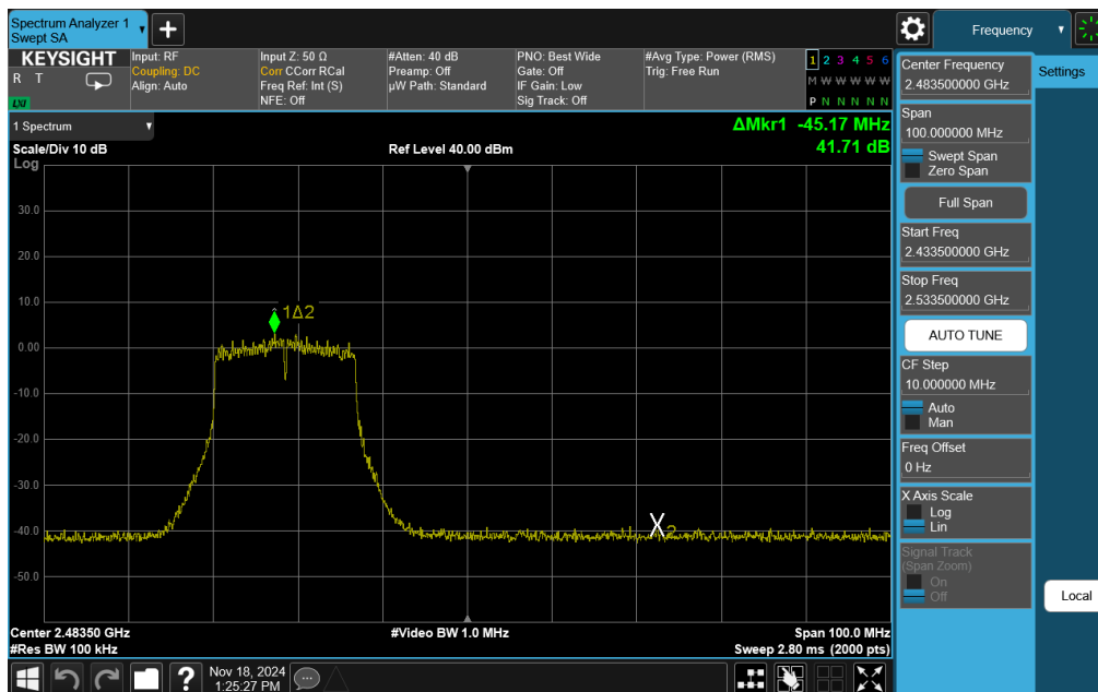
Plot 7-48. Band Edge Plot Antenna WF8 (802.11g – Ch. 11)
