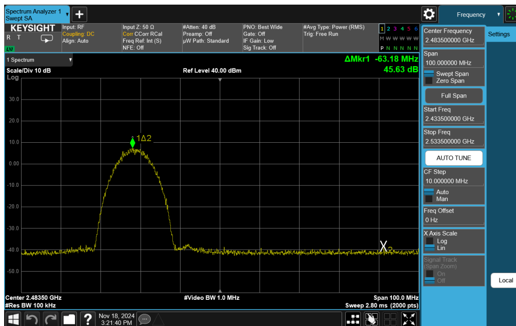
Plot 7-79. Band Edge Plot Antenna WF7b (802.11b – Ch. 11)
