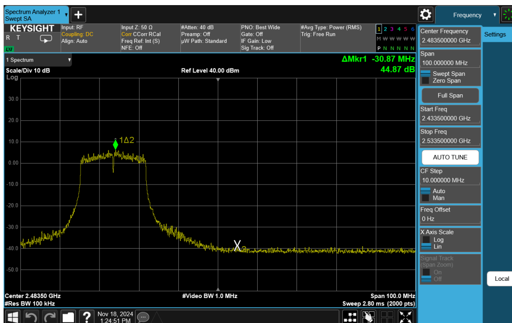
Plot 7-47. Band Edge Plot Antenna WF8 (802.11g – Ch. 10)
