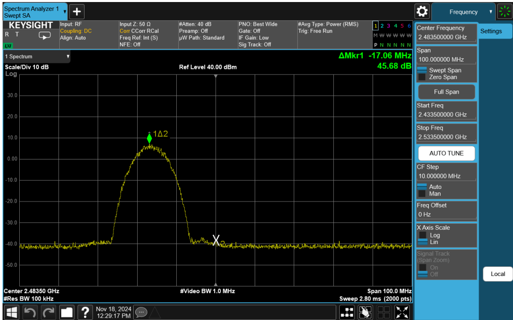
Plot 7-35. Band Edge Plot Antenna WF8 (802.11b – Ch. 12)
