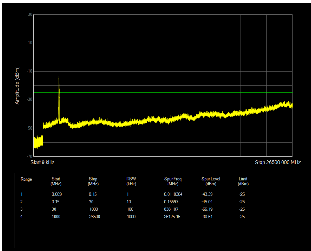
Band41(2555-2655) QAM16 BW=5MHz Channel=40265 RB Size=1 Position=#0
