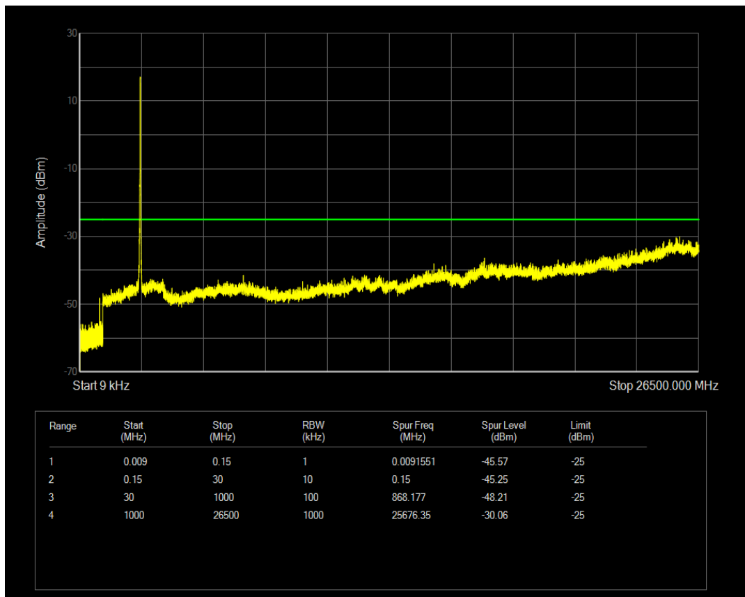
Band41(2555-2655) QAM16 BW=20MHz Channel=41140 RB Size=1 Position=#0
