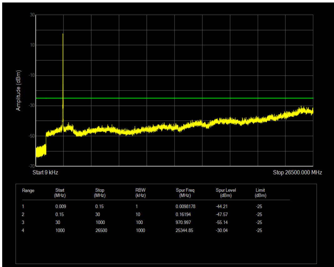
Band41(2555-2655) QAM16 BW=15MHz Channel=41165 RB Size=1 Position=#0
