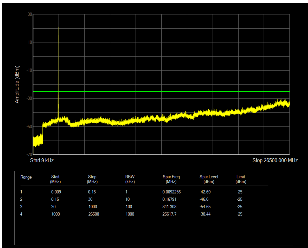
Band41(2555-2655) QAM16 BW=5MHz Channel=41215 RB Size=1 Position=#0
