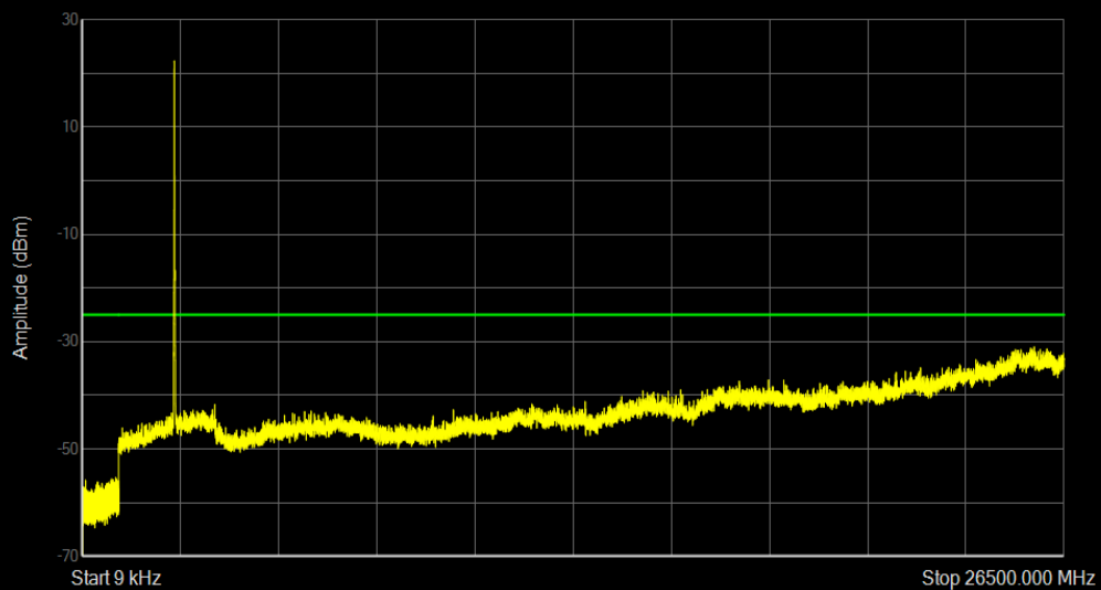
Band7 QPSK BW=5MHz Channel=20775 RB Size=25 Position=#0
