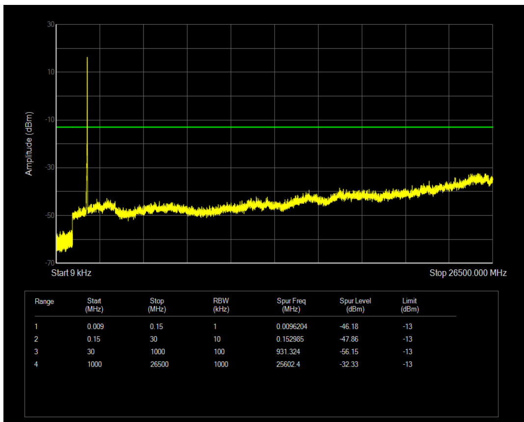
Band41(2555-2655) QAM16 BW=10MHz Channel=40290 RB Size=1 Position=#0
