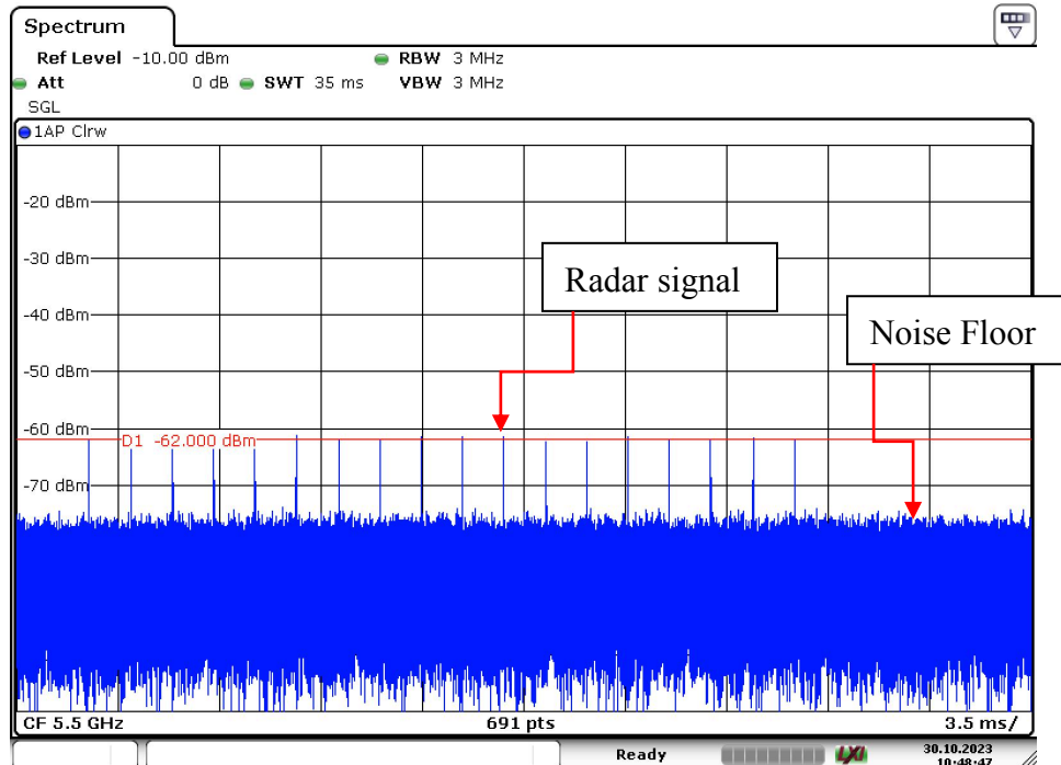
Radar Type 0 – 5500MHz
