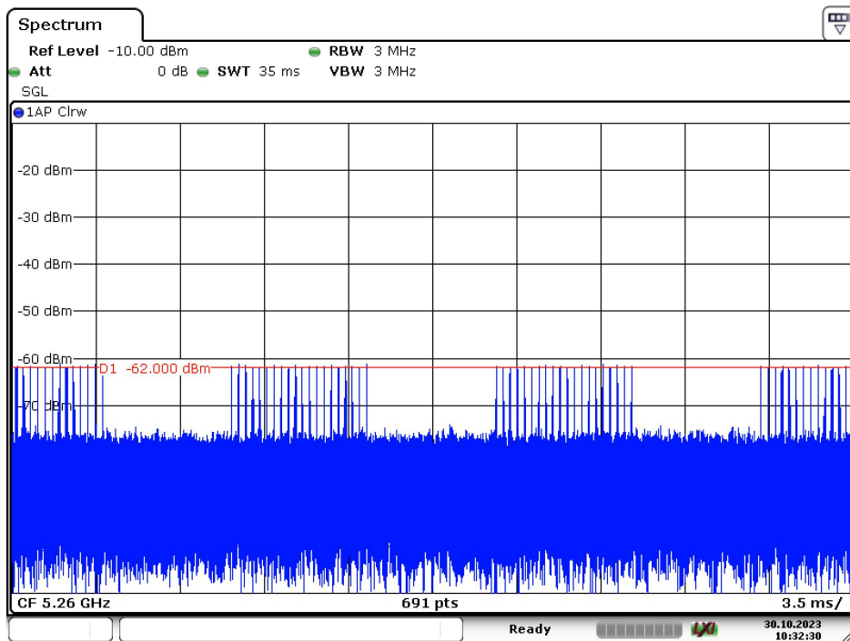
Radar Type 4 – 5260MHz
