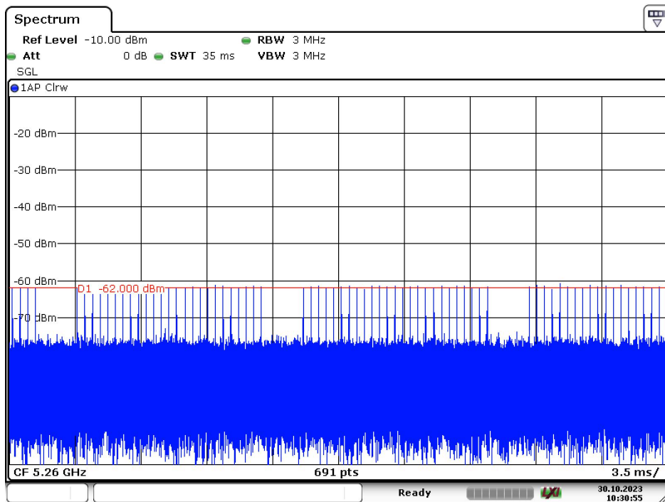
Radar Type 3 – 5260MHz
