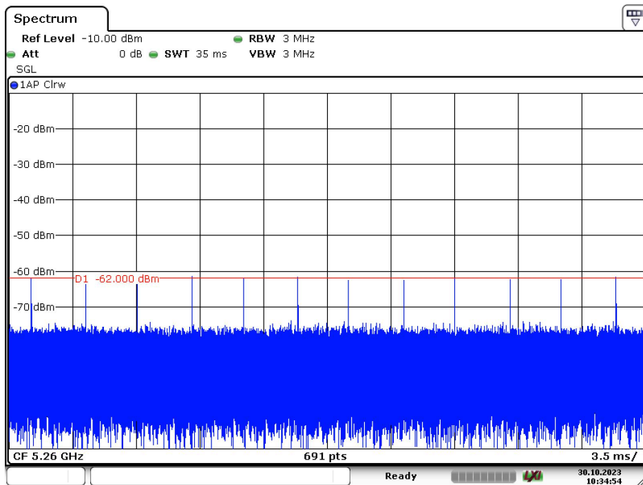
Radar Type 5 – 5260MHz
