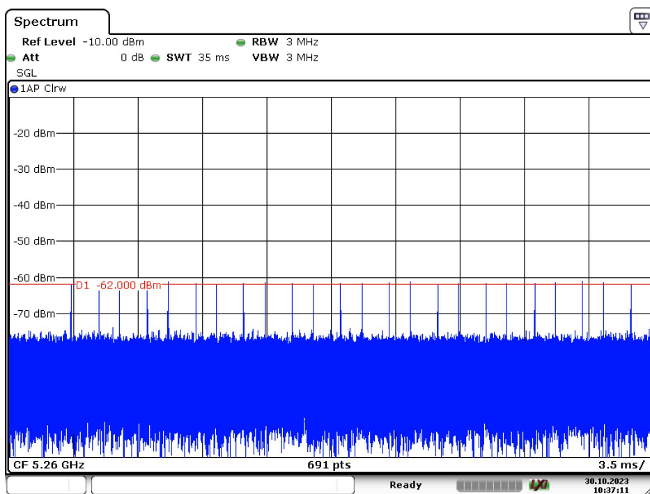
Radar Type 6 – 5260MHz
