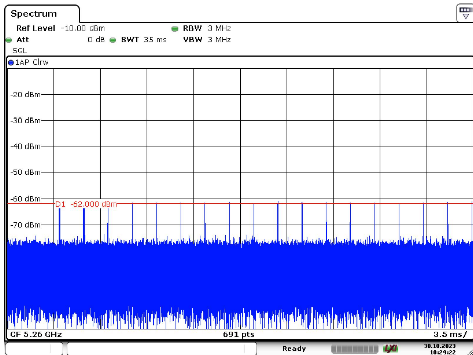
Radar Type 2 – 5260MHz
