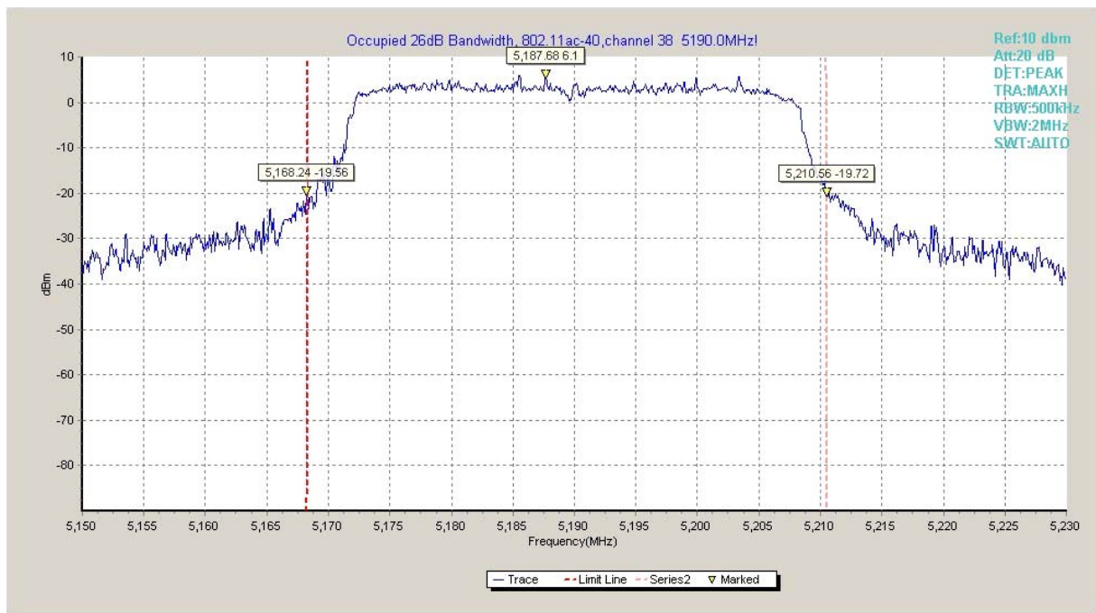
Fig.39 Occupied 26dB Bandwidth (802.11ac-HT40, 5190MHz)
