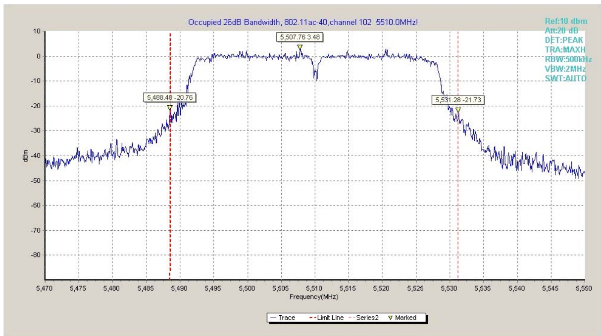
Fig.43 Occupied 26dB Bandwidth (802.11ac-HT40, 5510MHz)
