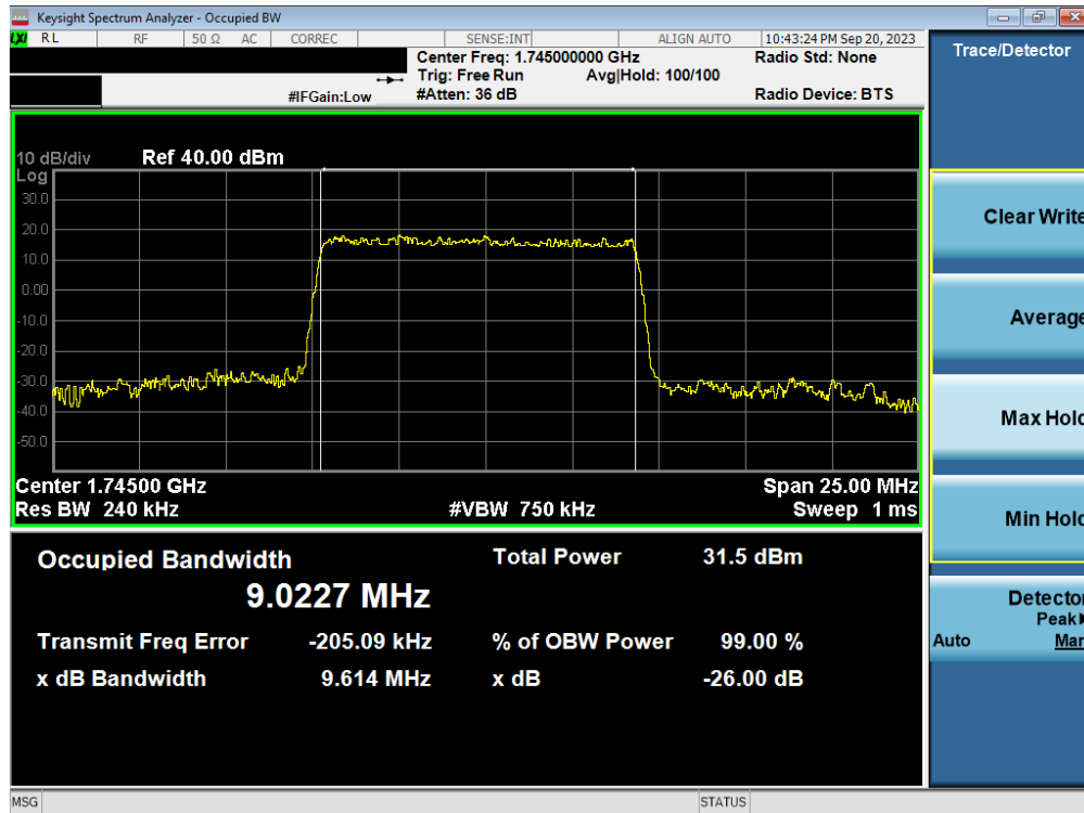
Plot 7-61. Occupied Bandwidth Plot (NR Band n66 - 10.0MHz DFT-s-OFDM BPSK - Full RB – ANT1)
