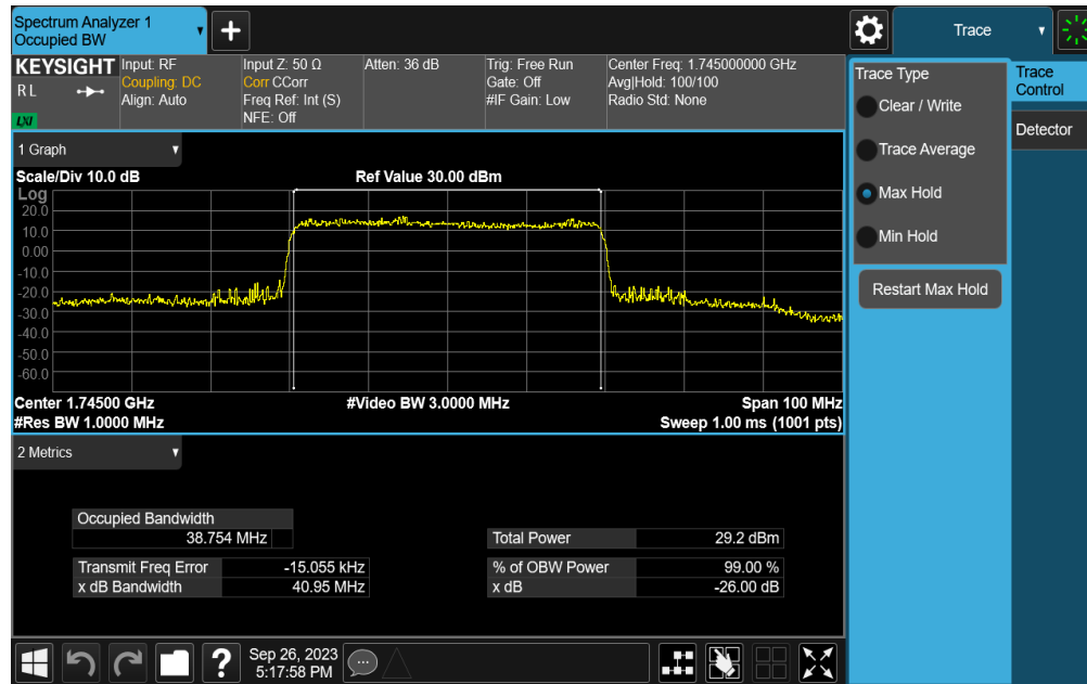
Plot 7-90. Occupied Bandwidth Plot (NR Band n66 - 40.0MHz CP-OFDM 16QAM - Full RB – ANT2)
