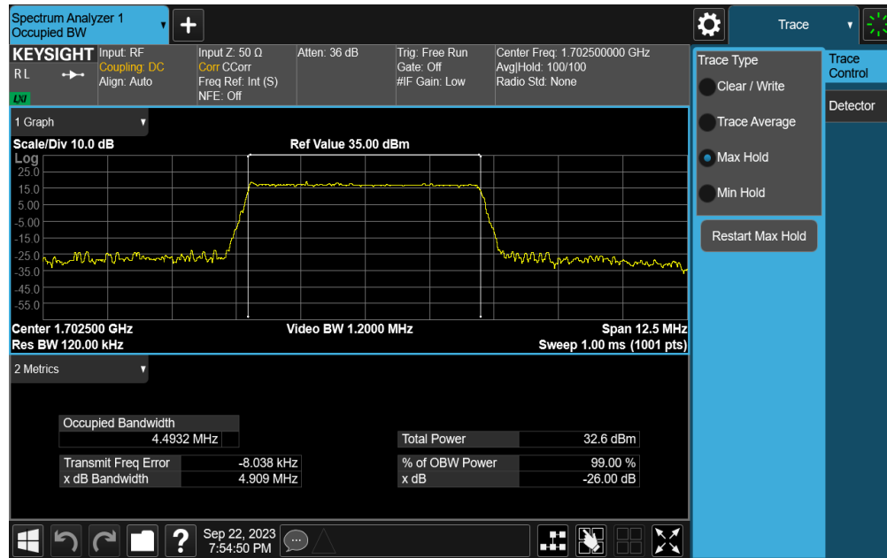
Plot 7-73. Occupied Bandwidth Plot (NR Band n70 - 5.0MHz DFT-s-OFDM BPSK - Full RB – ANT1)
