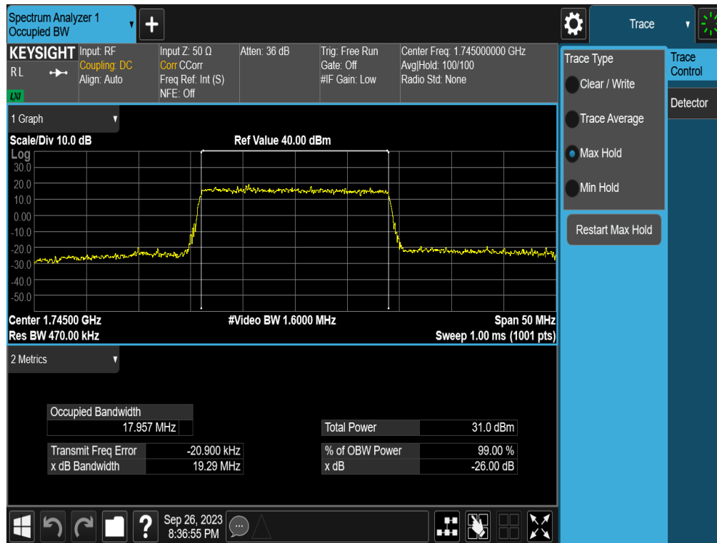
Plot 7-76. Occupied Bandwidth Plot (LTE Band 66/4 - 20MHz QPSK - Full RB - ANT2)
