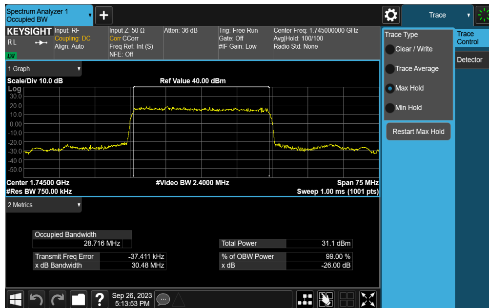
Plot 7-91. Occupied Bandwidth Plot (NR Band n66 - 30.0MHz DFT-s-OFDM BPSK - Full RB – ANT2)
