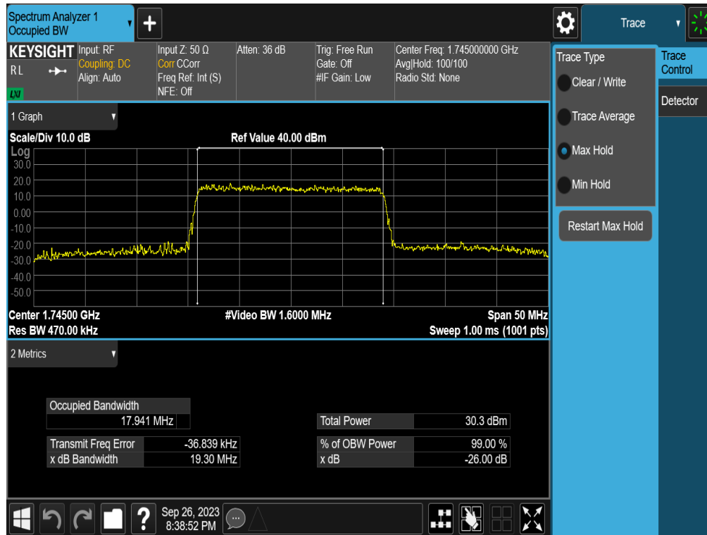
Plot 7-77. Occupied Bandwidth Plot (LTE Band 66/4 - 20MHz 16-QAM - Full RB - ANT2)
