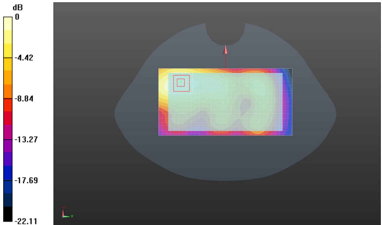
Body- worn Rear Side (LTE Band V Middle Channel)
