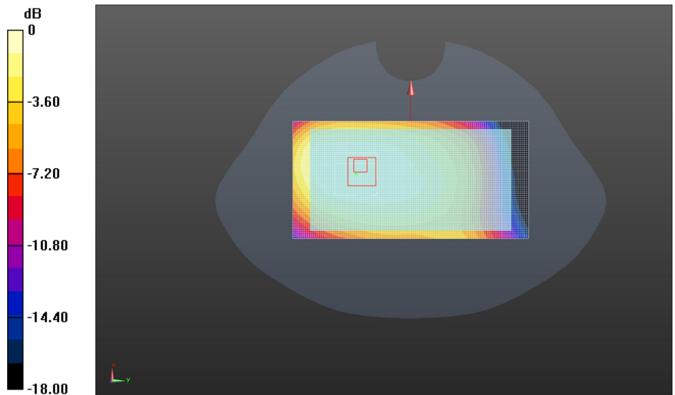
Body- worn Rear Side (LTE Band VII Middle Channel)
