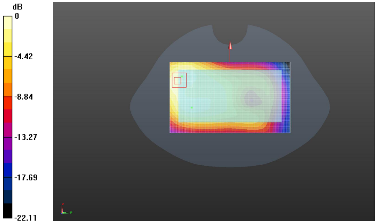
Body- worn Rear Side (LTE Band II Middle Channel)
