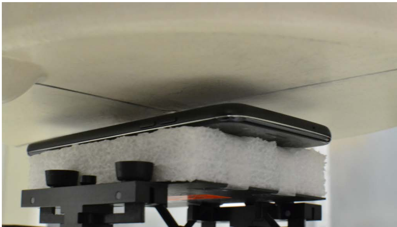
SAR Test Setup Photo 5 – Back Side at 10mm
