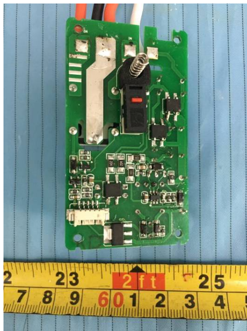
EUT – Main Board Top 2 View
