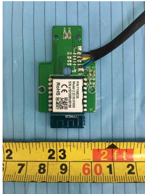
EUT – Main Board Top 1 View
