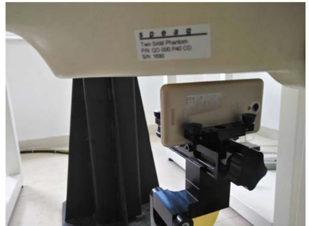
Hotspot mode - Right Side (10mm)
