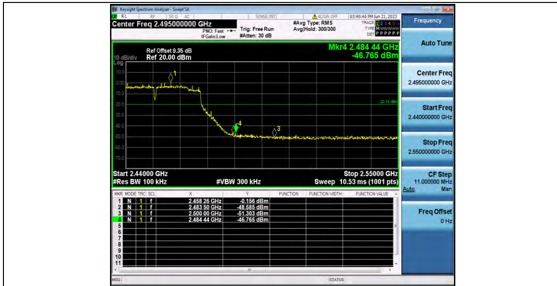
11N40SISO_Ant2_High_2452
