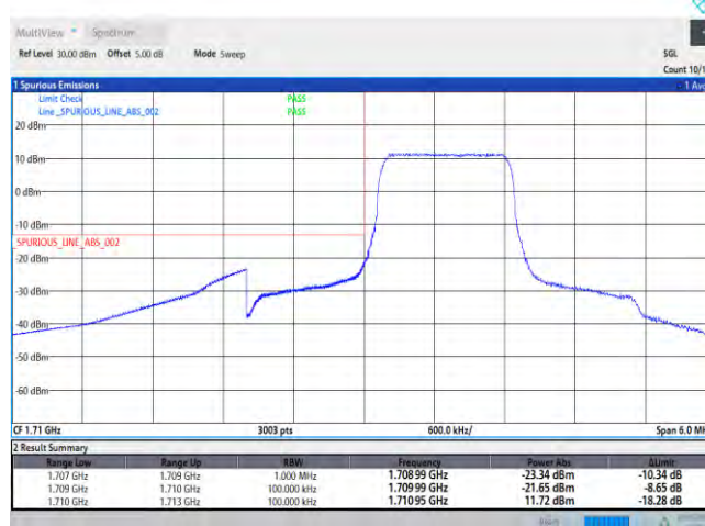
Band66-1.4MHz-QPSK-131979-6RB#0
