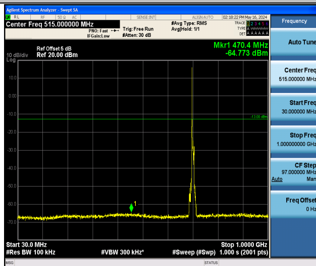
Band17_10MHz_16QAM_23780_1RB#0_30~1000_30~1000
