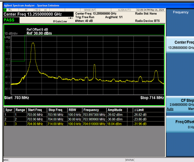
Band17_10MHz_16QAM_23780_1RB#0
