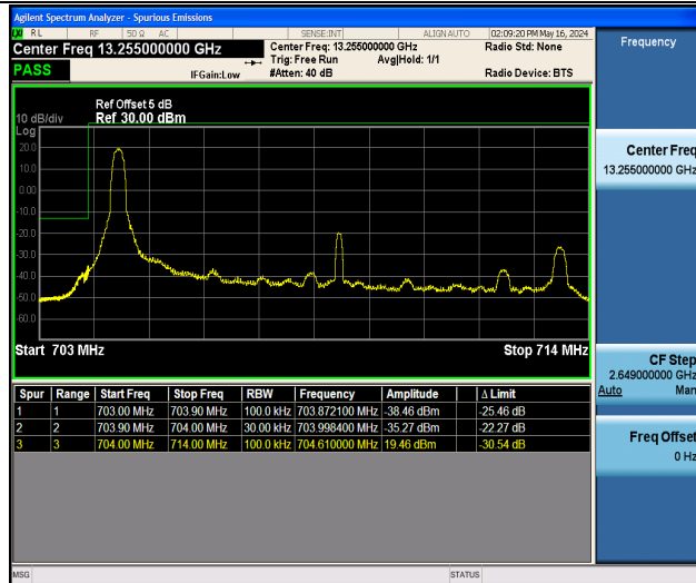
Band17_10MHz_QPSK_23780_1RB#0
