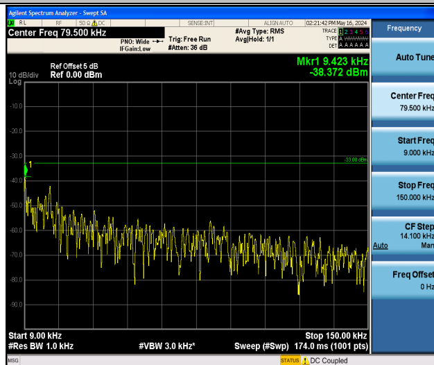
Band17_10MHz_16QAM_23800_1RB#0_0.009~0.15_0.009~0.15
