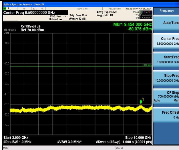
Band17_10MHz_QPSK_23800_1RB#0_3000~10000_3000~10000
