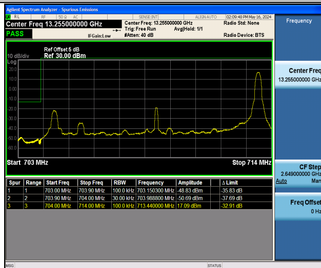
Band17_10MHz_QPSK_23780_1RB#49
