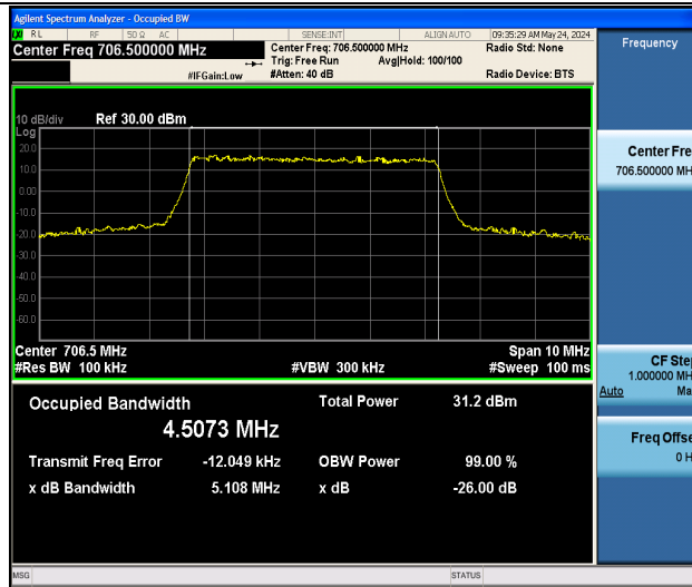
Band17-5MHz-QPSK-23755-25RB#0-PASS
