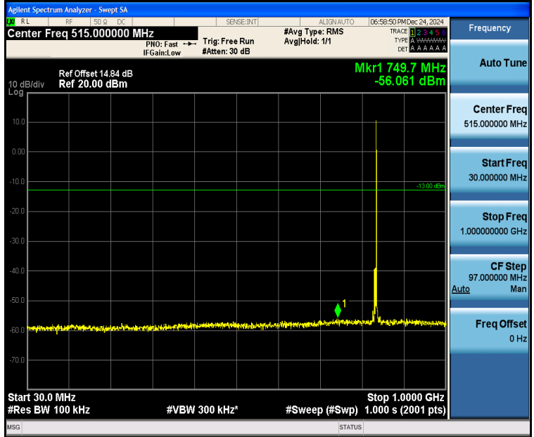
Band5_5MHz_16QAM_20525_1RB#24_30~1000_30~1000
