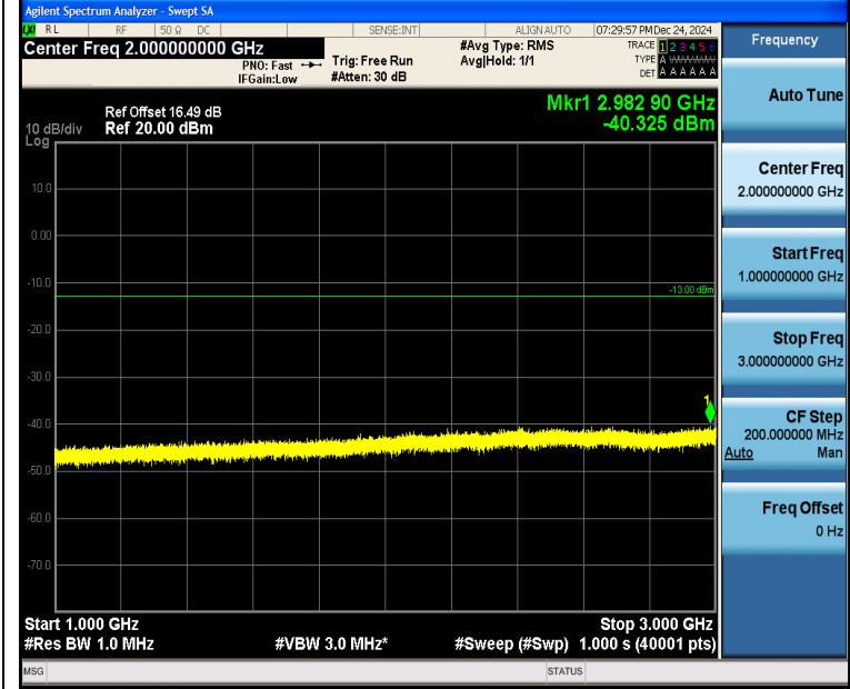
Band5_10MHz_16QAM_20525_1RB#0_1000~3000_1000~3000
