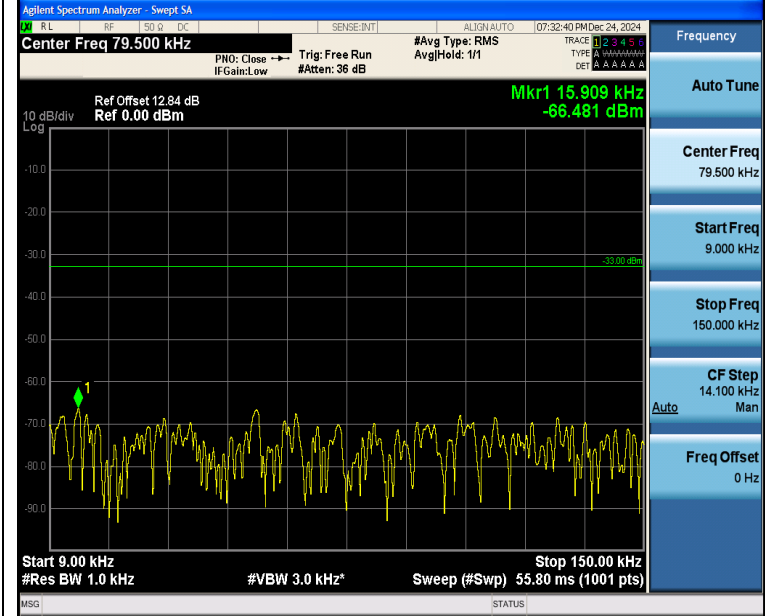
Band5_10MHz_QPSK_20600_1RB#0_0.009~0.15_0.009~0.15
