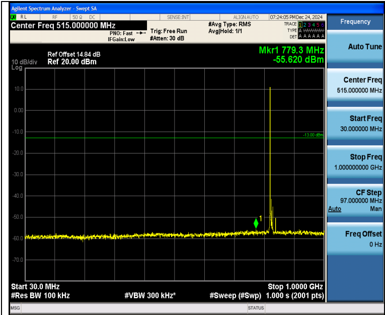
Band5_10MHz_QPSK_20450_1RB#0_30~1000_30~1000
