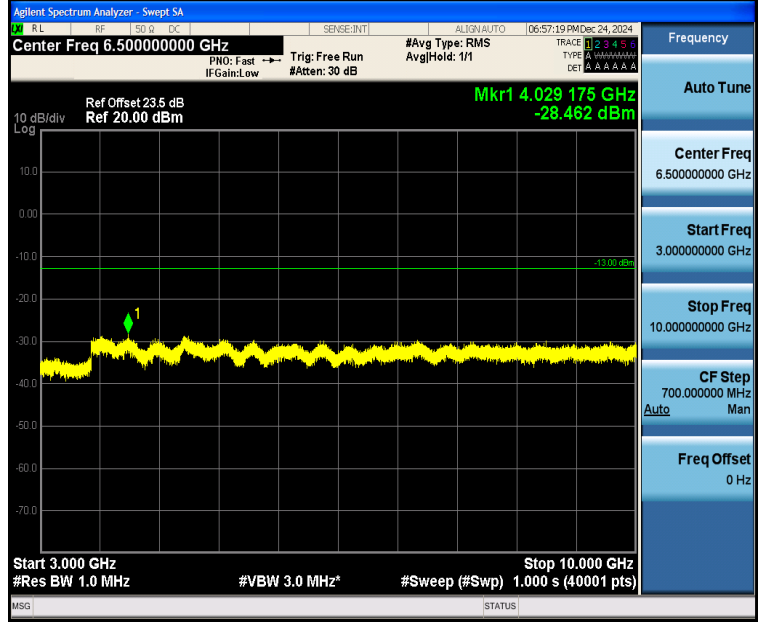
Band5_5MHz_16QAM_20525_1RB#0_3000~10000_3000~10000
