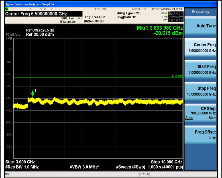
Band5_5MHz_16QAM_20425_25RB#0_3000~10000_3000~10000
