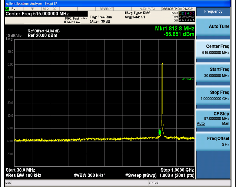
Band5_5MHz_16QAM_20425_25RB#0_30~1000_30~1000
