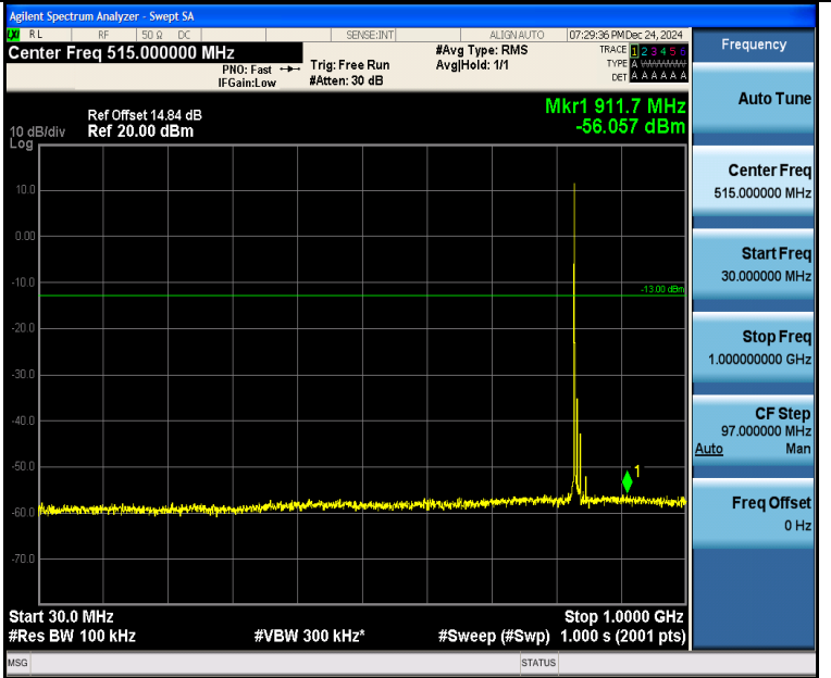
Band5_10MHz_16QAM_20525_1RB#0_30~1000_30~1000
