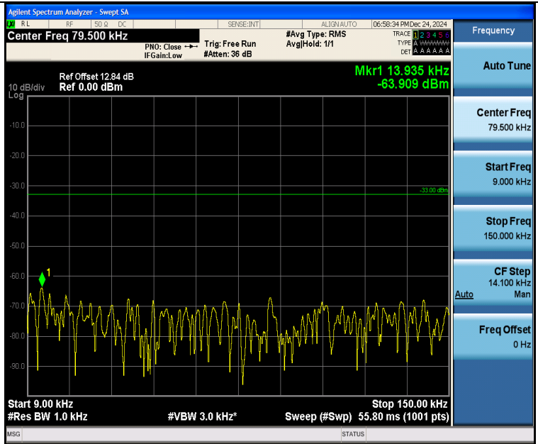
Band5_5MHz_16QAM_20525_1RB#24_0.009~0.15_0.009~0.15
