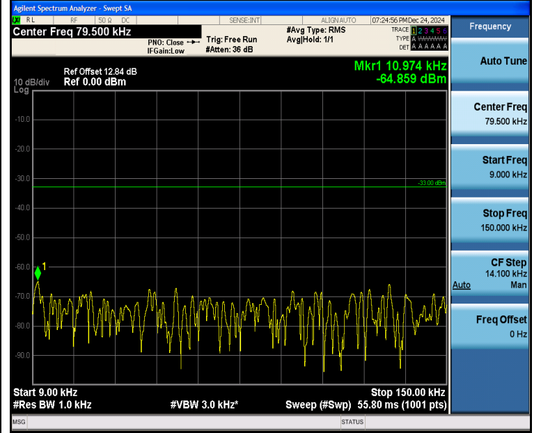
Band5_10MHz_16QAM_20450_1RB#0_0.009~0.15_0.009~0.15
