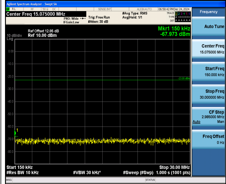
Band5_5MHz_16QAM_20525_1RB#24_0.15~30_0.15~30
