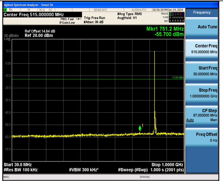
Band5_5MHz_16QAM_20525_1RB#0_30~1000_30~1000
