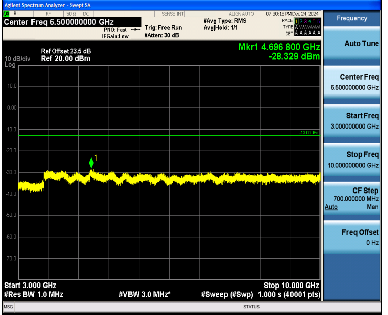
Band5_10MHz_16QAM_20525_1RB#0_3000~10000_3000~10000
