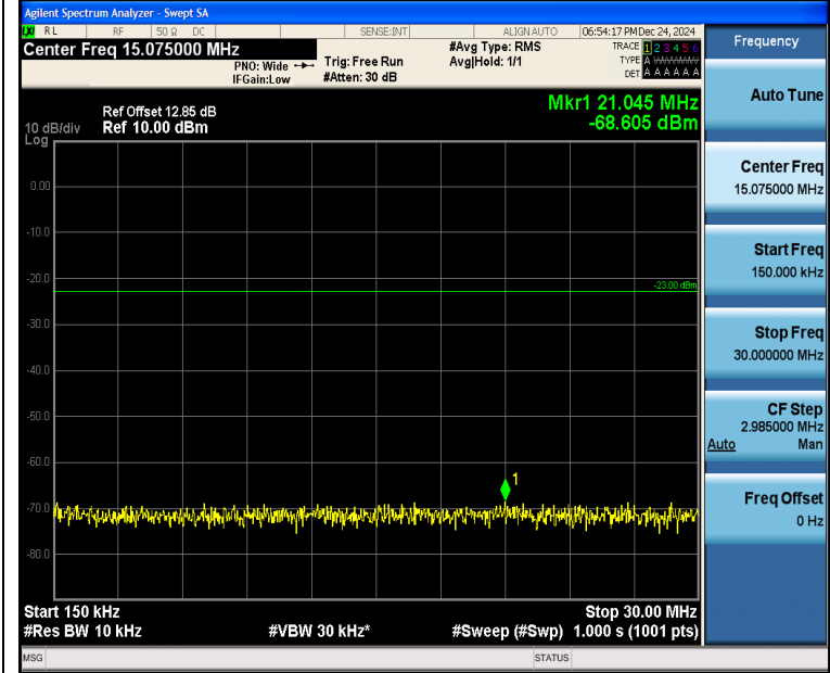
Band5_5MHz_16QAM_20425_25RB#0_0.15~30_0.15~30
