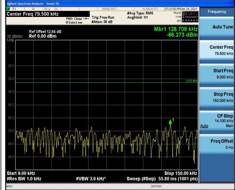
Band5_10MHz_QPSK_20450_1RB#0_0.009~0.15_0.009~0.15
