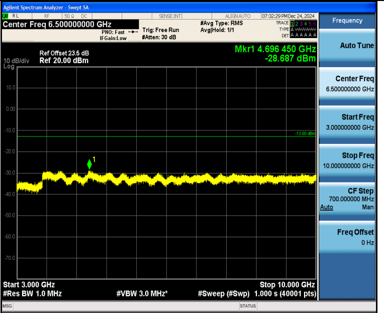
Band5_10MHz_16QAM_20525_1RB#49_3000~10000_3000~10000
