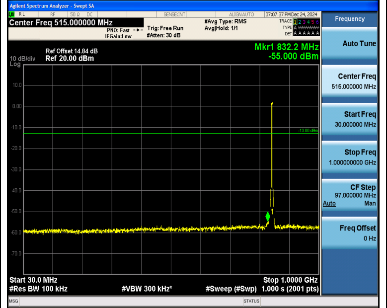
Band5_5MHz_16QAM_20625_25RB#0_30~1000_30~1000
