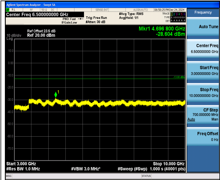
Band5_5MHz_QPSK_20525_1RB#24_3000~10000_3000~10000
