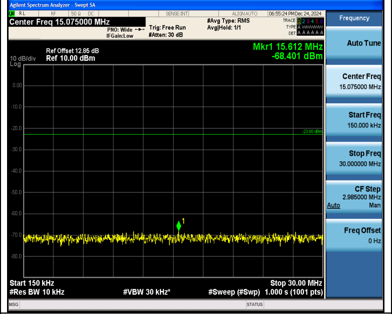
Band5_5MHz_QPSK_20525_1RB#0_0.15~30_0.15~30
