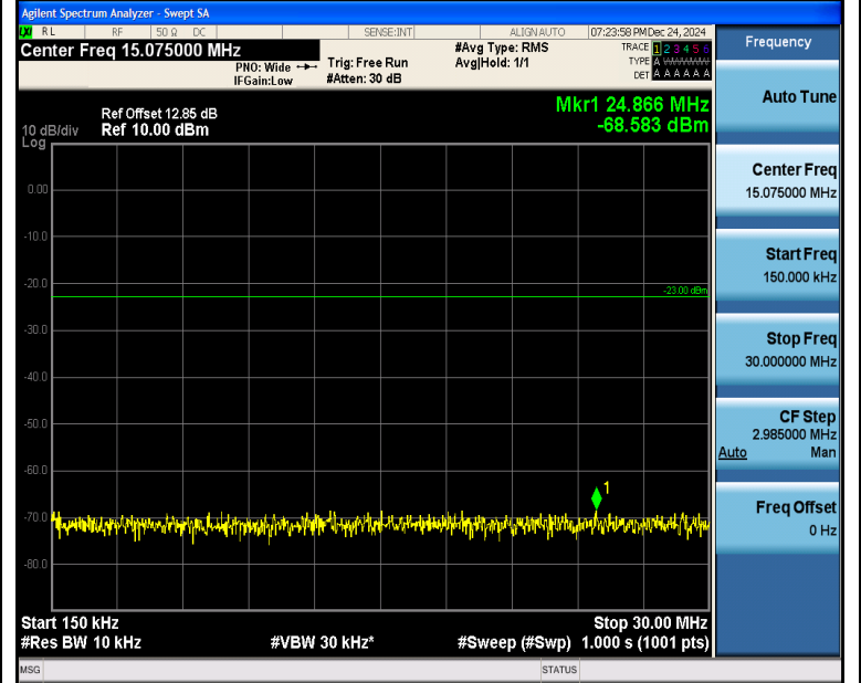
Band5_10MHz_QPSK_20450_1RB#0_0.15~30_0.15~30
