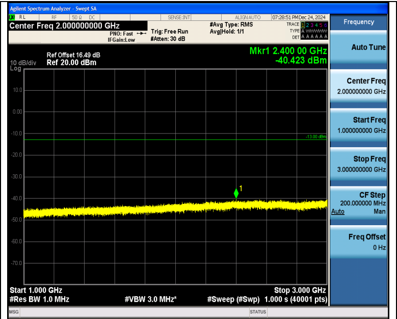
Band5_10MHz_QPSK_20525_1RB#0_1000~3000_1000~3000
