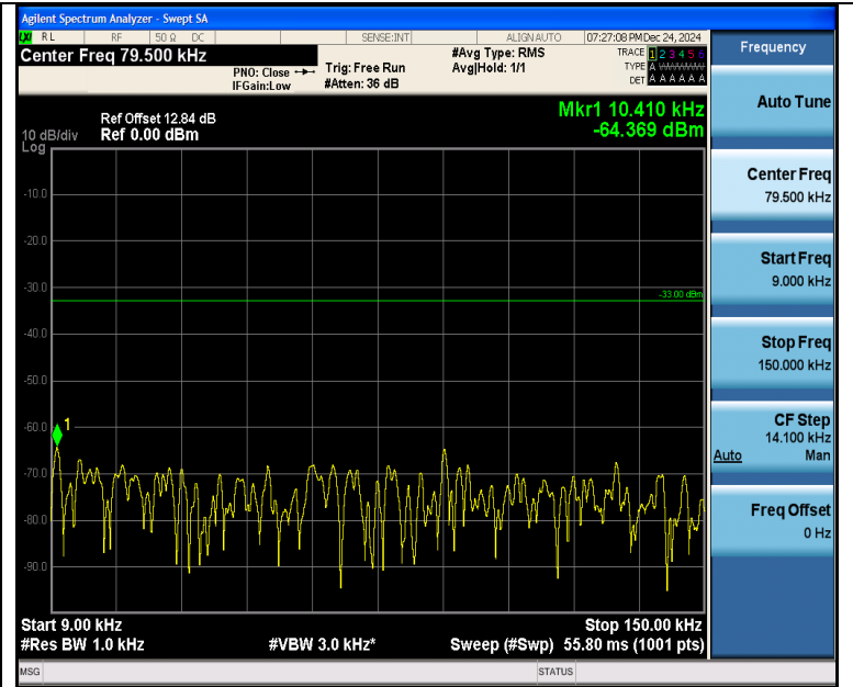
Band5_10MHz_16QAM_20450_1RB#49_0.009~0.15_0.009~0.15
