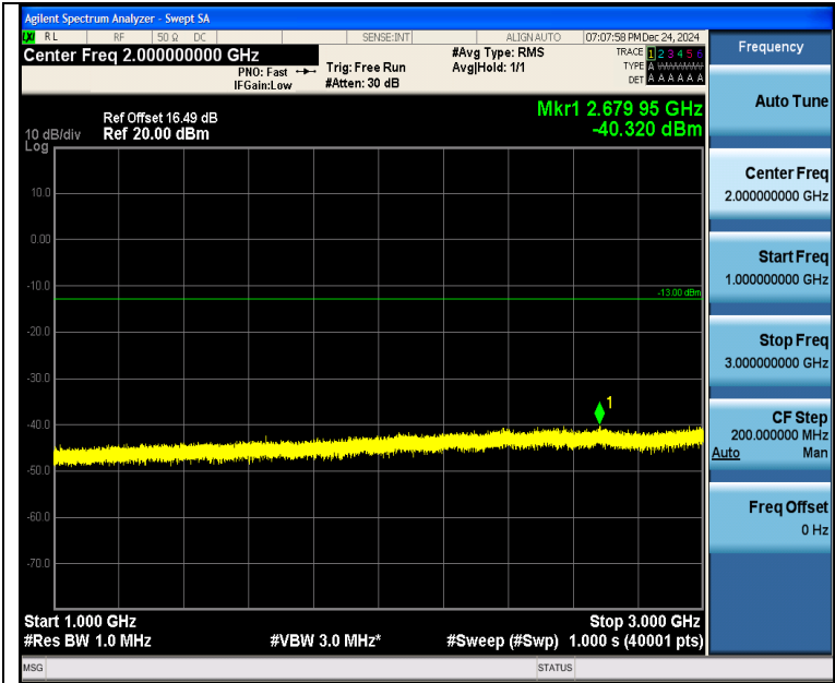
Band5_5MHz_16QAM_20625_25RB#0_1000~3000_1000~3000
