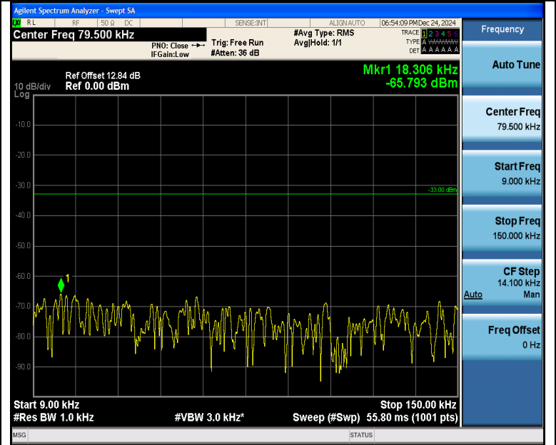
Band5_5MHz_16QAM_20425_25RB#0_0.009~0.15_0.009~0.15
