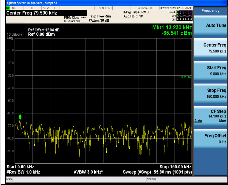
Band5_5MHz_QPSK_20525_1RB#0_0.009~0.15_0.009~0.15
