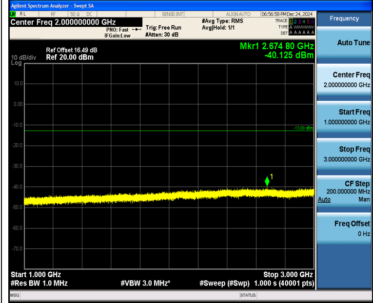
Band5_5MHz_16QAM_20525_1RB#0_1000~3000_1000~3000
