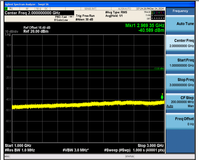
Band5_10MHz_QPSK_20450_1RB#0_1000~3000_1000~3000
