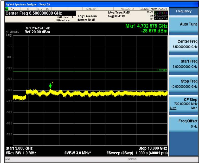
Band5_10MHz_QPSK_20450_1RB#49_3000~10000_3000~10000
