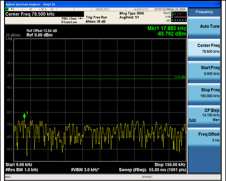
Band5_5MHz_16QAM_20625_25RB#0_0.009~0.15_0.009~0.15
