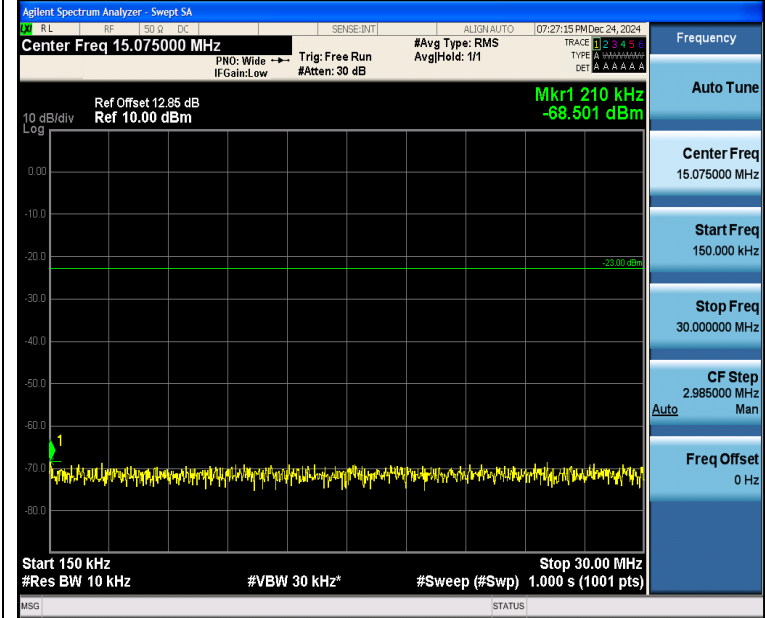
Band5_10MHz_16QAM_20450_1RB#49_0.15~30_0.15~30
