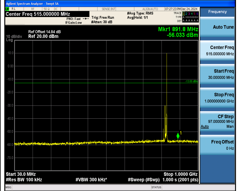
Band5_10MHz_16QAM_20450_1RB#49_30~1000_30~1000
