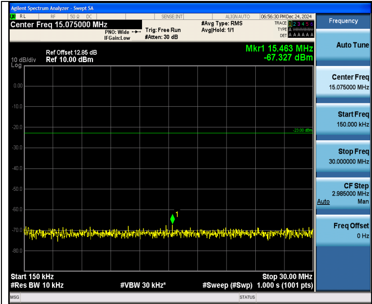
Band5_5MHz_16QAM_20525_1RB#0_0.15~30_0.15~30
