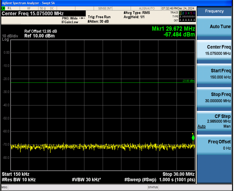
Band5_10MHz_QPSK_20600_1RB#0_0.15~30_0.15~30
