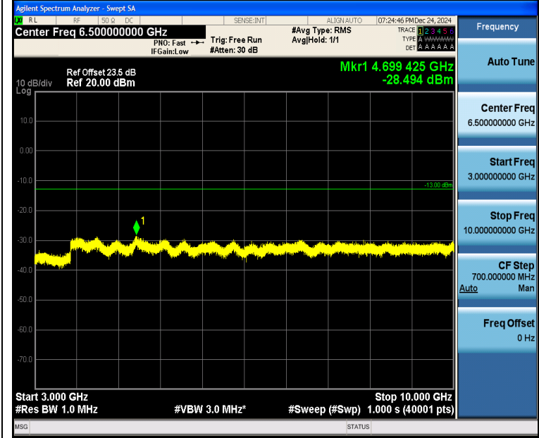
Band5_10MHz_QPSK_20450_1RB#0_3000~10000_3000~10000
