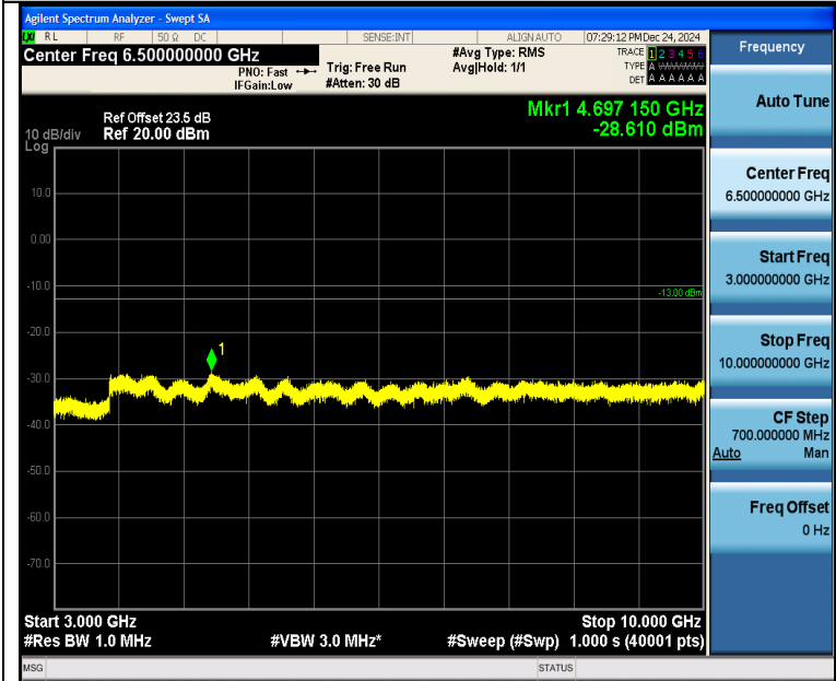
Band5_10MHz_QPSK_20525_1RB#0_3000~10000_3000~10000
