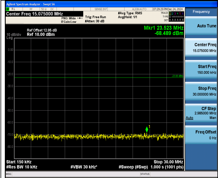
Band5_10MHz_16QAM_20525_1RB#0_0.15~30_0.15~30
