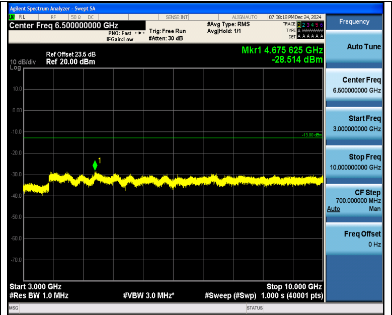
Band5_5MHz_16QAM_20625_25RB#0_3000~10000_3000~10000
