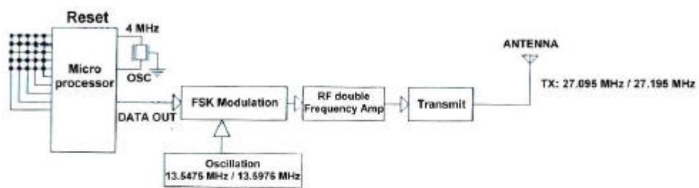
Transmitter (Keyboard) Block Diagram
