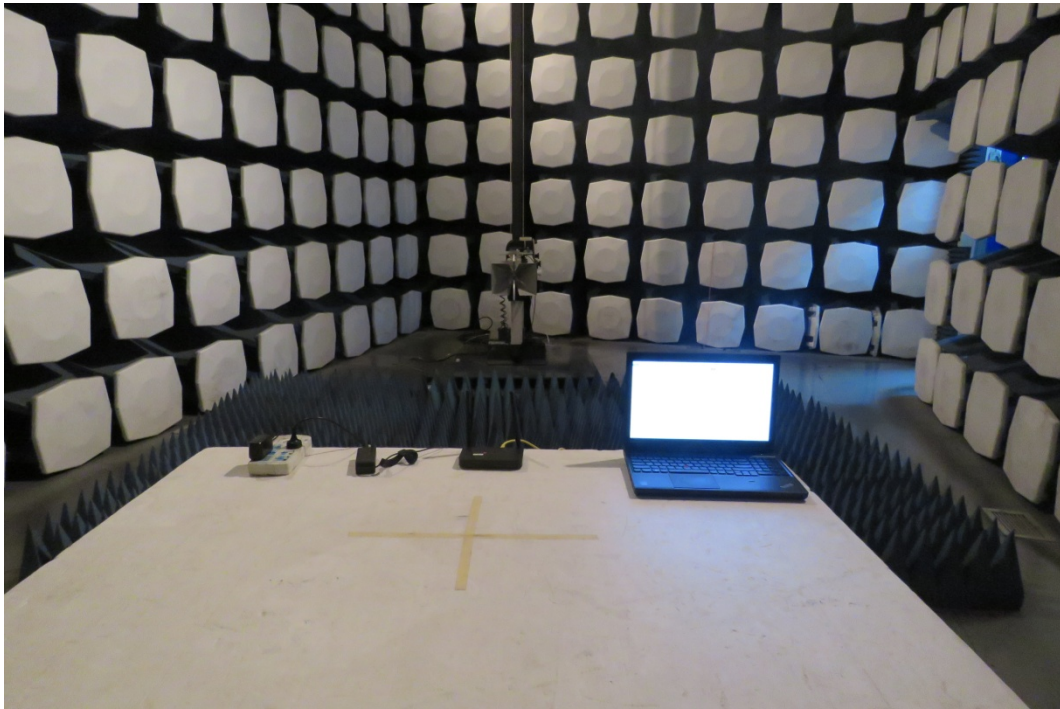
b: Above 1GHz Radiated Emission Test Setup
