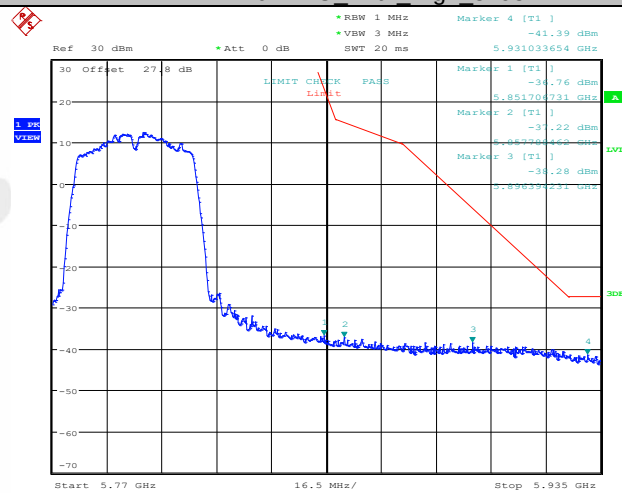
11N40MIMO Ant1 High 5795
