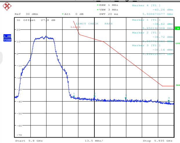
11N20MIMO Ant2 High 5825
