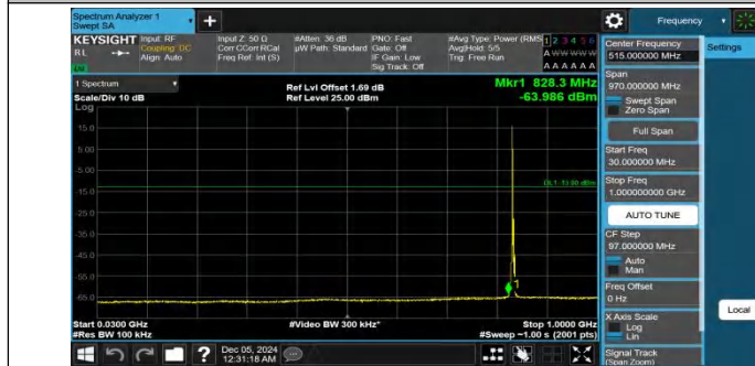
Band26(824-849)-3MHz-QPSK-26915-1RB#0-30~1000-PASS
