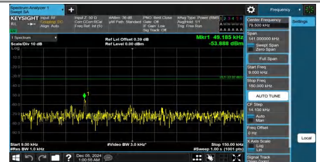
Band26(824-849)-15MHz-QPSK-26865-1RB#74-0.009~0.15-PASS
