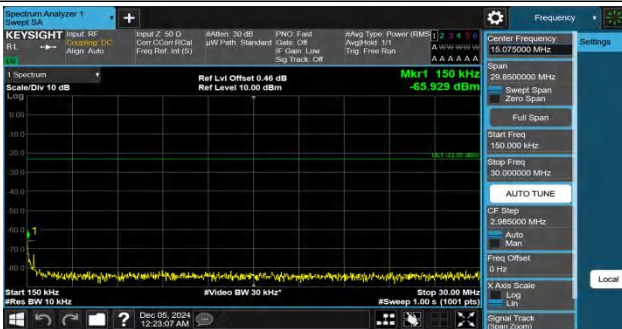
Band26(824-849)-1.4MHz-QPSK-27033-1RB#5-0.15~30-PASS
