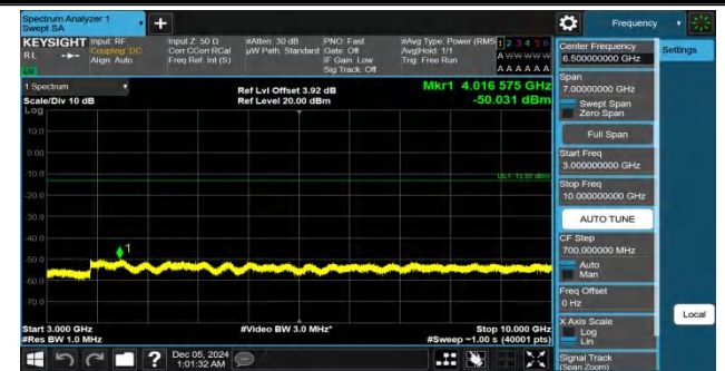
Band26(824-849)-15MHz-QPSK-26865-1RB#74-3000~10000-PAS
