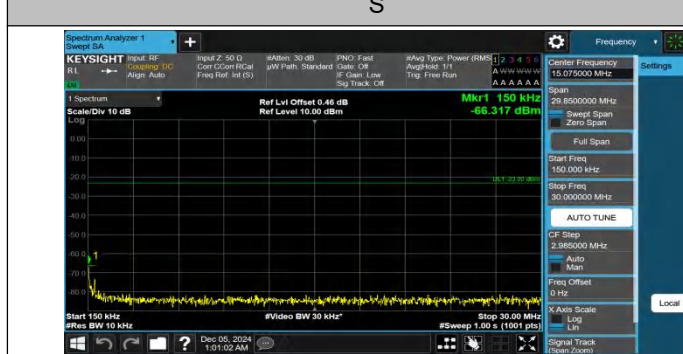
Band26(824-849)-15MHz-QPSK-26865-1RB#74-0.15~30-PASS
