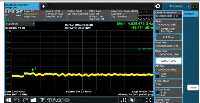
Band26(824-849)-10MHz-QPSK-26915-1RB#49-3000~10000-PAS
