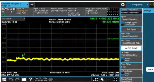
Band26(824-849)-1.4MHz-QPSK-27033-1RB#0-3000~10000-PAS S
