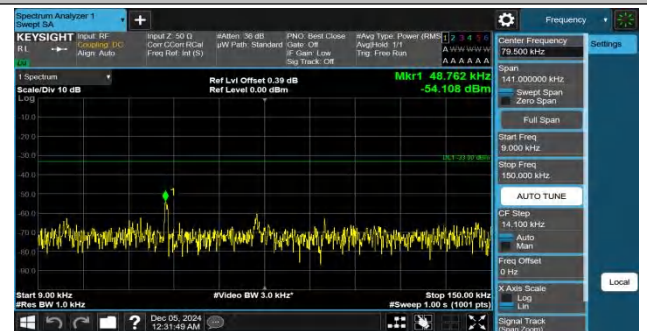
Band26(824-849)-3MHz-QPSK-26915-1RB#14-0.009~0.15-PASS
