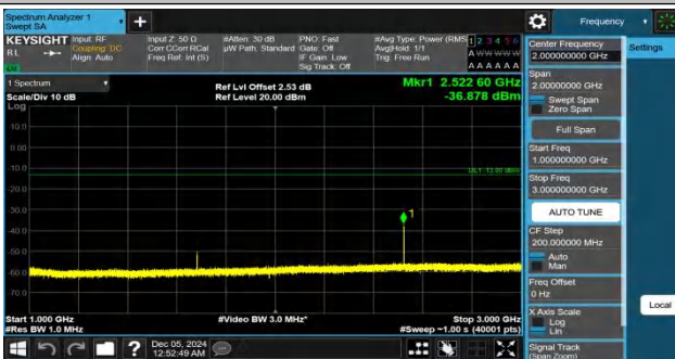
Band26(824-849)-10MHz-QPSK-26915-1RB#49-1000~3000-PAS
