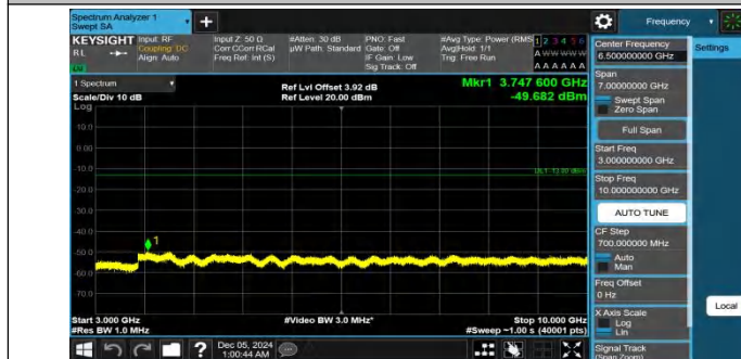
Band26(824-849)-15MHz-QPSK-26865-1RB#0-3000~10000-PASS
