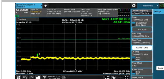
Band26(824-849)-15MHz-QPSK-26915-1RB#0-3000~10000-PAS
