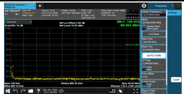
Band26(824-849)-3MHz-QPSK-26915-1RB#0-0.15~30-PASS
