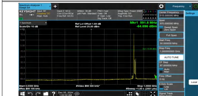
Band26(824-849)-15MHz-QPSK-26915-1RB#0-30~1000-PASS
