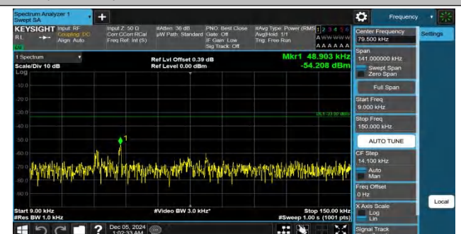
Band26(824-849)-15MHz-QPSK-26915-1RB#74-0.009~0.15-PASS
