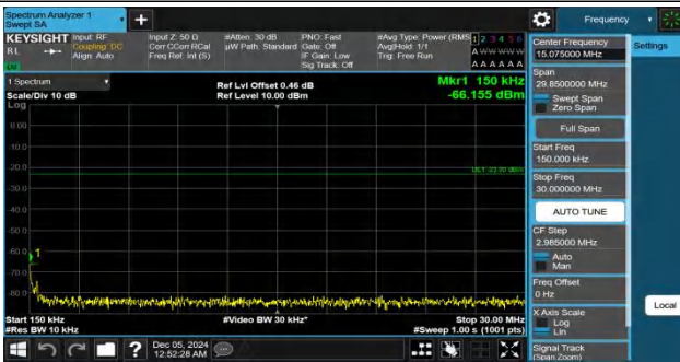
Band26(824-849)-10MHz-QPSK-26915-1RB#49-0.15~30-PASS
