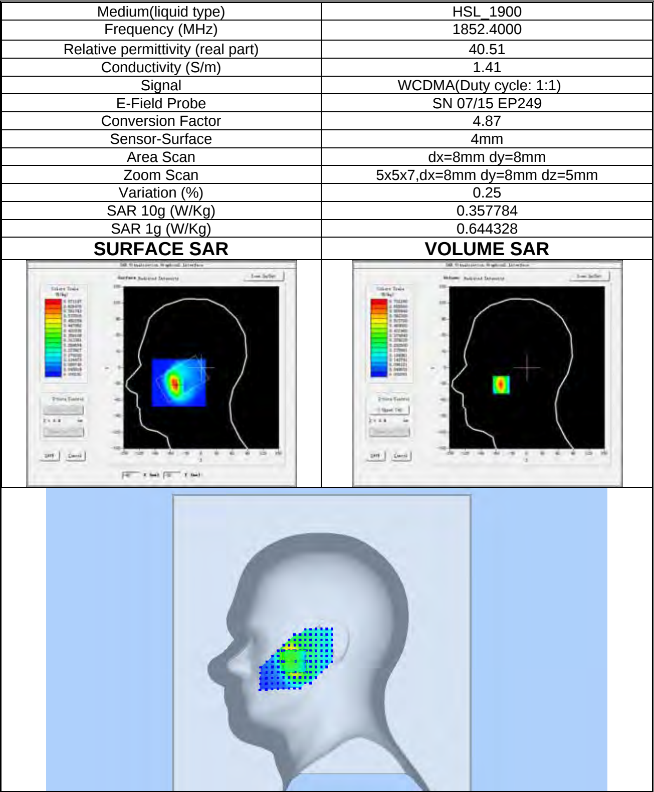
Plot 10: WCDMA BAND , Low channel (Right Head Cheek) Product Description: SMARTPHONE Test Date: 2018-07-10
