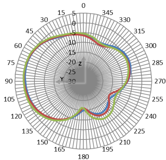
Ant1_2G4 Elevation YZ
