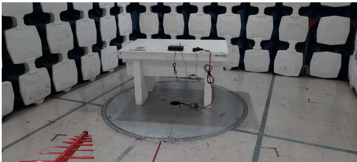
30MHz-1GHz Front
