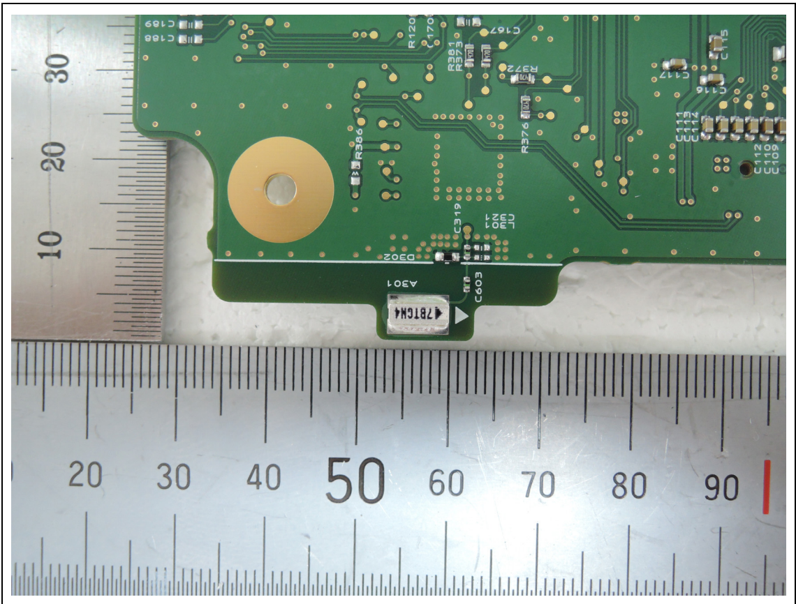
<BT Antenna>
