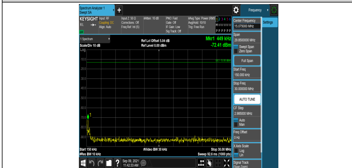
Band4-3MHz-16QAM-20385-1RB#0-Range2:0.15~30MHz
