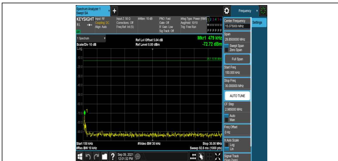
Band4-5MHz-16QAM-19975-1RB#0-Range2:0.15~30MHz
