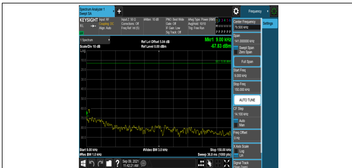
Band4-3MHz-16QAM-20385-1RB#0-Range1:0.009~0.15MHz
