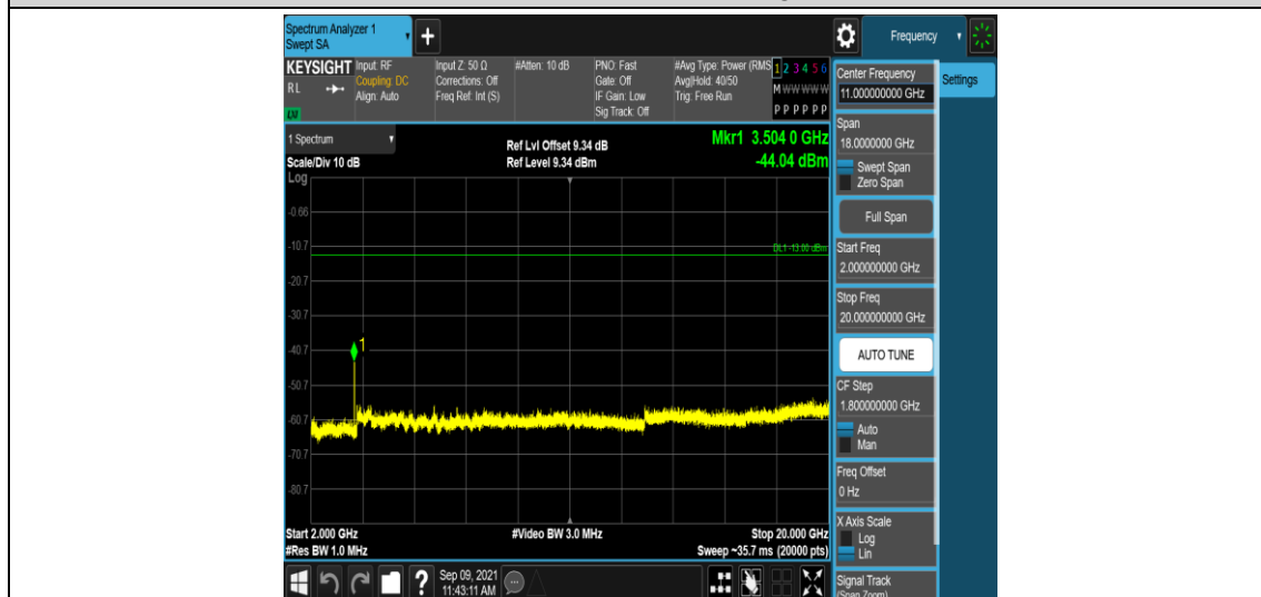
Band4-3MHz-16QAM-20385-1RB#0-Range5:2000~20000MHz
