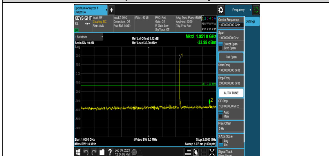
Band4-5MHz-16QAM-20175-1RB#0-Range4:1000~2000MHz
