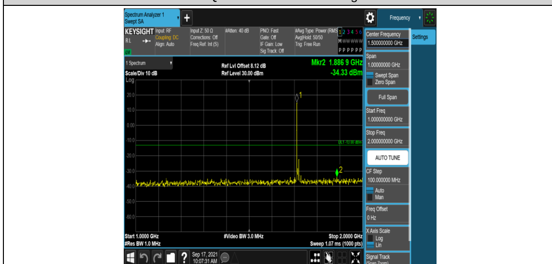
Band4-10MHz-16QAM-20000-1RB#0-Range4:1000~2000MHz
