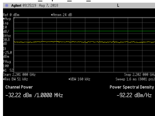
Dual LTE5_Top Ch_UBE_2201 to 2202MHz
