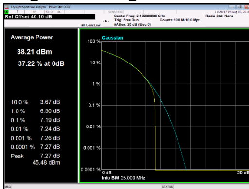
LTE5_Middle Channel_CCDF
