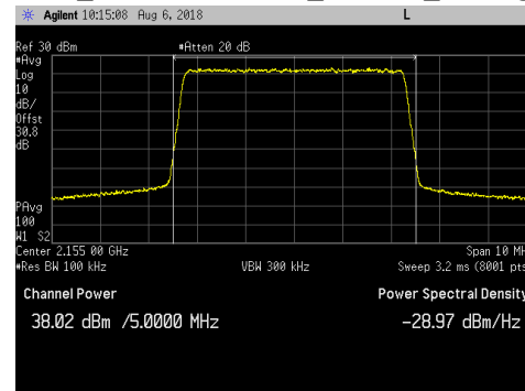
LTE5_Middle Channel_64QAM_Average
