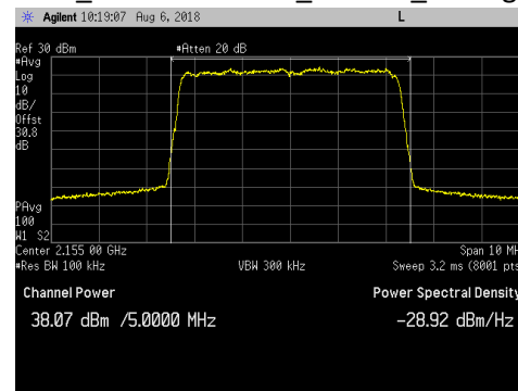
LTE5_Middle Channel_16QAM_Average
