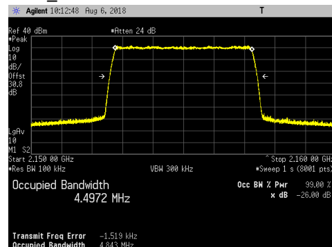
LTE5_64QAM
