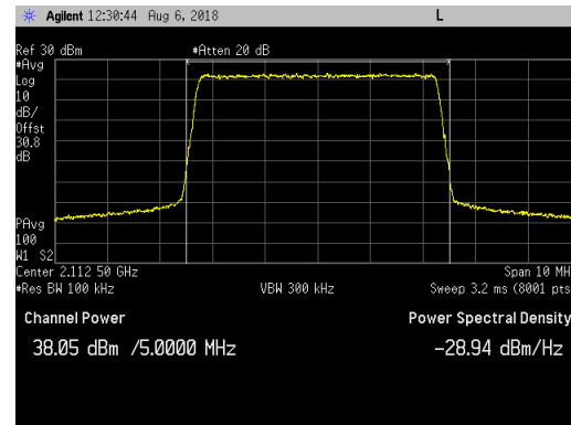
LTE5_Bottom Channel Average
