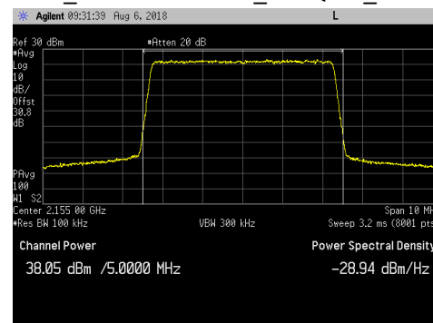
LTE5_Middle Channel_256QAM_Average
