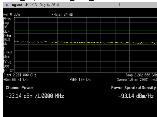
LTE5_Top Channel_UBE_2201 to 2202MHz
