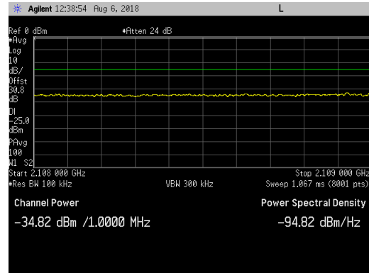
LTE10_Bottom Channel_LBE_2108 to 2109MHz
