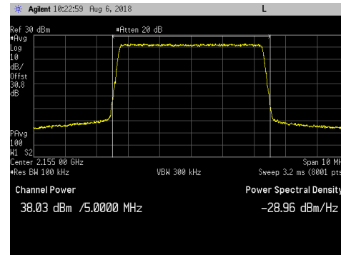
LTE5_Middle Channel_16QAM_Average
