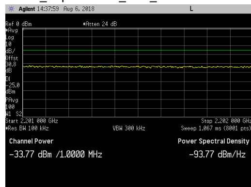
LTE10_Top Channel_UBE_2201 to 2202MHz
