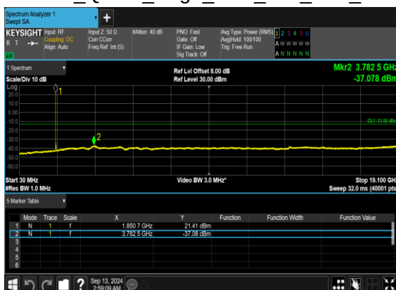
N2(20M)_DFT-s- OFDM_QPSK_Edge_1RB_Left_Low_CH
