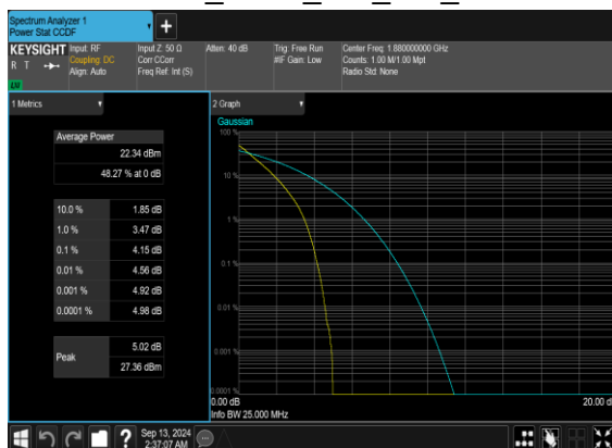
N2(20M)_DFT-s-OFDM_PI_2- BPSK_Outer_Full_Mid_CH
